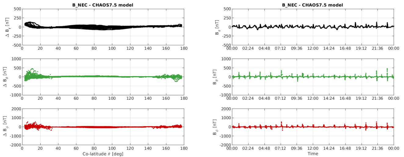
Figure 3-12: S/C C day 05/06: time series of B_{NEC} - B_{Chaos} residuals (right) and B_{NEC} - B_{Chaos} vs colatitude (left)
