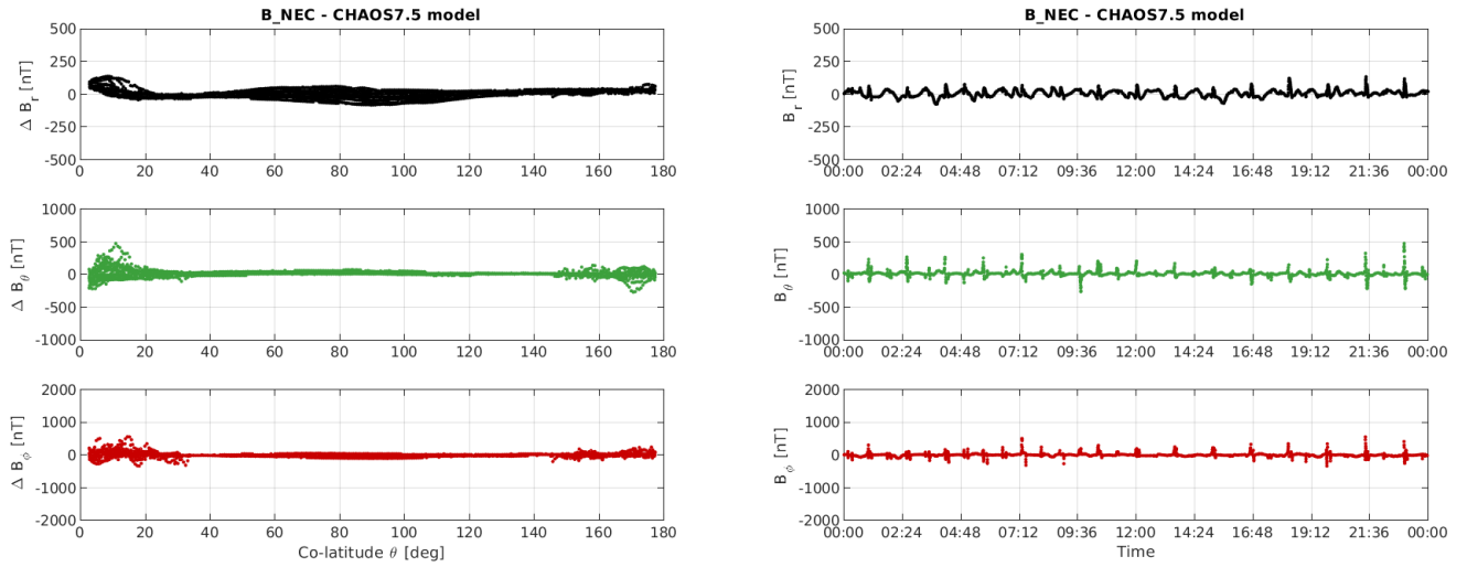
Figure 3-10: S/C A day 05/06: time series of B_{NEC} - B_{Chaos} residuals (right) and B_{NEC} - B_{Chaos} vs colatitude (left).
