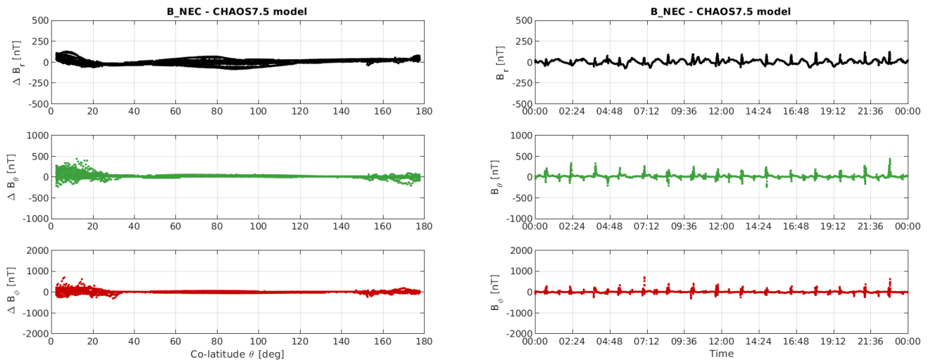
Figure 3-11: S/C B day 05/06: time series of B_{NEC} - B_{Chaos} residuals (right) and B_{NEC} - B_{Chaos} vs colatitude (left).
