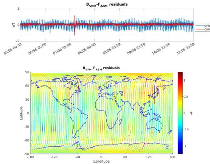
Figure 3-5: ASM-VFM residuals for S/C A, during monitoring period 05/06-11/06. In top figure are plotted: difference between |B_{VFM}| and F_{ASM} (without dB_{Sun} correction) (blue colour), and the residuals with dB_{Sun} corrections (red colour). In bottom figure residuals are presented on the world map.
