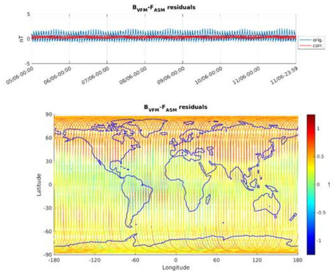
Figure 3-6: ASM-VFM residuals for S/C B, during monitoring period 05/06-11/06. In top figure are plotted: difference between |B_{VFM}| and F_{ASM} (without dB_{Sun} correction) (blue colour), and the residuals with dB_{Sun} corrections (red colour). In bottom figure residuals are presented on the world map.
