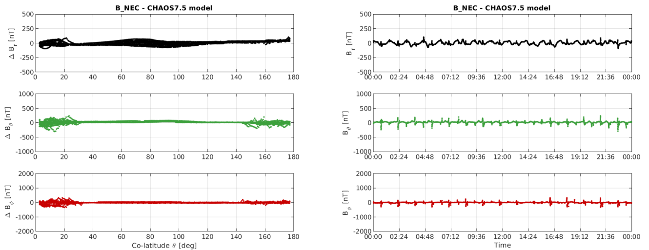
Figure 3-10: S/C A day 29/05: time series of B_{NEC} - B_{Chaos} residuals (right) and B_{NEC} - B_{Chaos} vs colatitude (left).
