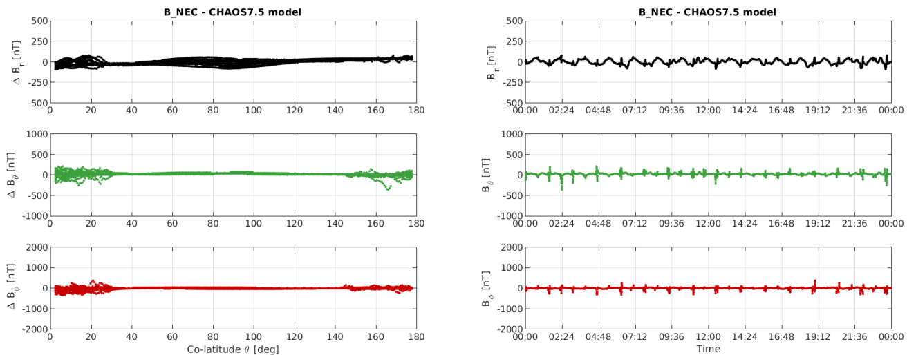
Figure 3-11: S/C B day 29/05: time series of B_{NEC} - B_{Chaos} residuals (right) and B_{NEC} - B_{Chaos} vs colatitude (left).
