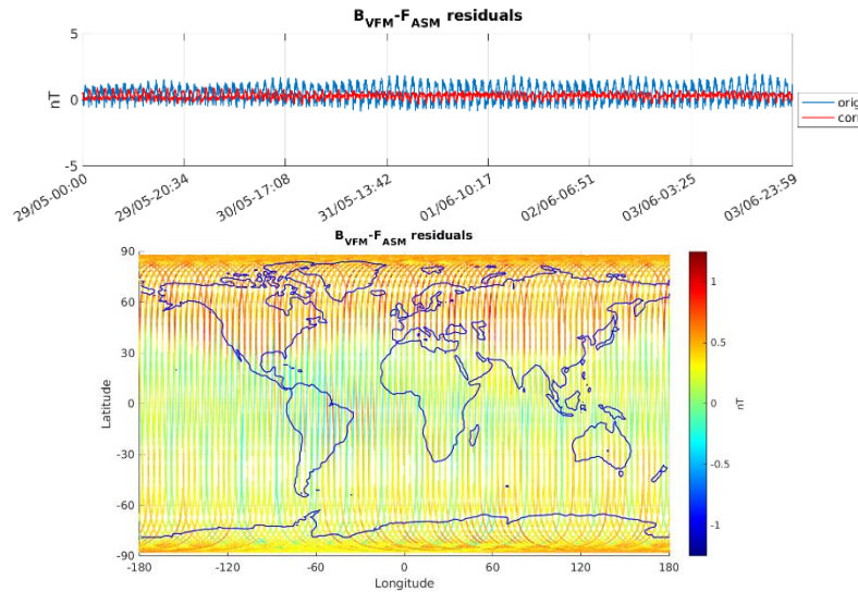
Figure 3-6: ASM-VFM residuals for S/C B, during monitoring period 29/05-04/06. In top figure are plotted: difference between |B_{VFM}| and F_{ASM} (without dB_{Sun} correction) (blue colour), and the residuals with dB_{Sun} corrections (red colour). In bottom figure residuals are presented on the world map.
