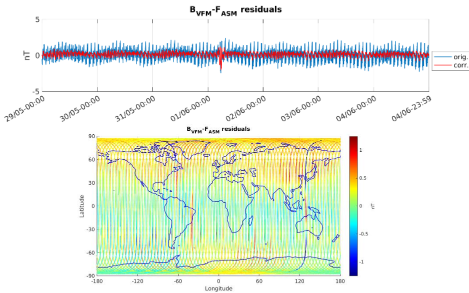
Figure 3-5: ASM-VFM residuals for S/C A, during monitoring period 29/05-04/06. In top figure are plotted: difference between |B_{VFM}| and F_{ASM} (without dB_{Sun} correction) (blue colour), and the residuals with dB_{Sun} corrections (red colour). In bottom figure residuals are presented on the world map.
