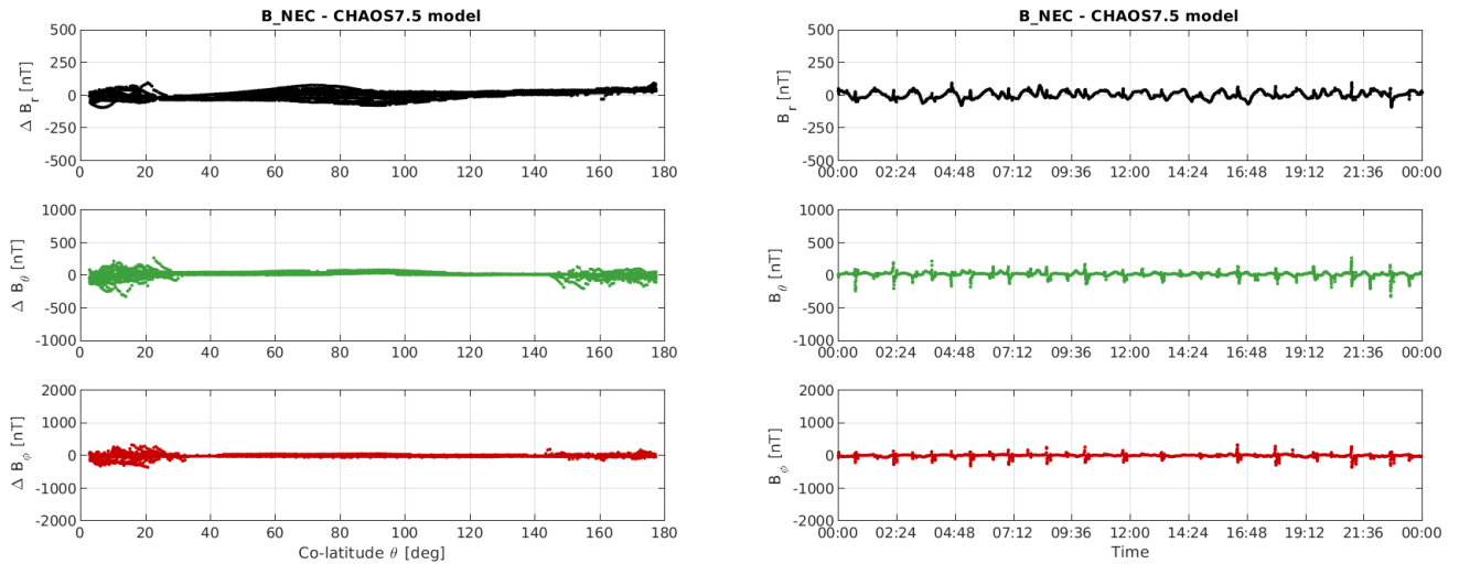
Figure 3-12: S/C C day 29/05: time series of B_{NEC} - B_{Chaos} residuals (right) and B_{NEC} - B_{Chaos} vs colatitude (left)
