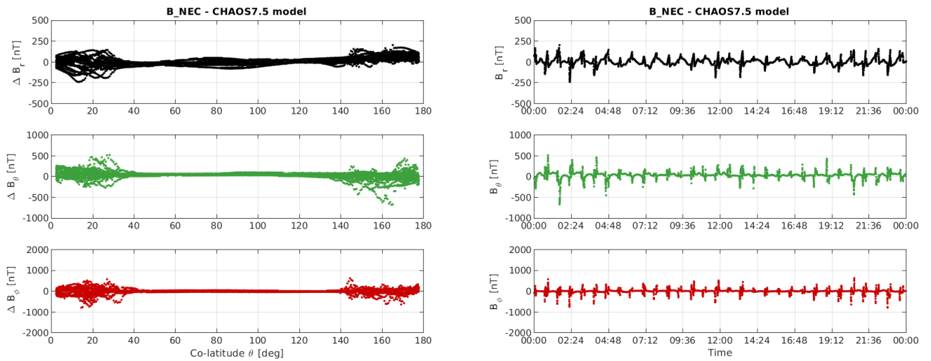
Figure 3-11: S/C B day 22/05: time series of B_{NEC} - B_{Chaos} residuals (right) and B_{NEC} - B_{Chaos} vs colatitude (left).
