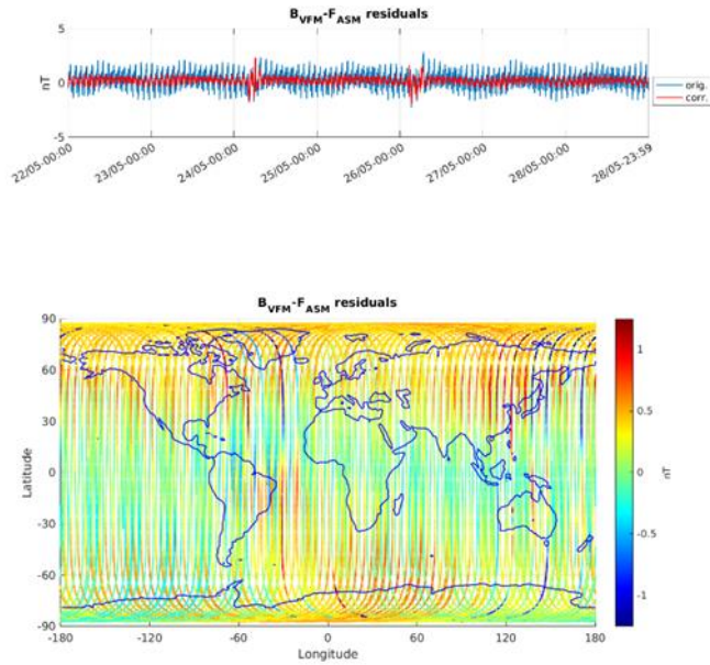
Figure 3-5: ASM-VFM residuals for S/C A, during monitoring period 22/05-28/05. In top figure are plotted: difference between |B_{VFM}| and F_{ASM} (without dB_Sun correction) (blue colour), and the residuals with dB_Sun corrections (red colour). In bottom figure residuals are presented on the world map.
