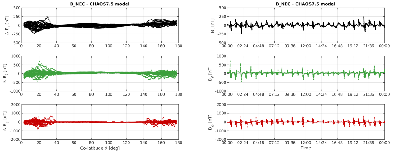
Figure 3-10: S/C A day 22/05: time series of B_{NEC} - B_{Chaos} residuals (right) and B_{NEC} - B_{Chaos} vs colatitude (left).
