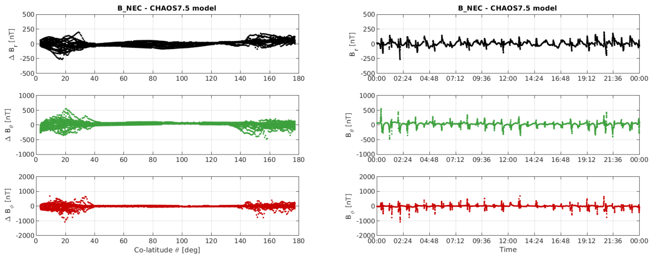
Figure 3-12: S/C C day 22/05: time series of B_{NEC} - B_{Chaos} residuals (right) and B_{NEC} - B_{Chaos} vs colatitude (left)
