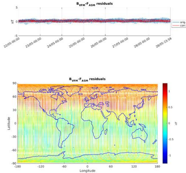
Figure 3-6: ASM-VFM residuals for S/C B, during monitoring period 22/05-28/05. In top figure are plotted: difference between |B_{VFM}| and F_{ASM} (without dB_Sun correction) (blue colour), and the residuals with dB_Sun corrections (red colour). In bottom figure residuals are presented on the world map.
