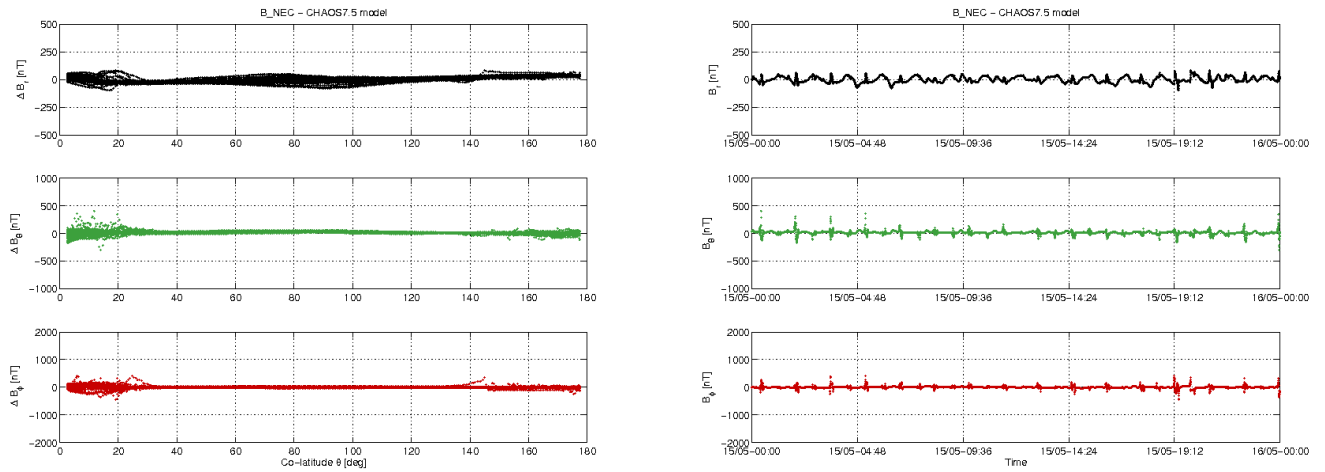
Figure 3-10: S/C A day 15/05: time series of B_{NEC} - B_{Chaos} residuals (right) and B_{NEC} - B_{Chaos} vs colatitude (left).
