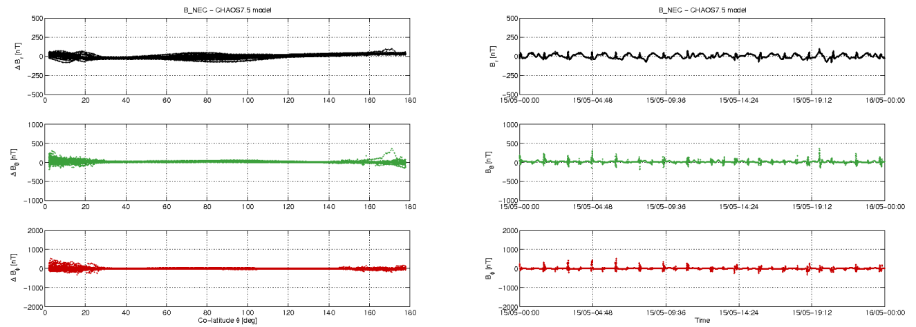
Figure 3-11: S/C B day 15/05: time series of B_{NEC} - B_{Chaos} residuals (right) and B_{NEC} - B_{Chaos} vs colatitude (left).
