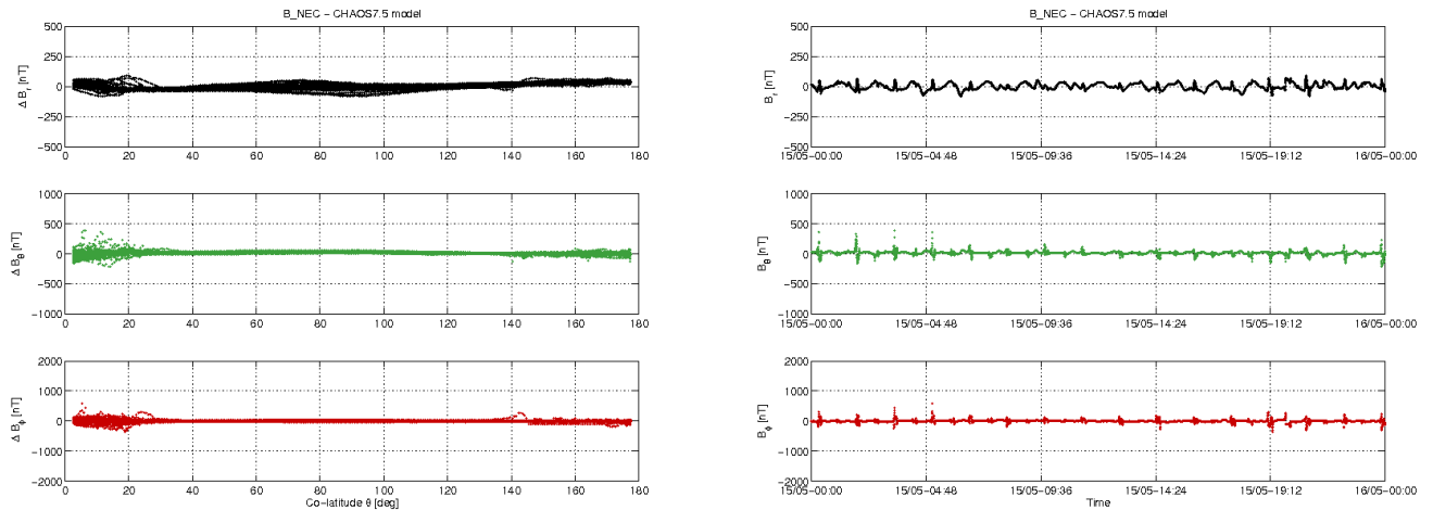
Figure 3-12: S/C C day 15/05: time series of B_{NEC} - B_{Chaos} residuals (right) and B_{NEC} - B_{Chaos} vs colatitude (left)
