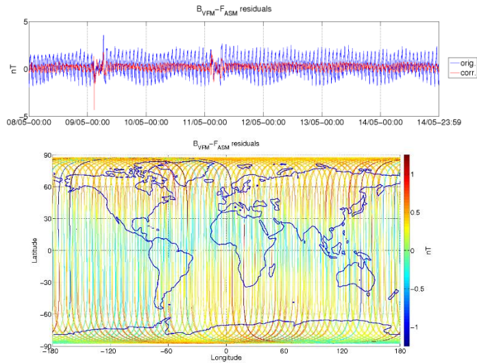
Figure 3-5: ASM-VFM residuals for S/C A, during monitoring period 08/05-14/05. In top figure are plotted: difference between |B_{VFM}| and F_{ASM} (without dB_{Sun} correction) (blue colour), and the residuals with dB_{Sun} corrections (red colour). In bottom figure residuals are presented on the world map.
