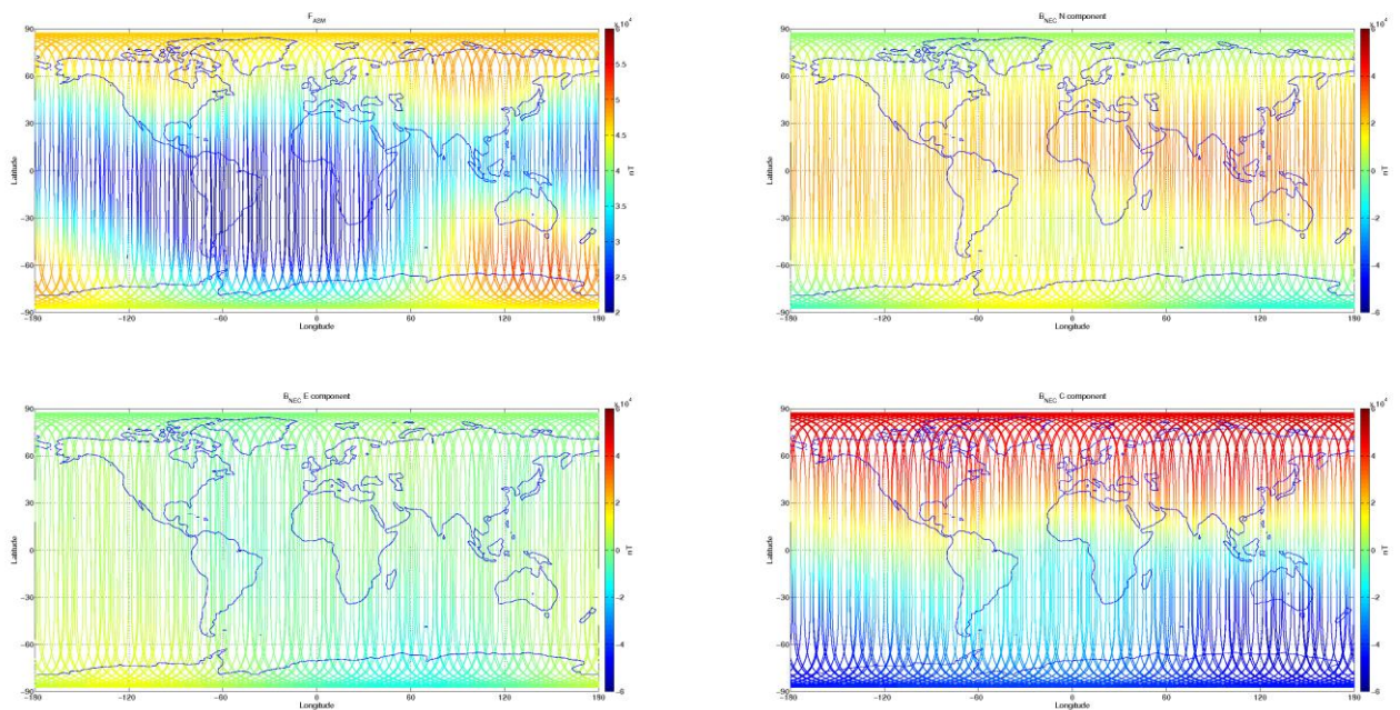
Figure 3-7: S/C A, world map plots of the geomagnetic field and components measured during monitoring period 08/05-14/05. From top to bottom: F-magnetic field from ASM measurement, B_{NEC} components (North, East, and Centre) of magnetic field from VFM measurement.
