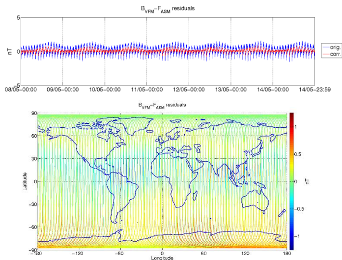
Figure 3-6: ASM-VFM residuals for S/C B, during monitoring period 08/05-14/05. In top figure are plotted: difference between |B_{VFM}| and F_{ASM} (without dB_{Sun} correction) (blue colour), and the residuals with dB_{Sun} corrections (red colour). In bottom figure residuals are presented on the world map.
