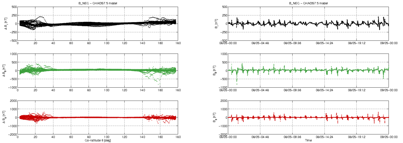
Figure 3-10: S/C A day 08/05: time series of B_{NEC} - B_{Chaos} residuals (right) and B_{NEC} - B_{Chaos} vs colatitude (left).
