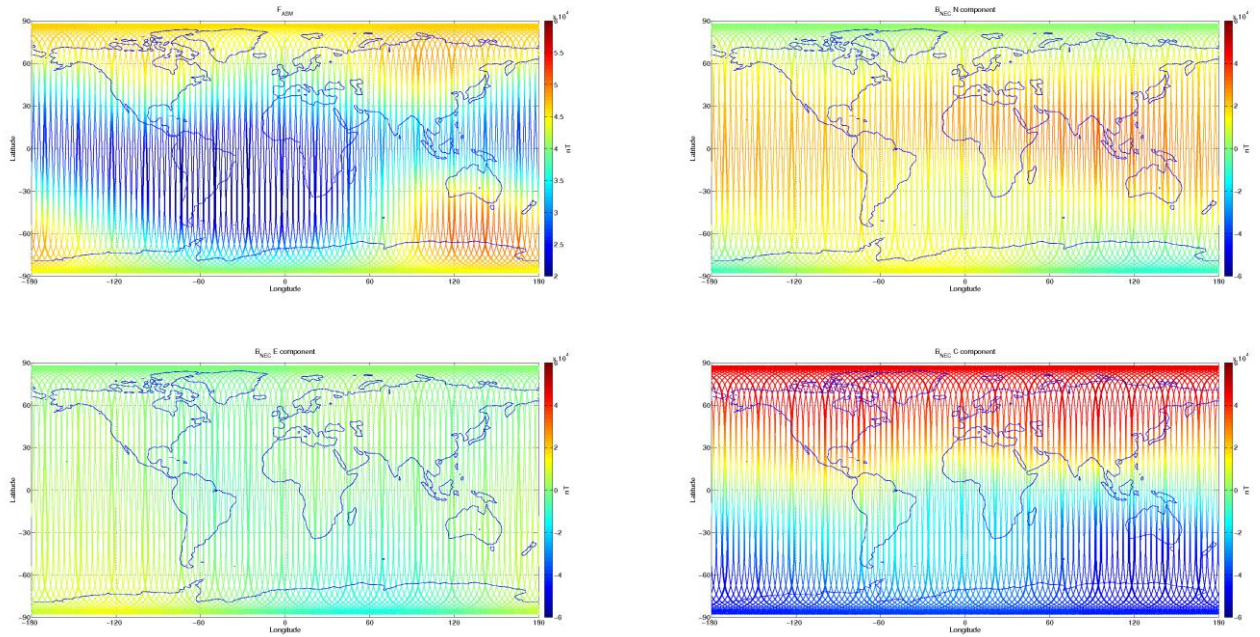
Figure 3-8: S/C B, world map plots of the geomagnetic field and components measured during monitoring period 08/05-14/05. From top to bottom: F-magnetic field from ASM measurement, B_{NEC} components (North, East, and Centre) of magnetic field from VFM measurement.
