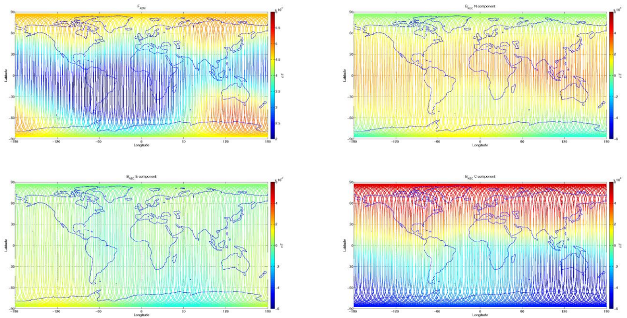
Figure 3-7: S/C A, world map plots of the geomagnetic field and components measured during monitoring period 01/05-07/05. From top to bottom: F-magnetic field from ASM measurement, B_{NEC} components (North, East, and Centre) of magnetic field from VFM measurement.
