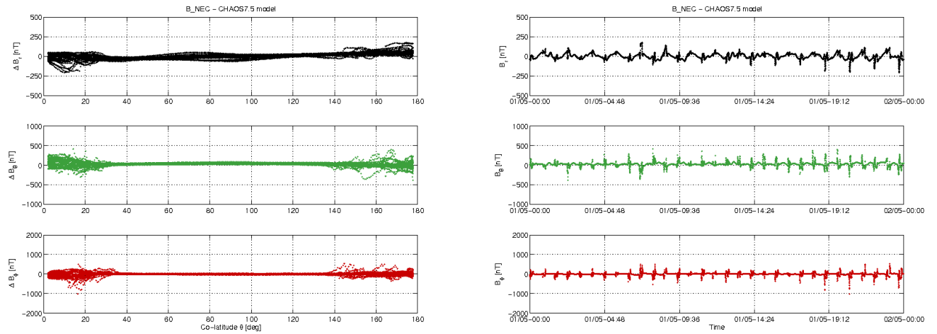
Figure 3-11: S/C B day 01/05: time series of B_{NEC} - B_{Chaos} residuals (right) and B_{NEC} - B_{Chaos} vs colatitude (left).
