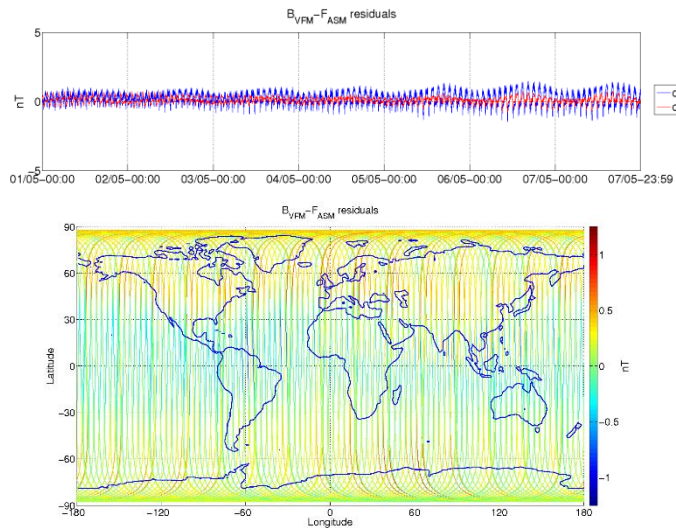
Figure 3-6: ASM-VFM residuals for S/C B, during monitoring period 01/05-07/05. In top figure are plotted: difference between |B_{VFM}| and F_{ASM} (without dB_{Sun} correction) (blue colour), and the residuals with dB_{Sun} corrections (red colour). In bottom figure residuals are presented on the world map.
