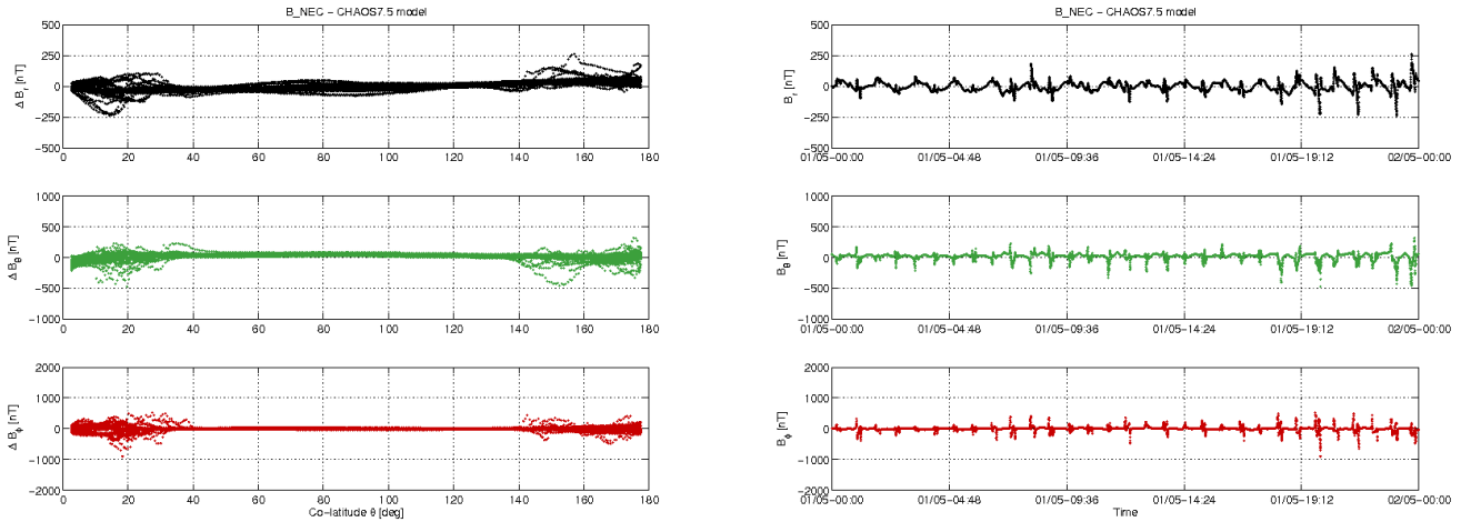
Figure 3-10: S/C A day 01/05: time series of B_{NEC} - B_{Chaos} residuals (right) and B_{NEC} - B_{Chaos} vs colatitude (left).
