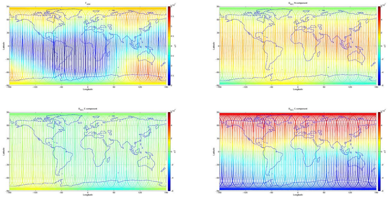
Figure 3-8: S/C B, world map plots of the geomagnetic field and components measured during monitoring period 01/05-07/05. From top to bottom: F-magnetic field from ASM measurement, B_{NEC} components (North, East, and Centre) of magnetic field from VFM measurement.
