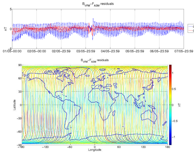
Figure 3-5: ASM-VFM residuals for S/C A, during monitoring period 01/05-07/05. In top figure are plotted: difference between |B_{VFM}| and F_{ASM} (without dB_{Sun} correction) (blue colour), and the residuals with dB_{Sun} corrections (red colour). In bottom figure residuals are presented on the world map.
