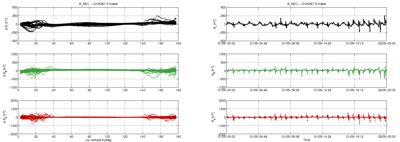
Figure 3-12: S/C C day 01/05: time series of B_{NEC} - B_{Chaos} residuals (right) and B_{NEC} - B_{Chaos} vs colatitude (left)
