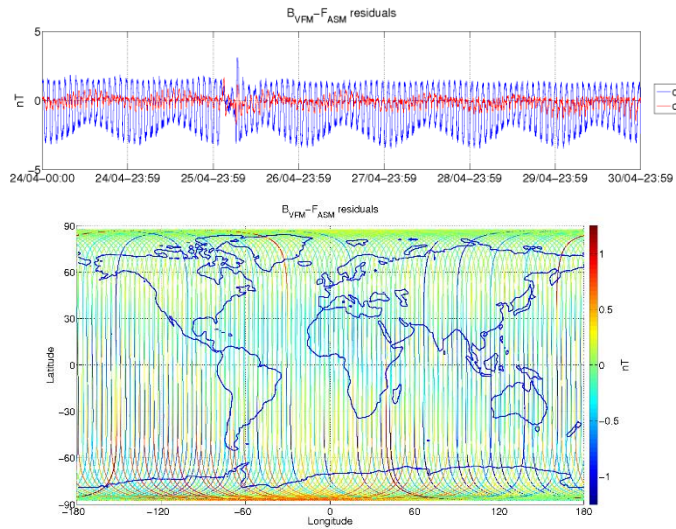
Figure 3-5: ASM-VFM residuals for S/C A, during monitoring period 24/04-30/04. In top figure are plotted: difference between |B_{VFM}| and F_{ASM} (without dB_{Sun} correction) (blue colour), and the residuals with dB_{Sun} corrections (red colour). In bottom figure residuals are presented on the world map.
