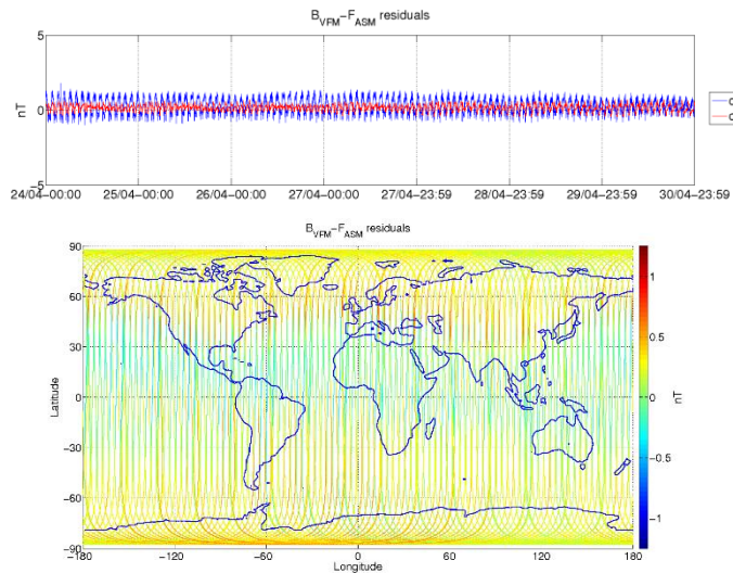
Figure 3-6: ASM-VFM residuals for S/C B, during monitoring period 24/04-30/04. In top figure are plotted: difference between |B_{VFM}| and F_{ASM} (without dB_{Sun} correction) (blue colour), and the residuals with dB_{Sun} corrections (red colour). In bottom figure residuals are presented on the world map.
