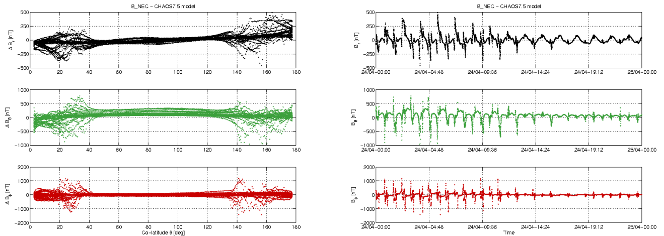
Figure 3-12: S/C C day 24/04: time series of B_{NEC} - B_{Chaos} residuals (right) and B_{NEC} - B_{Chaos} vs colatitude (left)
