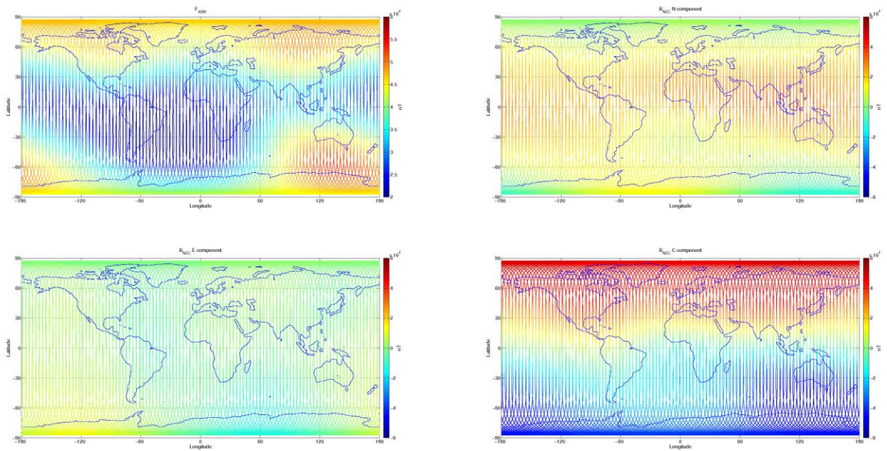
Figure 3-7: S/C A, world map plots of the geomagnetic field and components measured during monitoring period 24/04-30/04. From top to bottom: F-magnetic field from ASM measurement, B_{NEC} components (North, East, and Centre) of magnetic field from VFM measurement.
