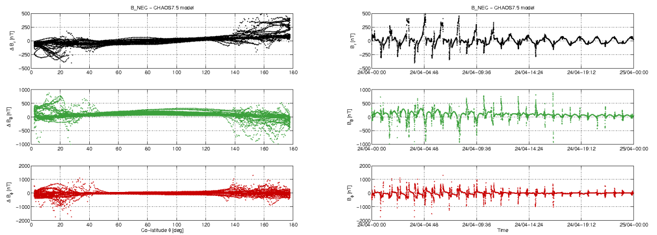
Figure 3-11: S/C B day 24/04: time series of B_{NEC} - B_{Chaos} residuals (right) and B_{NEC} - B_{Chaos} vs colatitude (left).
