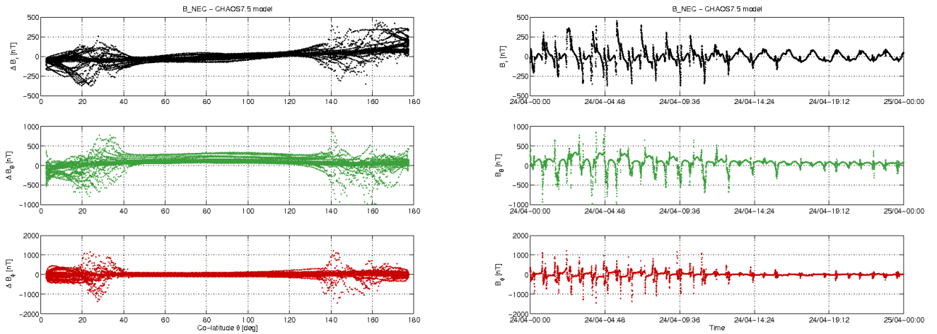
Figure 3-10: S/C A day 24/04: time series of B_{NEC} - B_{Chaos} residuals (right) and B_{NEC} - B_{Chaos} vs colatitude (left).
