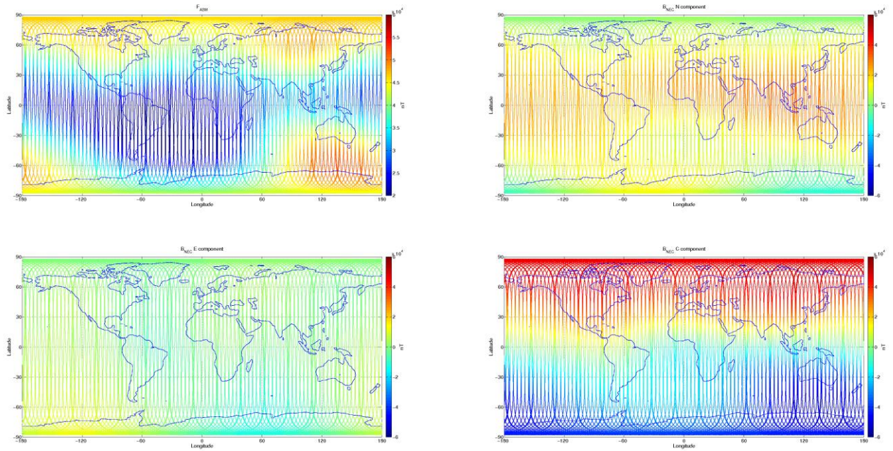
Figure 3-8: S/C B, world map plots of the geomagnetic field and components measured during monitoring period 24/04-30/04. From top to bottom: F-magnetic field from ASM measurement, B_{NEC} components (North, East, and Centre) of magnetic field from VFM measurement.
