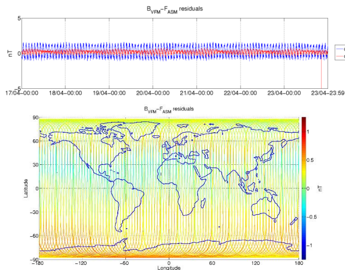
Figure 3-6: ASM-VFM residuals for S/C B, during monitoring period 17/04-23/04. In top figure are plotted: difference between |B_{VFM}| and F_{ASM} (without dB_{Sun} correction) (blue colour), and the residuals with dB_{Sun} corrections (red colour). In bottom figure residuals are presented on the world map.
