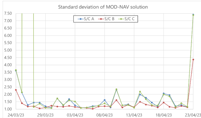
Figure 3-1: Plot of the standard deviation of the difference between MOD and NAV solutions for all satellites.
