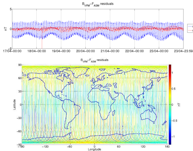
Figure 3-5: ASM-VFM residuals for S/C A, during monitoring period 17/04-23/04. In top figure are plotted: difference between |B_{VFM}| and F_{ASM} (without dB_{Sun} correction) (blue colour), and the residuals with dB_{Sun} corrections (red colour). In bottom figure residuals are presented on the world map.
