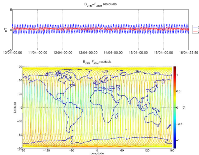
Figure 3-6: ASM-VFM residuals for S/C B, during monitoring period 10/04-16/04. In top figure are plotted: difference between |B_{VFM}| and F_{ASM} (without dB_{Sun} correction) (blue colour), and the residuals with dB_{Sun} corrections (red colour). In bottom figure residuals are presented on the world map.
