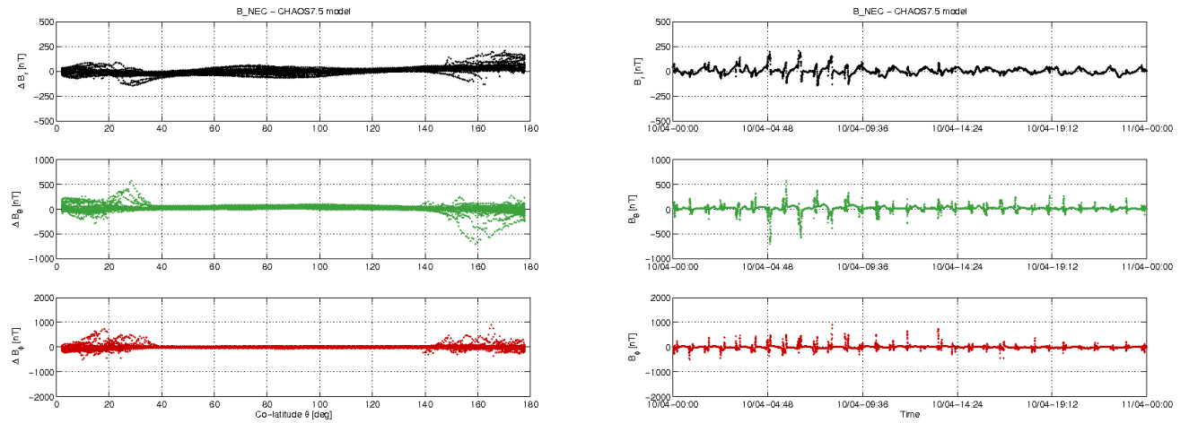
Figure 3-11: S/C B day 10/04: time series of B_{NEC} - B_{Chaos} residuals (right) and B_{NEC} - B_{Chaos} vs colatitude (left).
