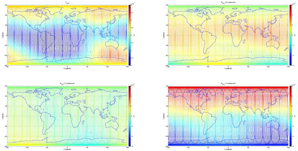
Figure 3-8: S/C B, world map plots of the geomagnetic field and components measured during monitoring period 10/04-16/04. From top to bottom: F-magnetic field from ASM measurement, B_{NEC} components (North, East, and Centre) of magnetic field from VFM measurement.
