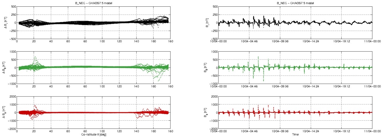
Figure 3-10: S/C A day 10/04: time series of B_{NEC} - B_{Chaos} residuals (right) and B_{NEC} - B_{Chaos} vs colatitude (left).
