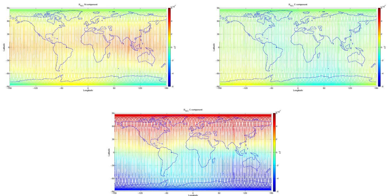
Figure 3-9: S/C C, world map plots of the geomagnetic field and components measured during monitoring period 10/04-16/04. From top to bottom: B_{NEC} components (North, East, and Centre) of magnetic field from VFM measurement.
