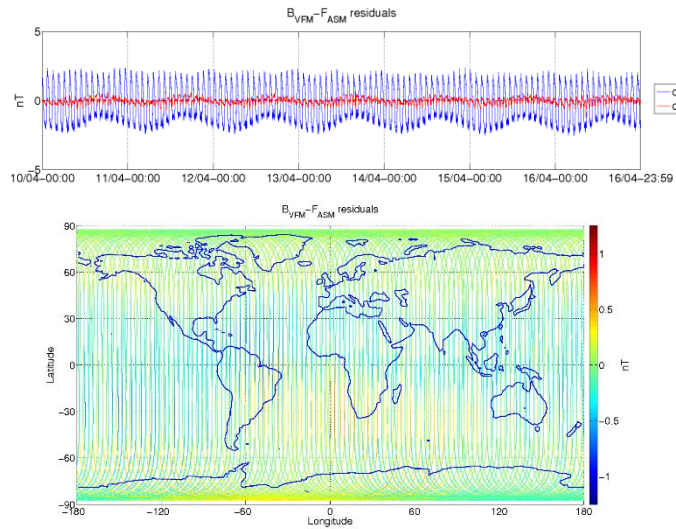
Figure 3-5: ASM-VFM residuals for S/C A, during monitoring period 10/04-16/04. In top figure are plotted: difference between |B_{VFM}| and F_{ASM} (without dB_{Sun} correction) (blue colour), and the residuals with dB_{Sun} corrections (red colour). In bottom figure residuals are presented on the world map.
