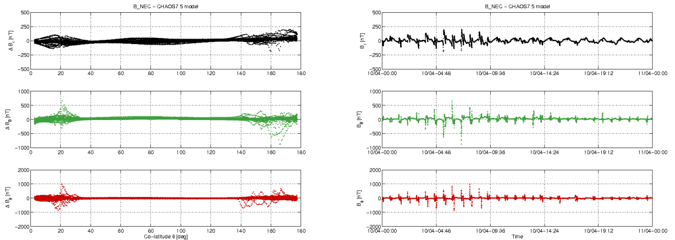
Figure 3-12: S/C C day 10/04: time series of B_{NEC} - B_{Chaos} residuals (right) and B_{NEC} - B_{Chaos} vs colatitude (left)
