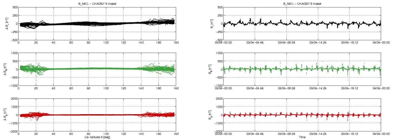
Figure 3-11: S/C B day 03/04: time series of B_{NEC} - B_{Chaos} residuals (right) and B_{NEC} - B_{Chaos} vs colatitude (left).
