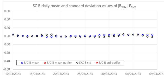
Figure 3-4: Daily mean and standard deviation values of ASM-VFM residuals (defined as dF = |B_{VFM}| - F_{ASM} ) for S/C B. Peak registered on 9 th April 2023 due to ASM F parameter being set to zero, could be related to Burst Mode session started on 10 th April 2023.
