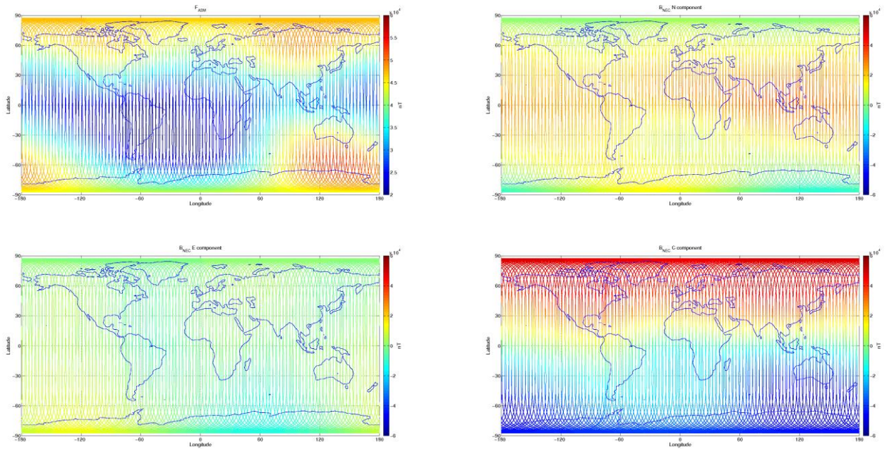
Figure 3-7: S/C A, world map plots of the geomagnetic field and components measured during monitoring period 03/04-09/04. From top to bottom: F-magnetic field from ASM measurement, B_{NEC} components (North, East, and Centre) of magnetic field from VFM measurement.
