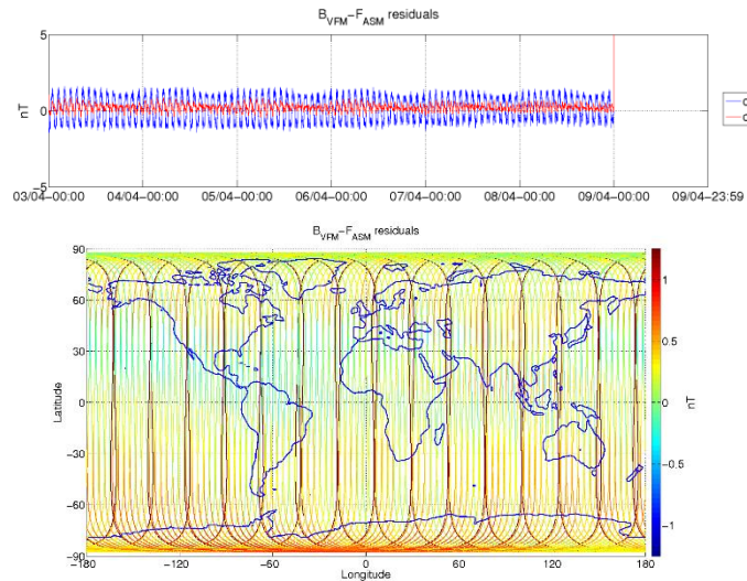
Figure 3-6: ASM-VFM residuals for S/C B, during monitoring period 03/04-09/04. In top figure are plotted: difference between |B_{VFM}| and F_{ASM} (without dB_{Sun} correction) (blue colour), and the residuals with dB_{Sun} corrections (red colour). In bottom figure residuals are presented on the world map.
