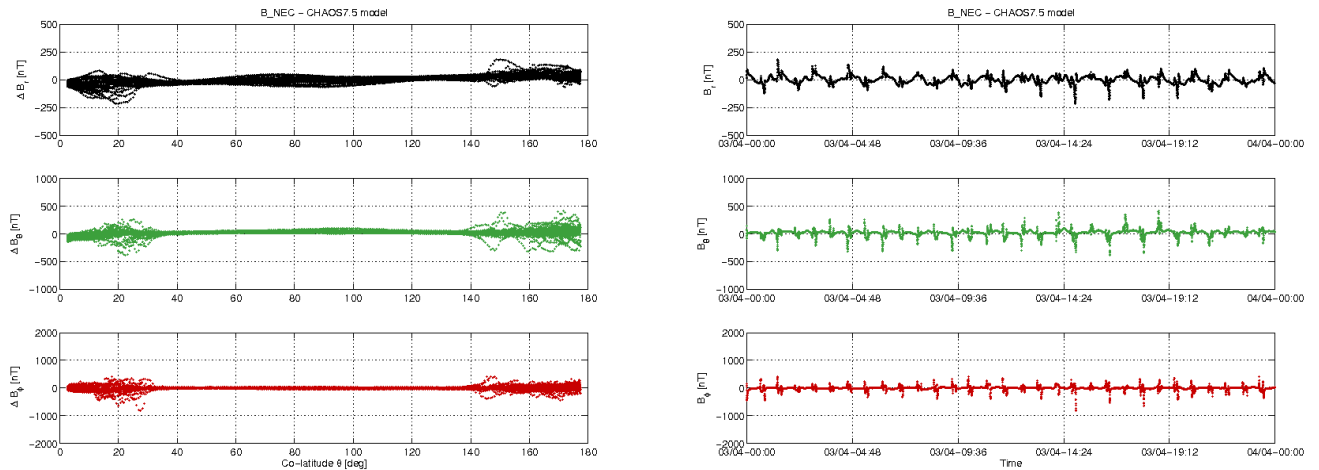
Figure 3-12: S/C C day 03/04: time series of B_{NEC} - B_{Chaos} residuals (right) and B_{NEC} - B_{Chaos} vs colatitude (left)
