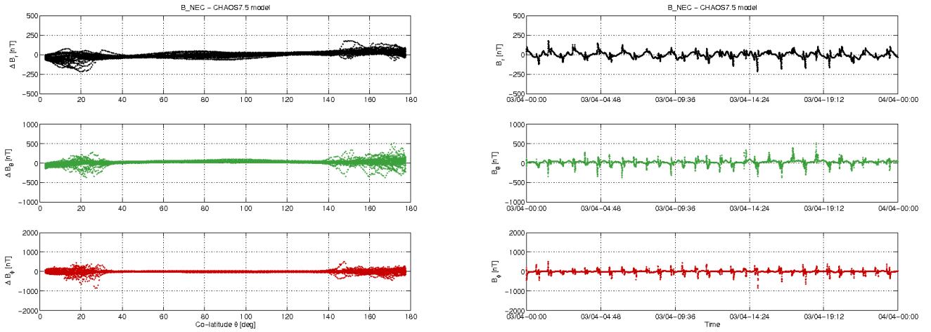
Figure 3-10: S/C A day 03/04: time series of B_{NEC} - B_{Chaos} residuals (right) and B_{NEC} - B_{Chaos} vs colatitude (left).
