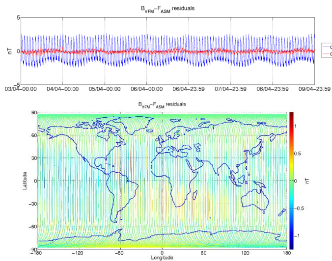
Figure 3-5: ASM-VFM residuals for S/C A, during monitoring period 03/04-09/04. In top figure are plotted: difference between |B_{VFM}| and F_{ASM} (without dB_{Sun} correction) (blue colour), and the residuals with dB_{Sun} corrections (red colour). In bottom figure residuals are presented on the world map.
