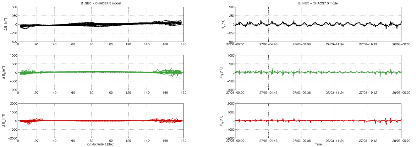
Figure 3-10: S/C A day 27/03: time series of B_{NEC} - B_{Chaos} residuals (right) and B_{NEC} - B_{Chaos} vs colatitude (left).
