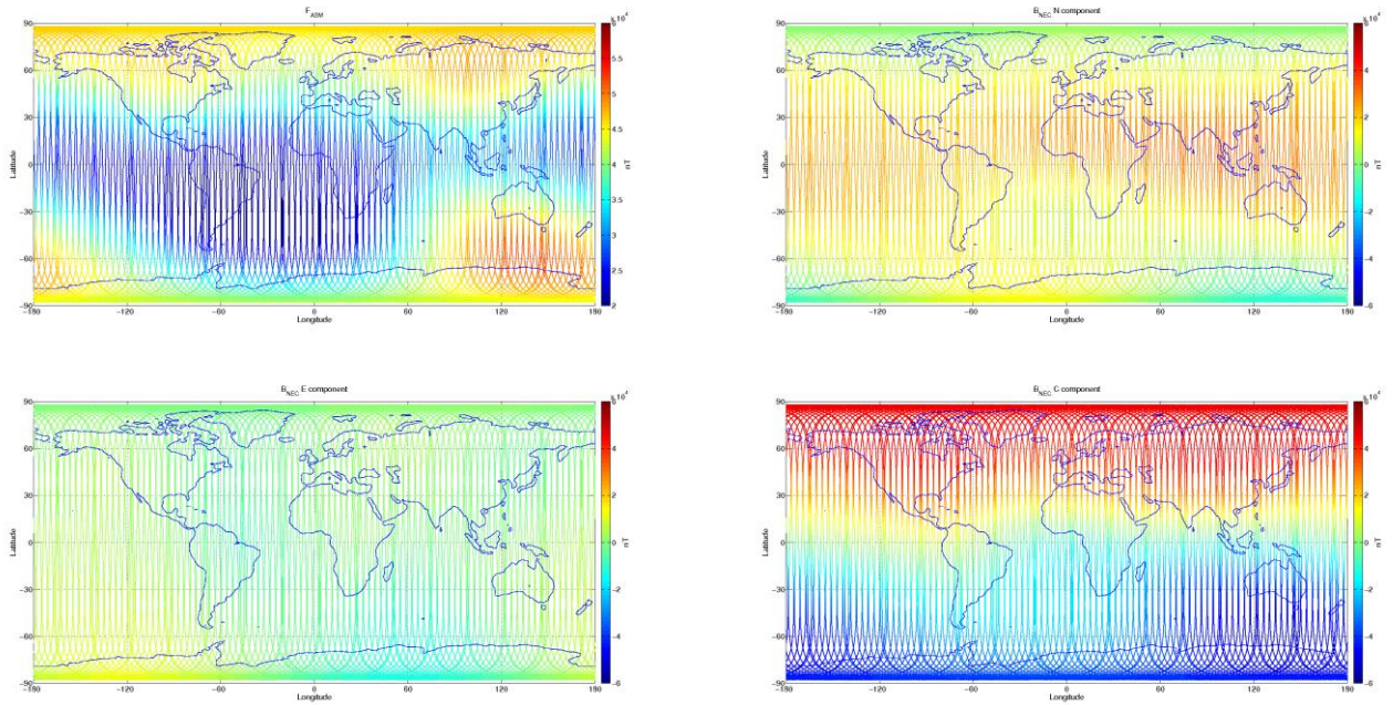
Figure 3-8: S/C B, world map plots of the geomagnetic field and components measured during monitoring period 27/03-02/04. From top to bottom: F-magnetic field from ASM measurement, B_{NEC} components (North, East, and Centre) of magnetic field from VFM measurement.
