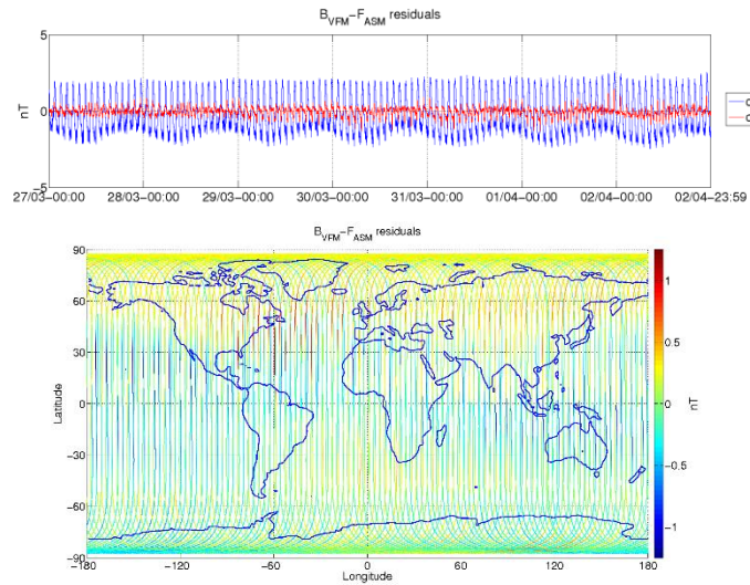
Figure 3-5: ASM-VFM residuals for S/C A, during monitoring period 27/03-02/04. In top figure are plotted: difference between |B_{VFM}| and F_{ASM} (without dB_{Sun} correction) (blue colour), and the residuals with dB_{Sun} corrections (red colour). In bottom figure residuals are presented on the world map.
