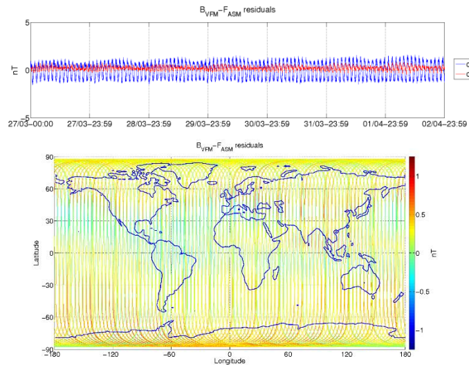
Figure 3-6: ASM-VFM residuals for S/C B, during monitoring period 27/03-02/04. In top figure are plotted: difference between |B_{VFM}| and F_{ASM} (without dB_{Sun} correction) (blue colour), and the residuals with dB_{Sun} corrections (red colour). In bottom figure residuals are presented on the world map.
