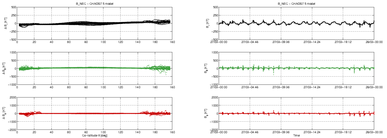
Figure 3-12: S/C C day 27/03: time series of B_{NEC} - B_{Chaos} residuals (right) and B_{NEC} - B_{Chaos} vs colatitude (left)
