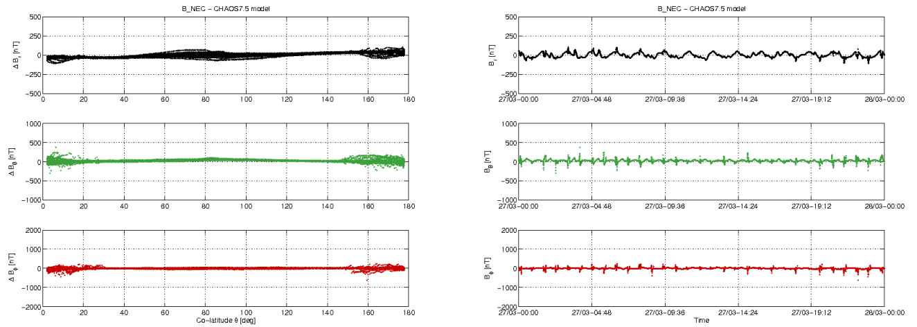
Figure 3-11: S/C B day 27/03: time series of B_{NEC} - B_{Chaos} residuals (right) and B_{NEC} - B_{Chaos} vs colatitude (left).
