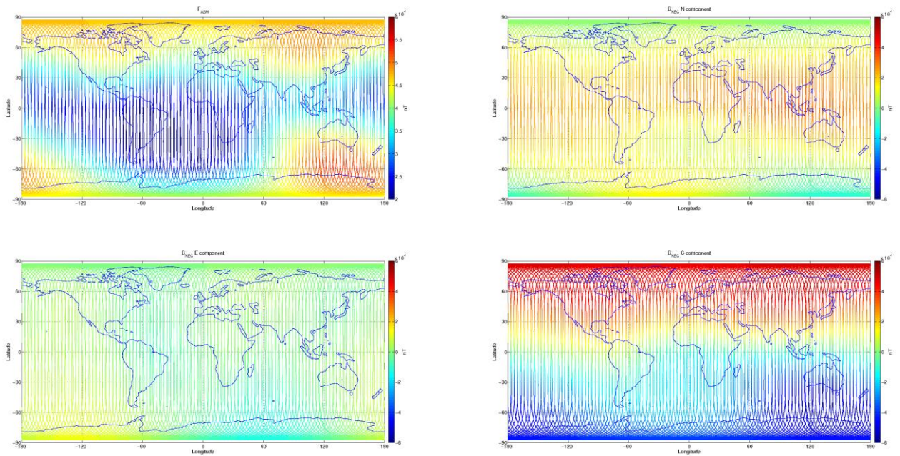
Figure 3-7: S/C A, world map plots of the geomagnetic field and components measured during monitoring period 27/03-02/04. From top to bottom: F-magnetic field from ASM measurement, B_{NEC} components (North, East, and Centre) of magnetic field from VFM measurement.
