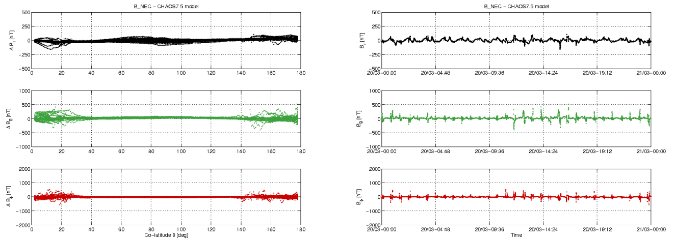
Figure 3-11: S/C B day 20/03: time series of B_{NEC} - B_{Chaos} residuals (right) and B_{NEC} - B_{Chaos} vs colatitude (left).
