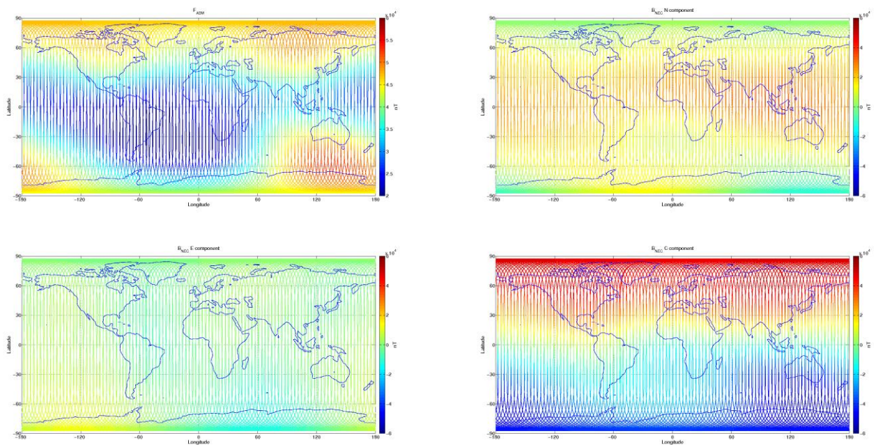
Figure 3-7: S/C A, world map plots of the geomagnetic field and components measured during monitoring period 20/03-26/03. From top to bottom: F-magnetic field from ASM measurement, B_{NEC} components (North, East, and Centre) of magnetic field from VFM measurement.
