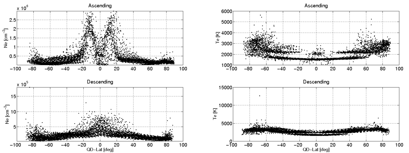
Figure 3-18: The panels show the electron density (left) and temperature (right) profile as a function of QD Latitudes for the last week of operation. The analysis is made separately for ascending (upper panels) and descending (bottom panels) orbits.
