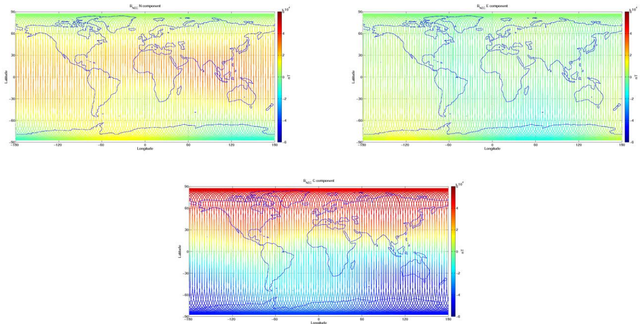
Figure 3-9: S/C C, world map plots of the geomagnetic field and components measured during monitoring period 20/03-26/03. From top to bottom: B_{NEC} components (North, East, and Centre) of magnetic field from VFM measurement.
