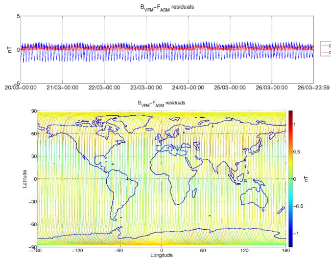
Figure 3-6: ASM-VFM residuals for S/C B, during monitoring period 20/03-26/03. In top figure are plotted: difference between |B_{VFM}| and F_{ASM} (without dB_{Sun} correction) (blue colour), and the residuals with dB_{Sun} corrections (red colour). In bottom figure residuals are presented on the world map.
