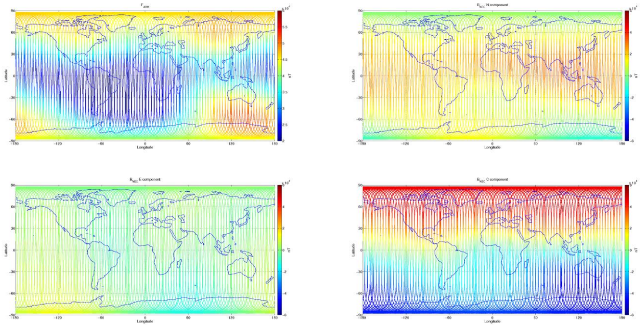
Figure 3-8: S/C B, world map plots of the geomagnetic field and components measured during monitoring period 20/03-26/03. From top to bottom: F-magnetic field from ASM measurement, B_{NEC} components (North, East, and Centre) of magnetic field from VFM measurement.
