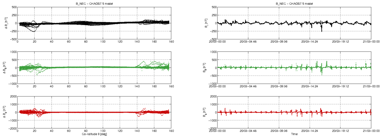
Figure 3-12: S/C C day 20/03: time series of B_{NEC} - B_{Chaos} residuals (right) and B_{NEC} - B_{Chaos} vs colatitude (left)
