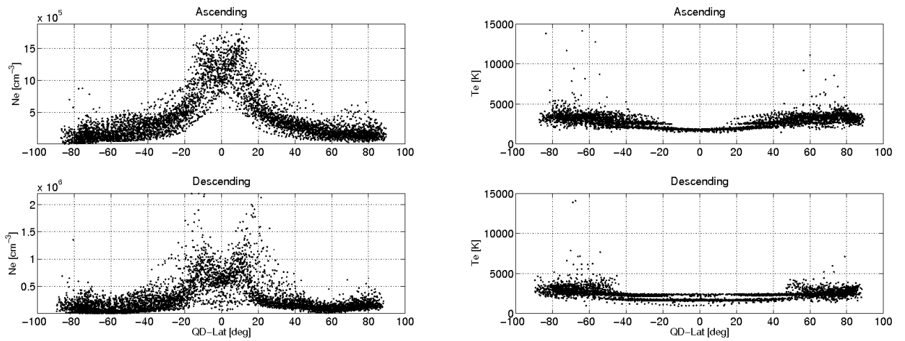
Figure 3-17: The panels show the electron density (left) and temperature (right) profile as a function of QD Latitudes for the last week of operation. The analysis is made separately for ascending (upper panels) and descending (bottom panels) orbits.
