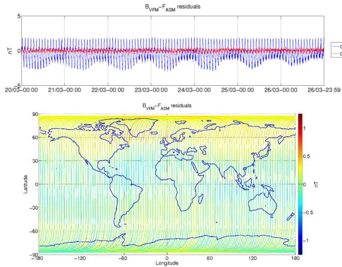
Figure 3-5: ASM-VFM residuals for S/C A, during monitoring period 20/03-26/03. In top figure are plotted: difference between |B_{VFM}| and F_{ASM} (without dB_{Sun} correction) (blue colour), and the residuals with dB_{Sun} corrections (red colour). In bottom figure residuals are presented on the world map.
