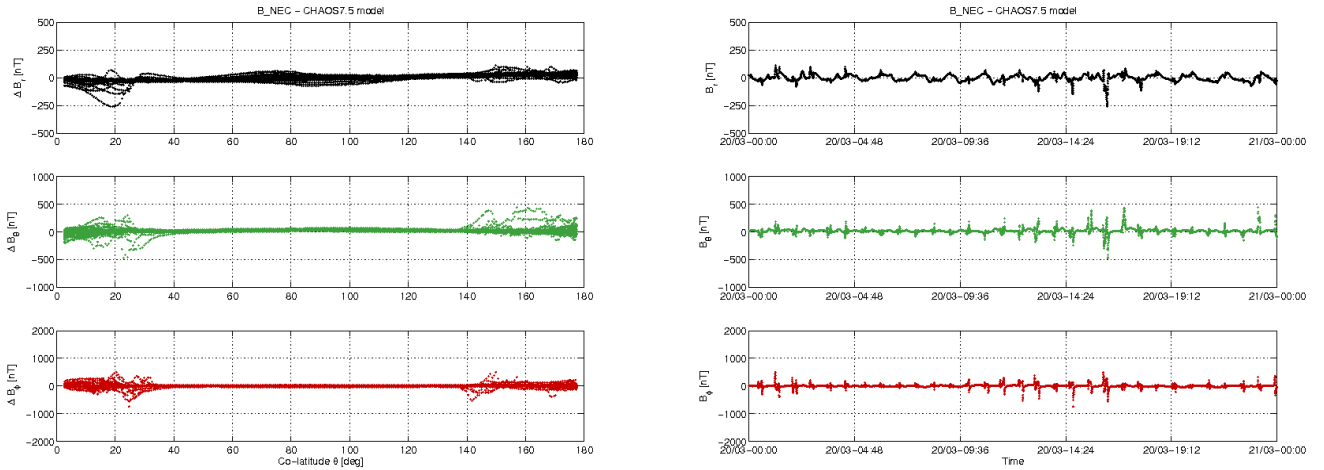
Figure 3-10: S/C A day 20/03: time series of B_{NEC} - B_{Chaos} residuals (right) and B_{NEC} - B_{Chaos} vs colatitude (left).
