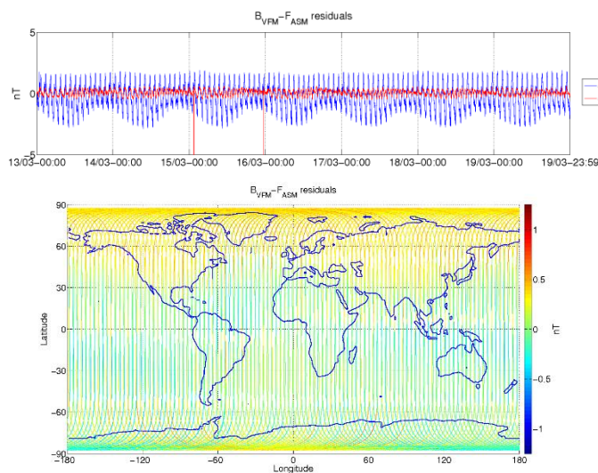
Figure 3-5: ASM-VFM residuals for S/C A, during monitoring period 13/03-19/03. In top figure are plotted: difference between |B_{VFM}| and F_{ASM} (without dB_{Sun} correction) (blue colour), and the residuals with dB_{Sun} corrections (red colour). In bottom figure residuals are presented on the world map.
