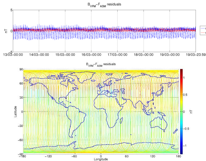
Figure 3-6: ASM-VFM residuals for S/C B, during monitoring period 13/03-19/03. In top figure are plotted: difference between |B_{VFM}| and F_{ASM} (without dB_{Sun} correction) (blue colour), and the residuals with dB_{Sun} corrections (red colour). In bottom figure residuals are presented on the world map.
