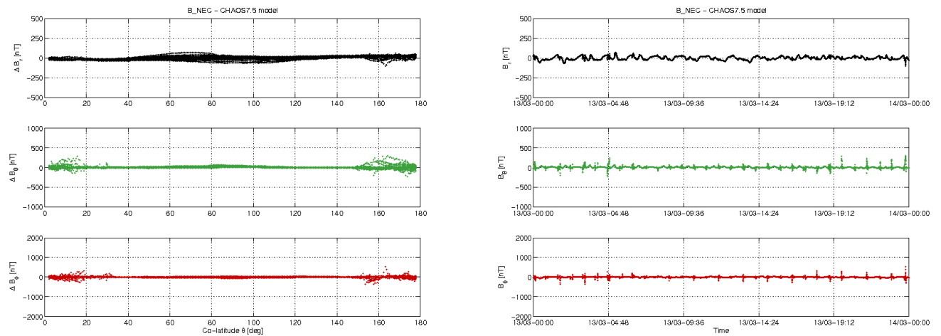
Figure 3-11: S/C B day 13.03: time series of B_{NEC} - B_{Chaos} residuals (right) and B_{NEC} - B_{Chaos} vs colatitude (left).
