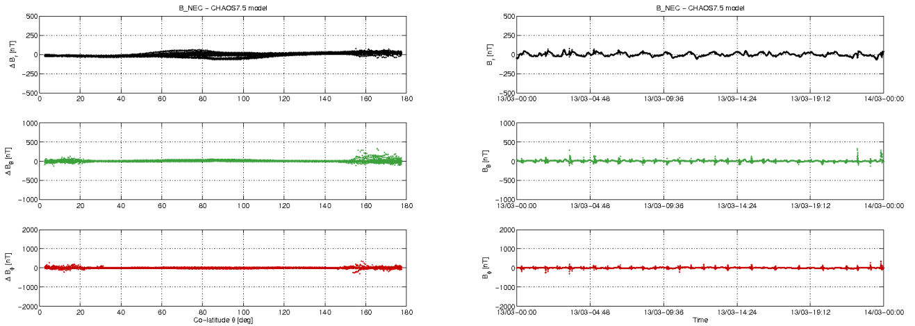
Figure 3-12: S/C C day 1303: time series of B_{NEC} - B_{Chaos} residuals (right) and B_{NEC} - B_{Chaos} vs colatitude (left)
