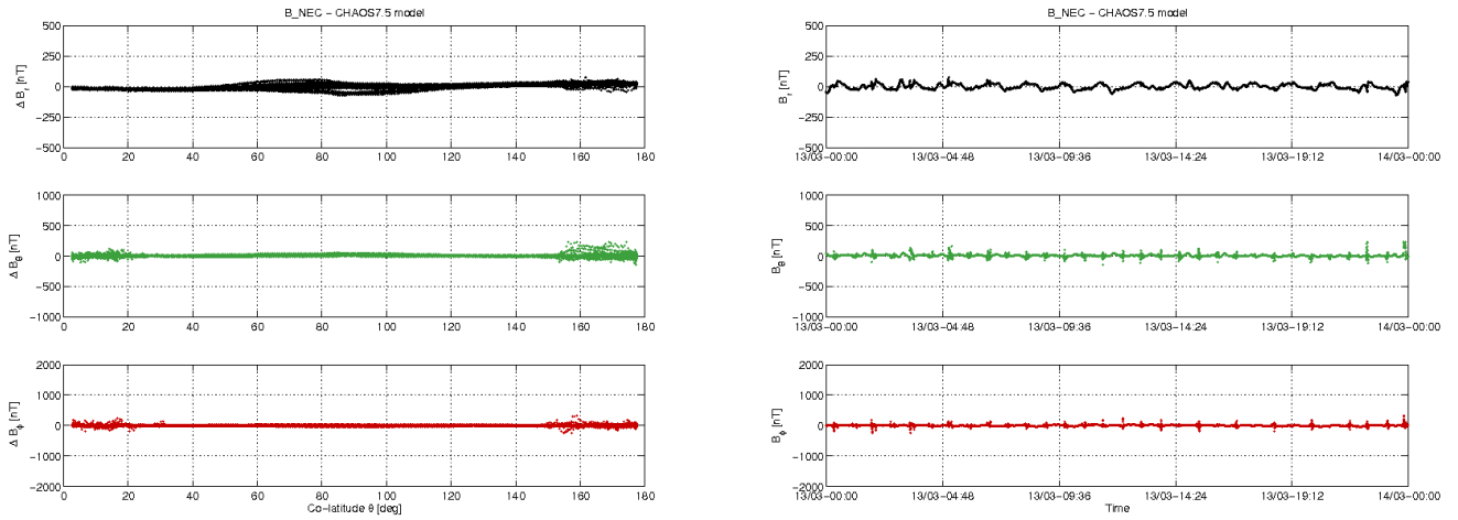
Figure 3-10: S/C A day 13.03: time series of B_{NEC} - B_{Chaos} residuals (right) and B_{NEC} - B_{Chaos} vs colatitude (left).
