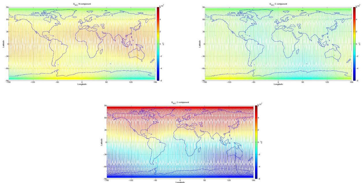
Figure 3-9: S/C C, world map plots of the geomagnetic field and components measured during monitoring period 13/03-19/03. From top to bottom: B_{NEC} components (North, East, and Centre) of magnetic field from VFM measurement.
