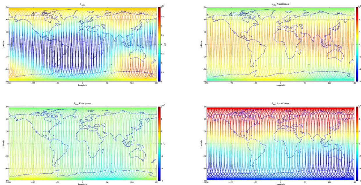
Figure 3-8: S/C B, world map plots of the geomagnetic field and components measured during monitoring period 13/03-19/03. From top to bottom: F-magnetic field from ASM measurement, B_{NEC} components (North, East, and Centre) of magnetic field from VFM measurement.
