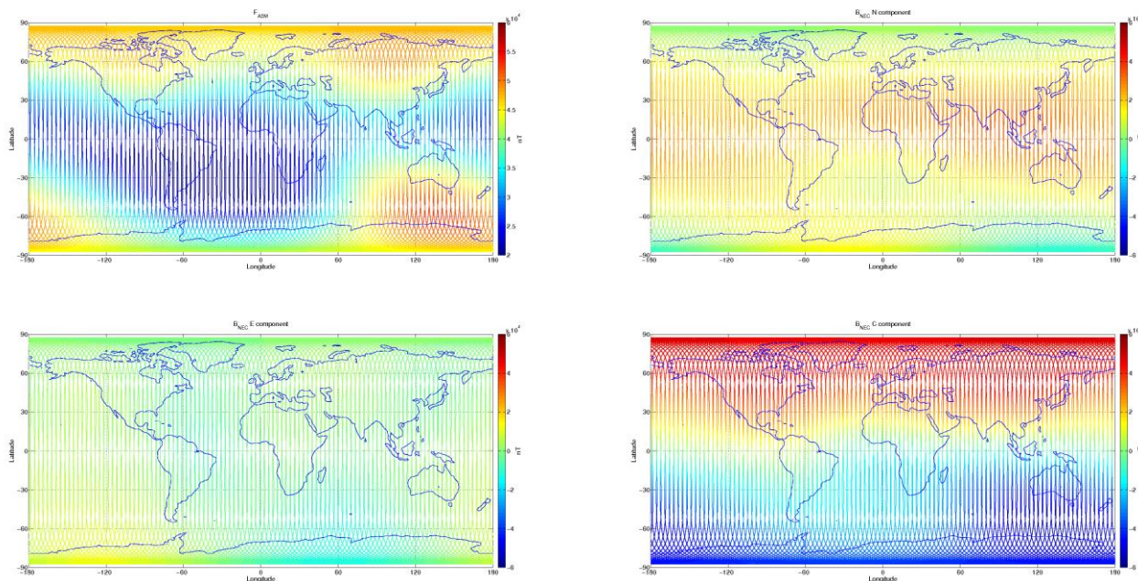
Figure 3-7: S/C A, world map plots of the geomagnetic field and components measured during monitoring period 06/03-12/03. From top to bottom: F-magnetic field from ASM measurement, B_{NEC} components (North, East, and Centre) of magnetic field from VFM measurement.
