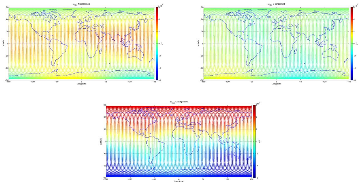
Figure 3-9: S/C C, world map plots of the geomagnetic field and components measured during monitoring period 06/03-12/03. From top to bottom: B_{NEC} components (North, East, and Centre) of magnetic field from VFM measurement.
