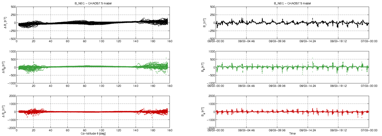
Figure 3-12: S/C C day 06/03: time series of B_{NEC} - B_{Chaos} residuals (right) and B_{NEC} - B_{Chaos} vs colatitude (left)
