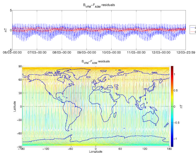
Figure 3-5: ASM-VFM residuals for S/C A, during monitoring period 06/03-12/03. In top figure are plotted: difference between |B_{VFM}| and F_{ASM} (without dB_{Sun} correction) (blue colour), and the residuals with dB_{Sun} corrections (red colour). In bottom figure residuals are presented on the world map.
