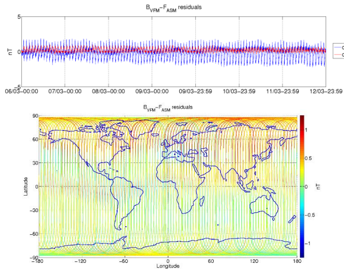
Figure 3-6: ASM-VFM residuals for S/C B, during monitoring period 06/03-12/03. In top figure are plotted: difference between |B_{VFM}| and F_{ASM} (without dB_{Sun} correction) (blue colour), and the residuals with dB_{Sun} corrections (red colour). In bottom figure residuals are presented on the world map.
