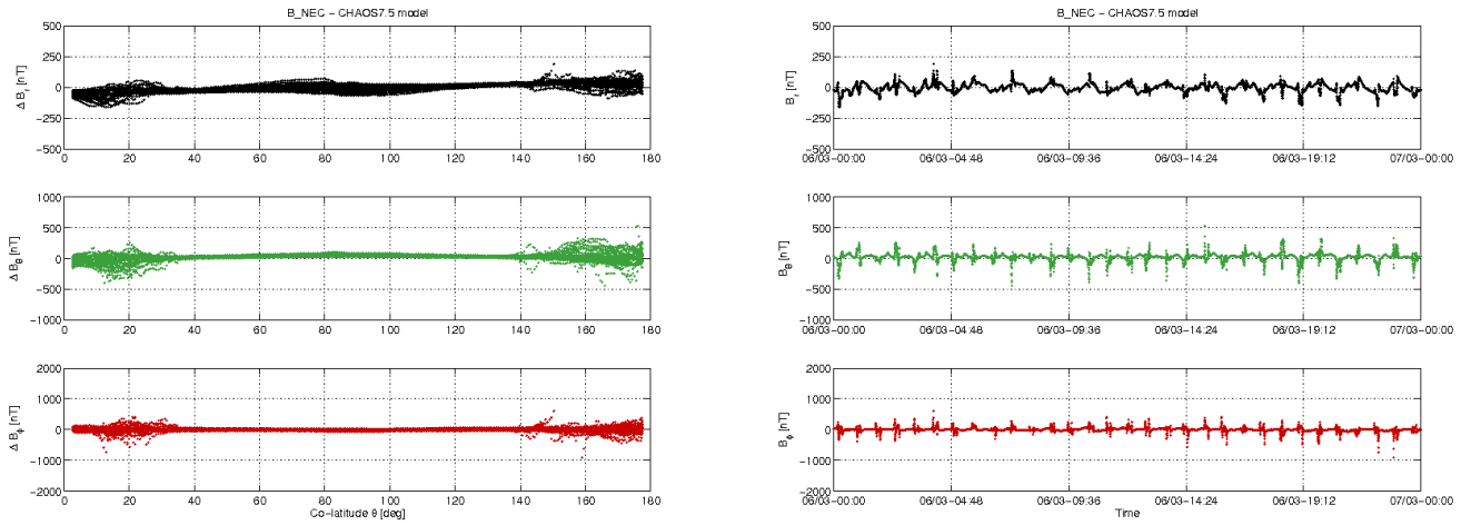
Figure 3-10: S/C A day 06.03: time series of B_{NEC} - B_{Chaos} residuals (right) and B_{NEC} - B_{Chaos} vs colatitude (left).
