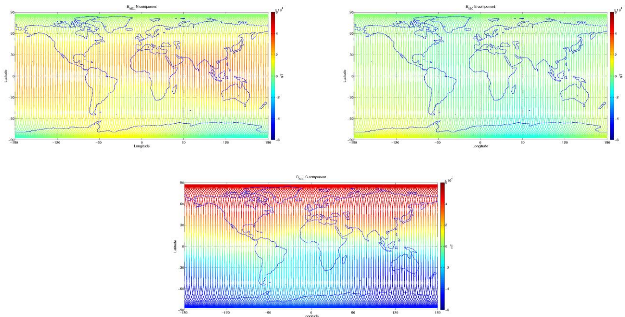
Figure 3-9: S/C C, world map plots of the geomagnetic field and components measured during monitoring period 27/02-05/03. From top to bottom: B_{NEC} components (North, East, and Centre) of magnetic field from VFM measurement.
