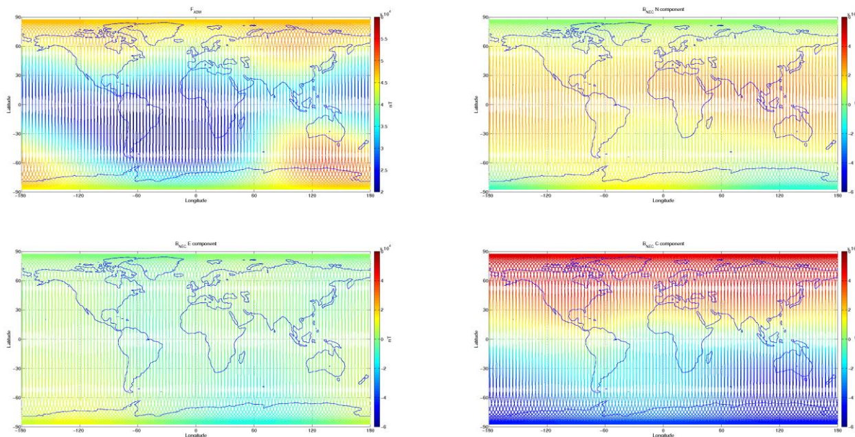
Figure 3-7: S/C A, world map plots of the geomagnetic field and components measured during monitoring period 27/02-05/03. From top to bottom: F-magnetic field from ASM measurement, B_{NEC} components (North, East, and Centre) of magnetic field from VFM measurement.
