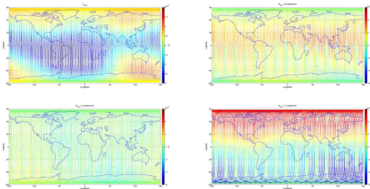
Figure 3-8: S/C B, world map plots of the geomagnetic field and components measured during monitoring period 27/02-05/03. From top to bottom: F-magnetic field from ASM measurement, B_{NEC} components (North, East, and Centre) of magnetic field from VFM measurement.
