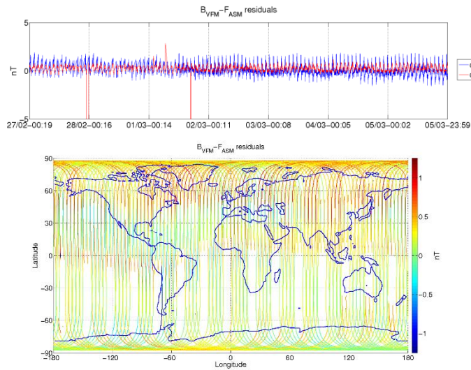
Figure 3-6: ASM-VFM residuals for S/C B, during monitoring period 27/02-05/03. In top figure are plotted: difference between |B_{VFM}| and F_{ASM} (without dB_{Sun} correction) (blue colour), and the residuals with dB_{Sun} corrections (red colour). In bottom figure residuals are presented on the world map.
