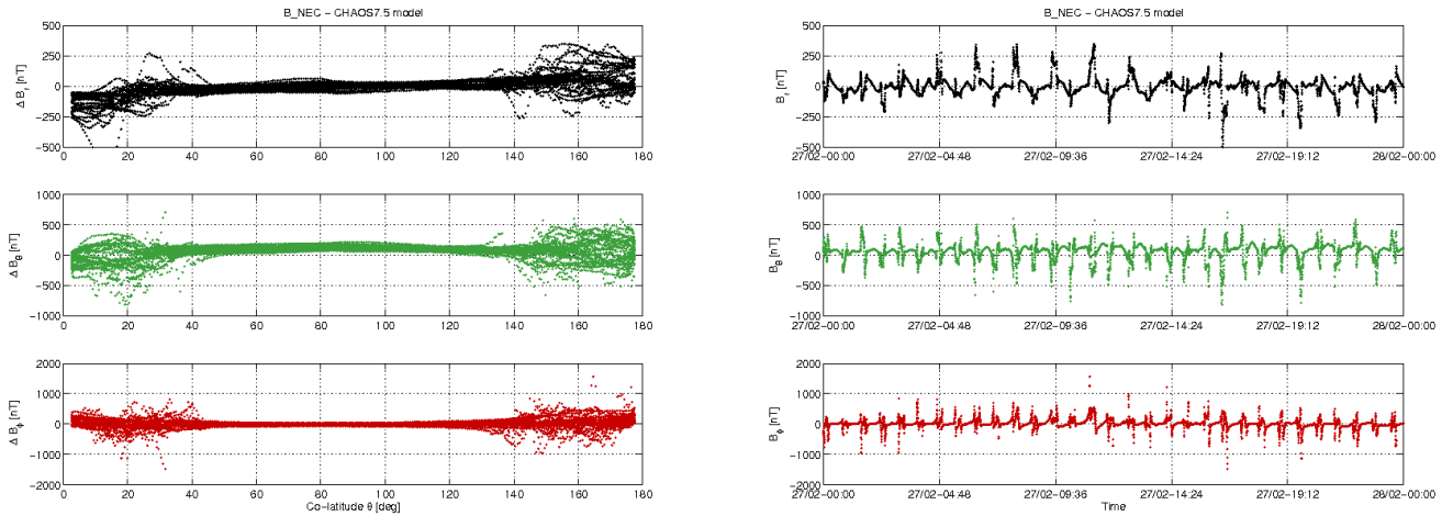
Figure 3-10: S/C A day 27/02: time series of B_{NEC} - B_{Chaos} residuals (right) and B_{NEC} - B_{Chaos} vs colatitude (left).
