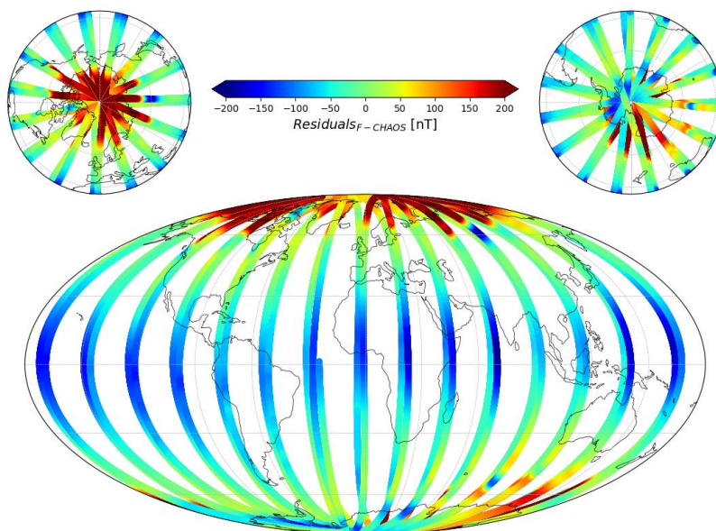
Figure 4-1 Residuals between the magnetic field intensity F measured by Swarm A-ASM and the Chaos model on 27 February 2023.
