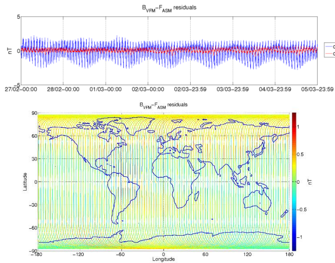
Figure 3-5: ASM-VFM residuals for S/C A, during monitoring period 27/02-05/03. In top figure are plotted: difference between |B_{VFM}| and F_{ASM} (without dB_{Sun} correction) (blue colour), and the residuals with dB_{Sun} corrections (red colour). In bottom figure residuals are presented on the world map.
