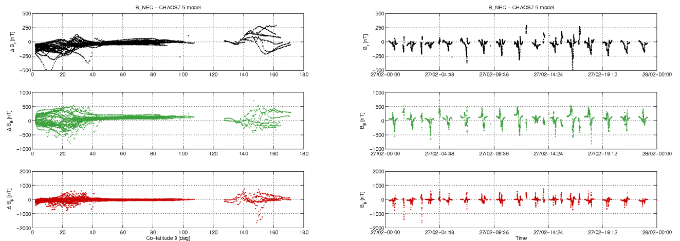
Figure 3-11: S/C B day 27/02: time series of B_{NEC} - B_{Chaos} residuals (right) and B_{NEC} - B_{Chaos} vs colatitude (left).
