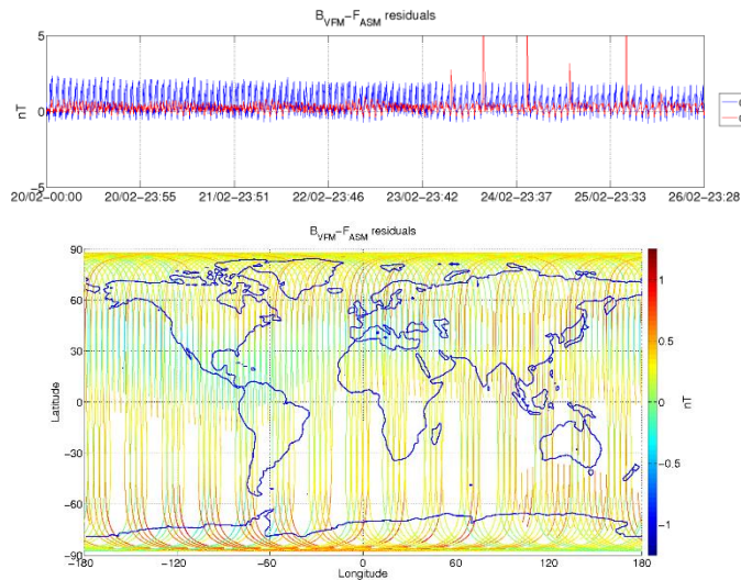
Figure 3-6: ASM-VFM residuals for S/C B, during monitoring period 20/02-26/02. In top figure are plotted: difference between |B_{VFM}| and F_{ASM} (without dB_{Sun} correction) (blue colour), and the residuals with dB_{Sun} corrections (red colour). In bottom figure residuals are presented on the world map.
