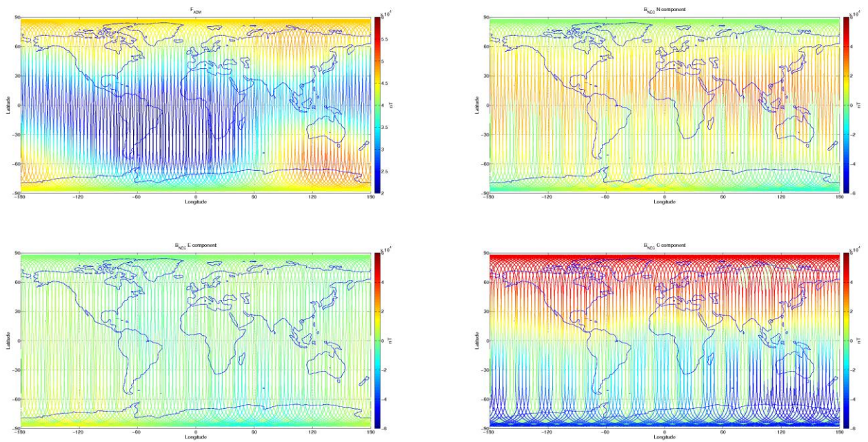
Figure 3-8: S/C B, world map plots of the geomagnetic field and components measured during monitoring period 20/02-26/02. From top to bottom: F-magnetic field from ASM measurement, B_{NEC} components (North, East, and Centre) of magnetic field from VFM measurement.
