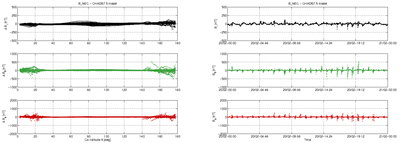
Figure 3-10: S/C A day 20/02: time series of B_{NEC} - B_{Chaos} residuals (right) and B_{NEC} - B_{Chaos} vs colatitude (left).
