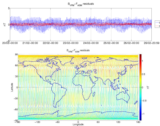
Figure 3-5: ASM-VFM residuals for S/C A, during monitoring period 20/02-26/02. In top figure are plotted: difference between |B_{VFM}| and F_{ASM} (without dB_{Sun} correction) (blue colour), and the residuals with dB_{Sun} corrections (red colour). In bottom figure residuals are presented on the world map.
