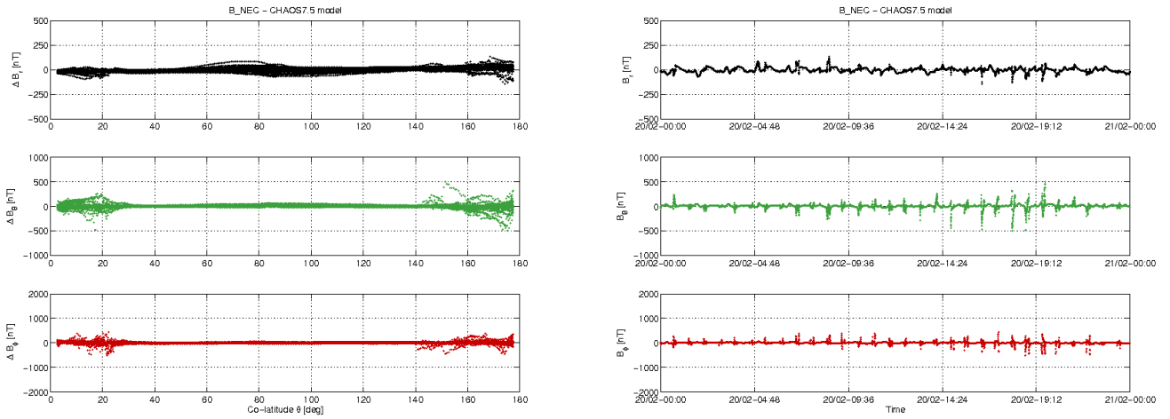
Figure 3-12: S/C C day 20/02: time series of B_{NEC} - B_{Chaos} residuals (right) and B_{NEC} - B_{Chaos} vs colatitude (left)
