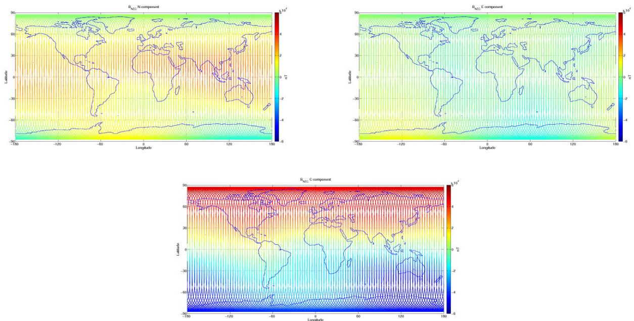
Figure 3-9: S/C C, world map plots of the geomagnetic field and components measured during monitoring period 20/02-26/02. From top to bottom: B_{NEC} components (North, East, and Centre) of magnetic field from VFM measurement.
