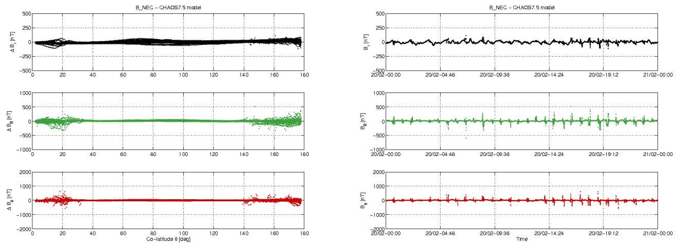
Figure 3-11: S/C B day 20/02: time series of B_{NEC} - B_{Chaos} residuals (right) and B_{NEC} - B_{Chaos} vs colatitude (left).
