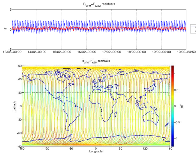
Figure 3-6: ASM-VFM residuals for S/C B, during monitoring period 13/02-19/02. In top figure are plotted: difference between |B_{VFM}| and F_{ASM} (without dB_{Sun} correction) (blue colour), and the residuals with dB_{Sun} corrections (red colour). In bottom figure residuals are presented on the world map.
