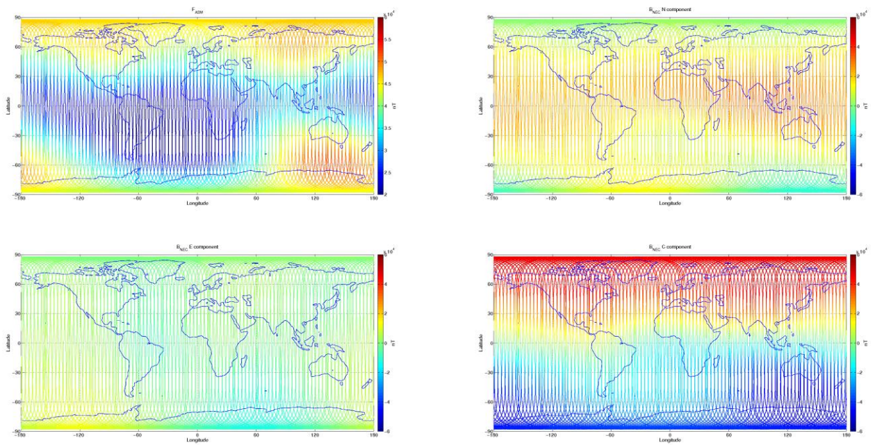
Figure 3-8: S/C B, world map plots of the geomagnetic field and components measured during monitoring period 13/02-19/02. From top to bottom: F-magnetic field from ASM measurement, B_{NEC} components (North, East, and Centre) of magnetic field from VFM measurement.
