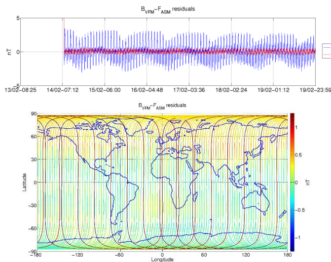
Figure 3-5: ASM-VFM residuals for S/C A, during monitoring period 13/02-19/02. In top figure are plotted: difference between |B_{VFM}| and F_{ASM} (without dB_{Sun} correction) (blue colour), and the residuals with dB_{Sun} corrections (red colour). In bottom figure residuals are presented on the world map.
