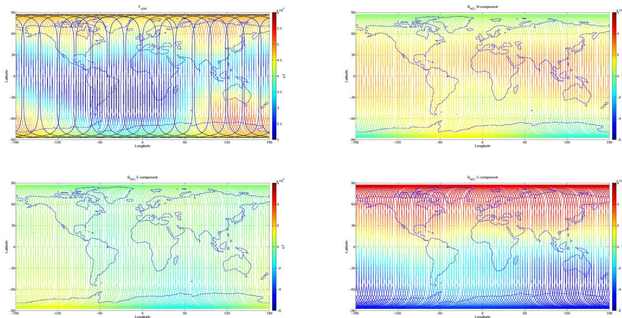
Figure 3-7: S/C A, world map plots of the geomagnetic field and components measured during monitoring period 13/02-19/02. From top to bottom: F-magnetic field from ASM measurement, B_{NEC} components (North, East, and Centre) of magnetic field from VFM measurement.
