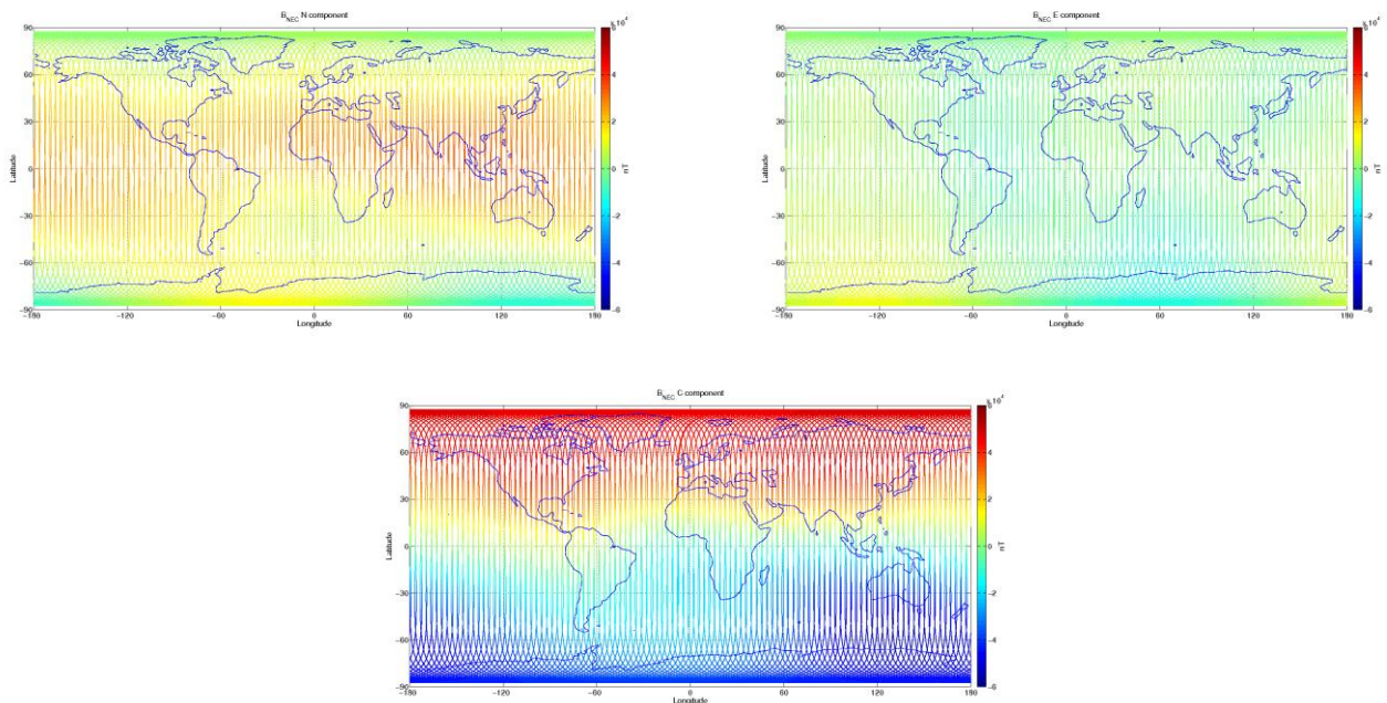
Figure 3-9: S/C C, world map plots of the geomagnetic field and components measured during monitoring period 13/02-19/02. From top to bottom: B_{NEC} components (North, East, and Centre) of magnetic field from VFM measurement.
