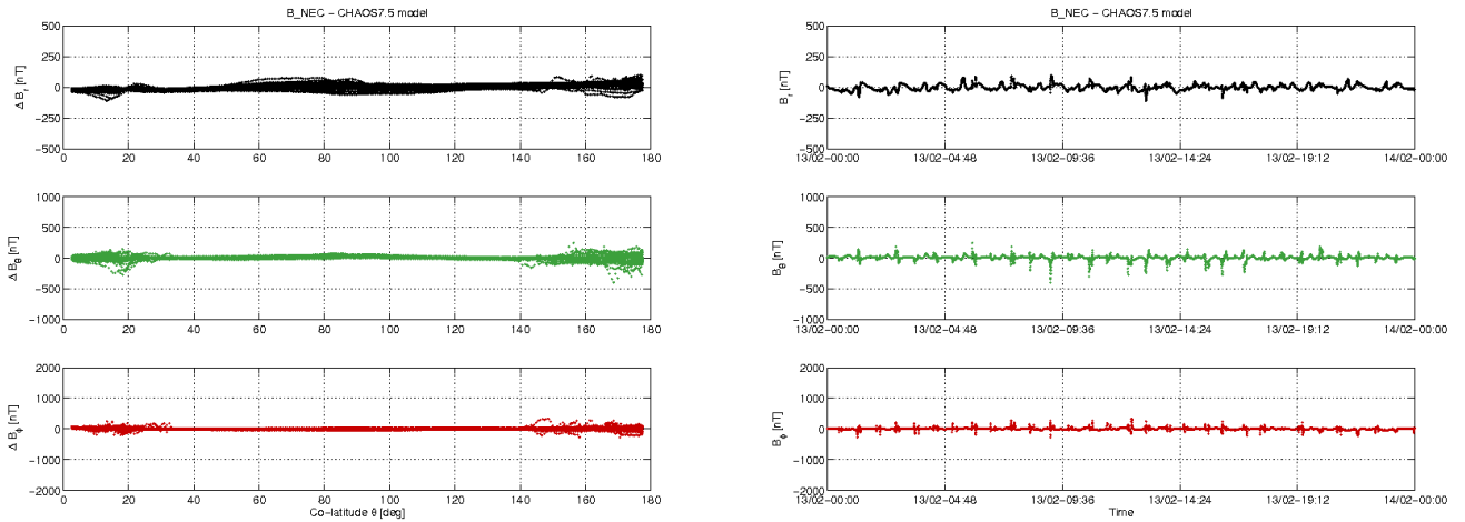
Figure 3-12: S/C C day 13/02: time series of B_{NEC} - B_{Chaos} residuals (right) and B_{NEC} - B_{Chaos} vs colatitude (left)
