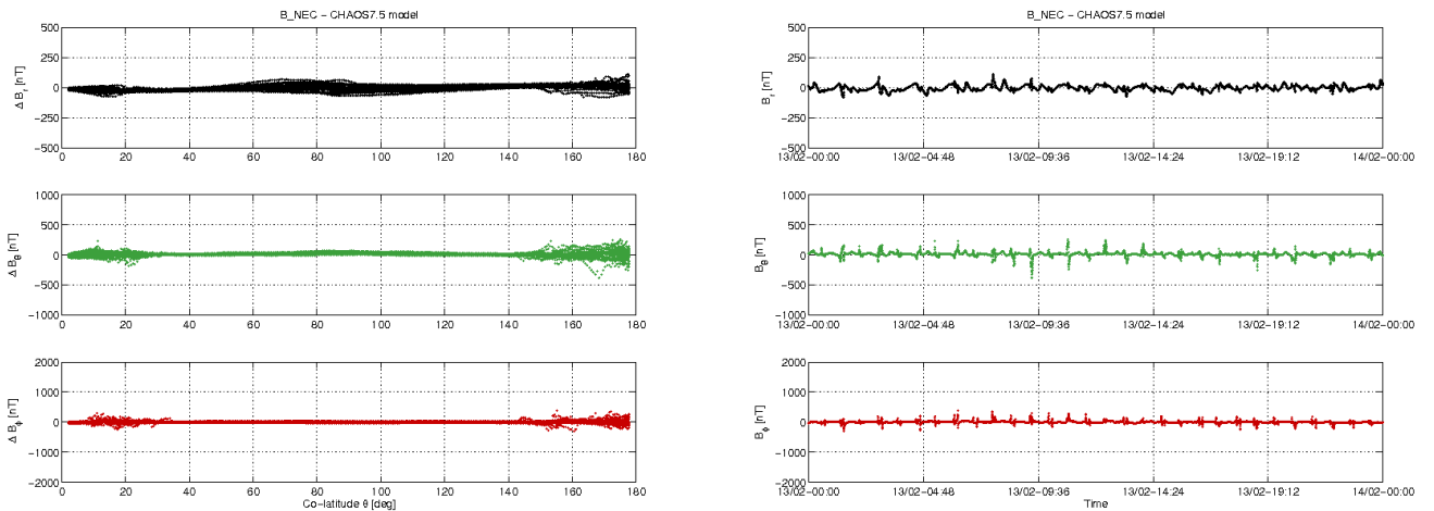
Figure 3-11: S/C B day 13/02: time series of B_{NEC} - B_{Chaos} residuals (right) and B_{NEC} - B_{Chaos} vs colatitude (left).
