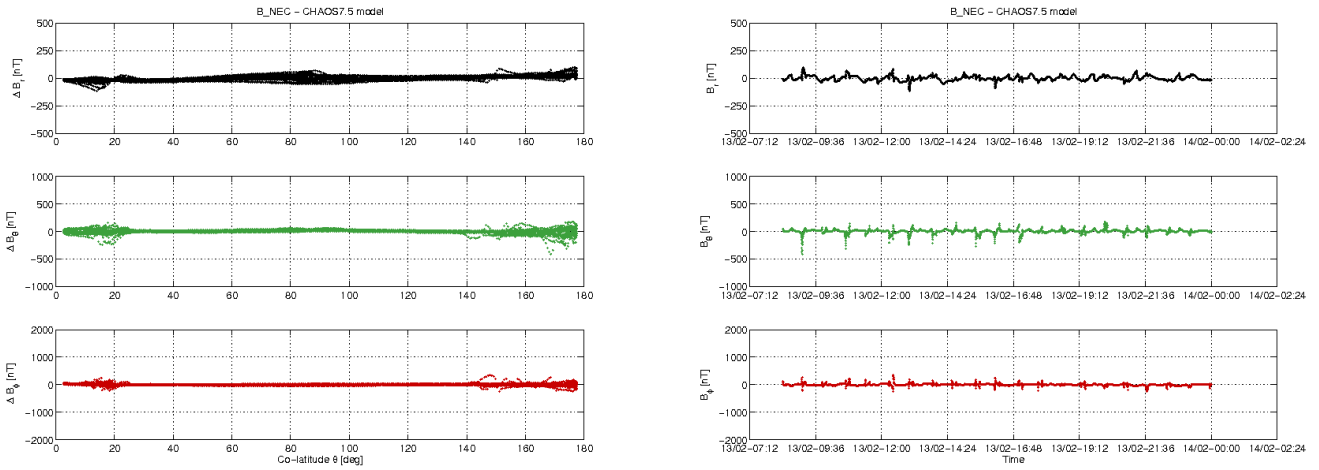
Figure 3-10: S/C A day 13/02: time series of B_{NEC} - B_{Chaos} residuals (right) and B_{NEC} - B_{Chaos} vs colatitude (left).
