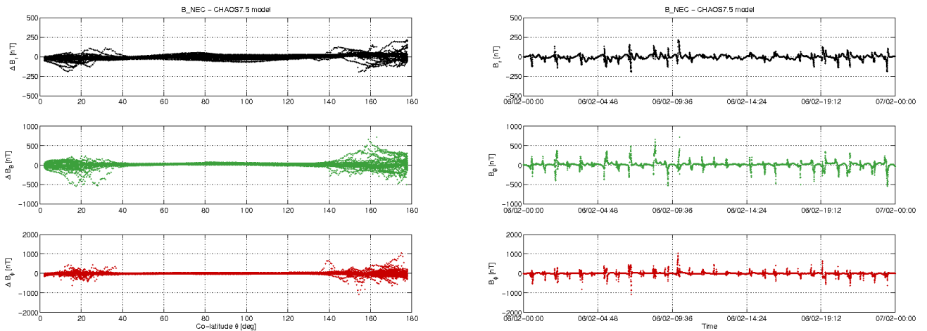
Figure 3-11: S/C B day 06/02: time series of B_{NEC} - B_{Chaos} residuals (right) and B_{NEC} - B_{Chaos} vs colatitude (left).
