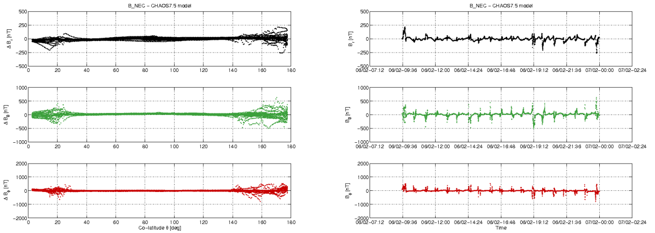
Figure 3-10: S/C A day 06/02: time series of B_{NEC} - B_{Chaos} residuals (right) and B_{NEC} - B_{Chaos} vs colatitude (left).
