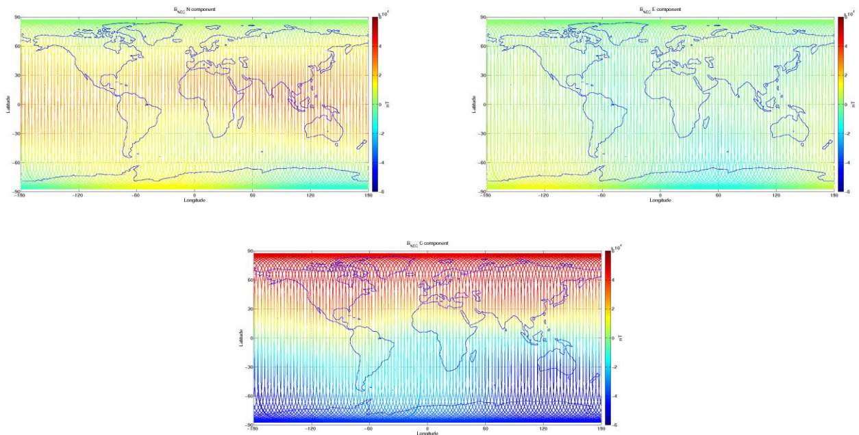
Figure 3-9: S/C C, world map plots of the geomagnetic field and components measured during monitoring period 06/02-12/02. From top to bottom: B_{NEC} components (North, East, and Centre) of magnetic field from VFM measurement.
