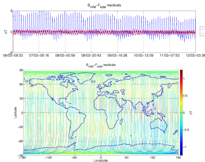
Figure 3-5: ASM-VFM residuals for S/C A, during monitoring period 06/02-12/02. In top figure are plotted: difference between |B_{VFM}| and F_{ASM} (without dB_Sun correction) (blue colour), and the residuals with dB_Sun corrections (red colour). In bottom figure residuals are presented on the world map.
