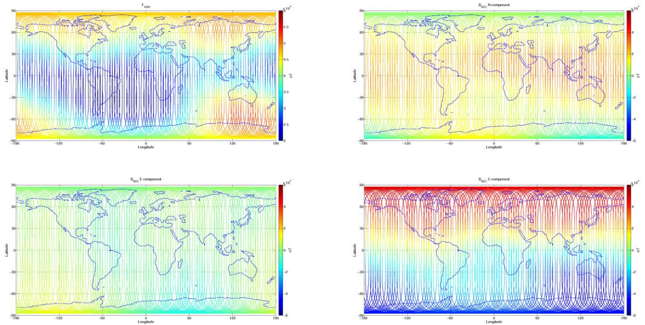
Figure 3-7: S/C A, world map plots of the geomagnetic field and components measured during monitoring period 06/02-12/02. From top to bottom: F-magnetic field from ASM measurement, B_{NEC} components (North, East, and Centre) of magnetic field from VFM measurement.
