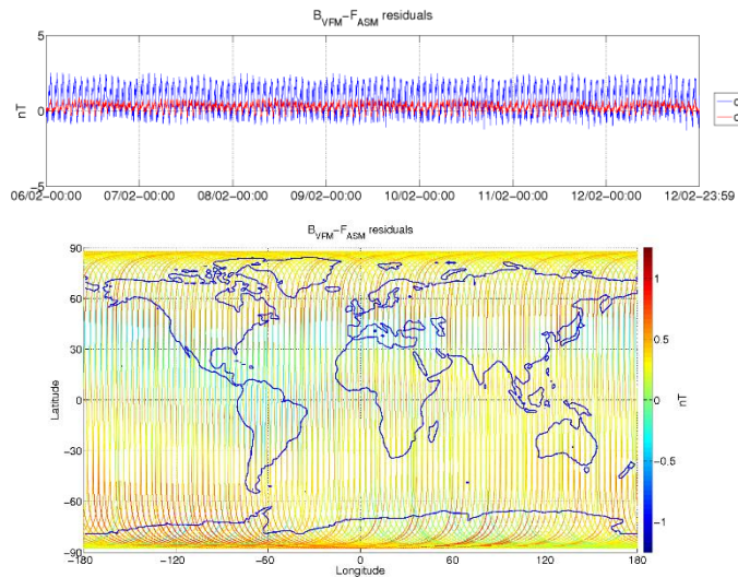
Figure 3-6: ASM-VFM residuals for S/C B, during monitoring period 06/02-12/02. In top figure are plotted: difference between |B_{VFM}| and F_{ASM} (without dB_{Sun} correction) (blue colour), and the residuals with dB_{Sun} corrections (red colour). In bottom figure residuals are presented on the world map.
