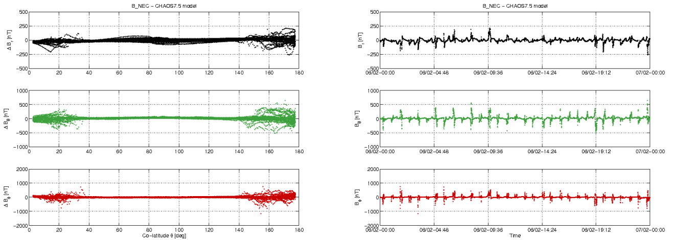
Figure 3-12: S/C C day 06/02: time series of B_{NEC} - B_{Chaos} residuals (right) and B_{NEC} - B_{Chaos} vs colatitude (left)
