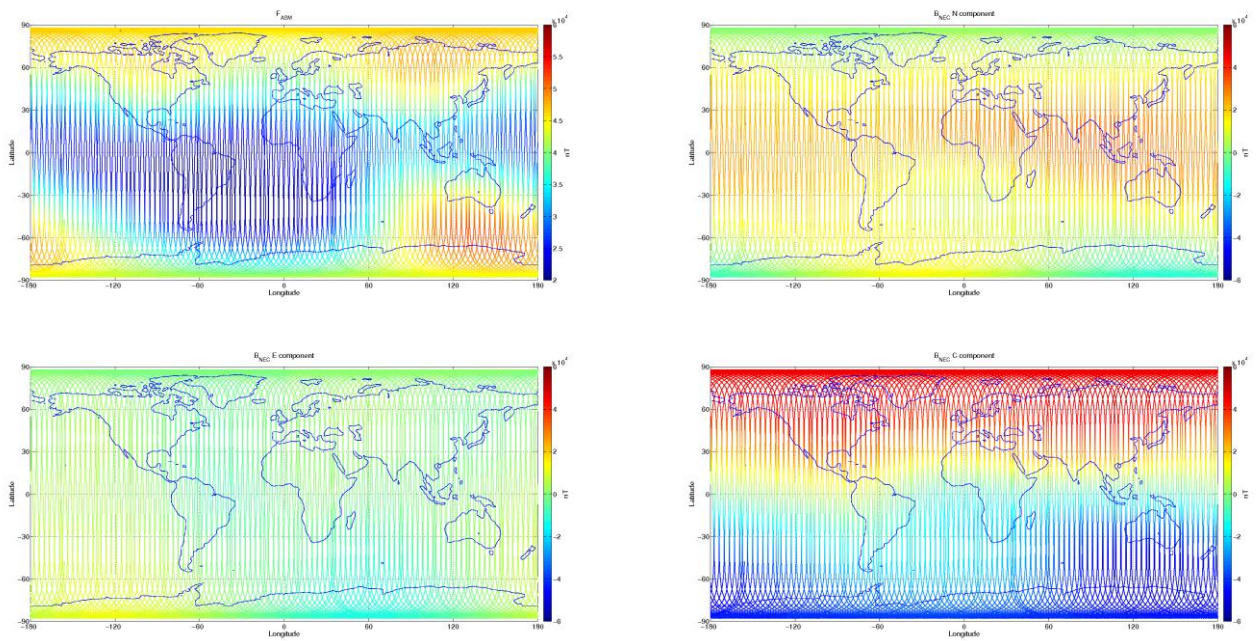
Figure 3-8: S/C B, world map plots of the geomagnetic field and components measured during monitoring period 06/02-12/02. From top to bottom: F-magnetic field from ASM measurement, B_{NEC} components (North, East, and Centre) of magnetic field from VFM measurement.
