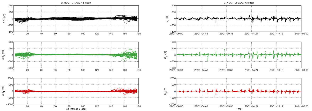
Figure 3-12: S/C C day 23/01: time series of B_{NEC} - B_{Chaos} residuals (right) and B_{NEC} - B_{Chaos} vs colatitude (left)
