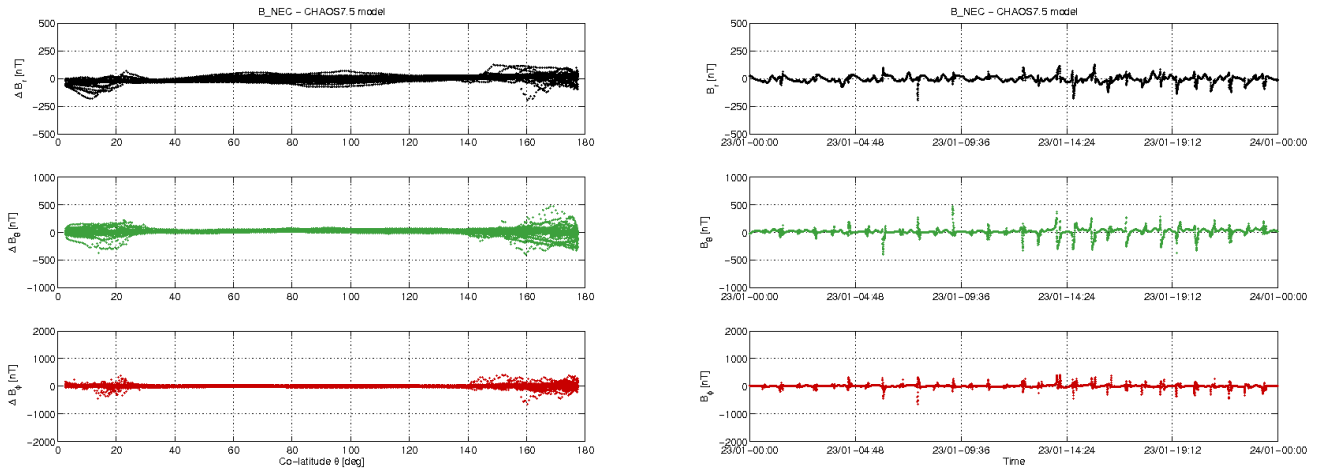
Figure 3-10: S/C A day 23/01: time series of B_{NEC} - B_{Chaos} residuals (right) and B_{NEC} - B_{Chaos} vs colatitude (left).
