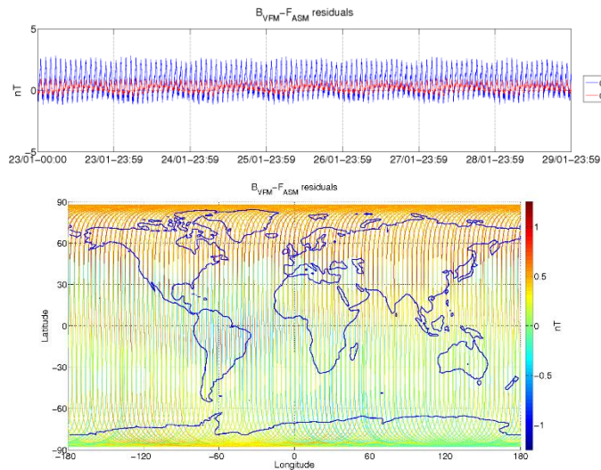
Figure 3-6: ASM-VFM residuals for S/C B, during monitoring period 23/01-29/01. In top figure are plotted: difference between |B_{VFM}| and F_{ASM} (without dB_{Sun} correction) (blue colour), and the residuals with dB_{Sun} corrections (red colour). In bottom figure residuals are presented on the world map.
