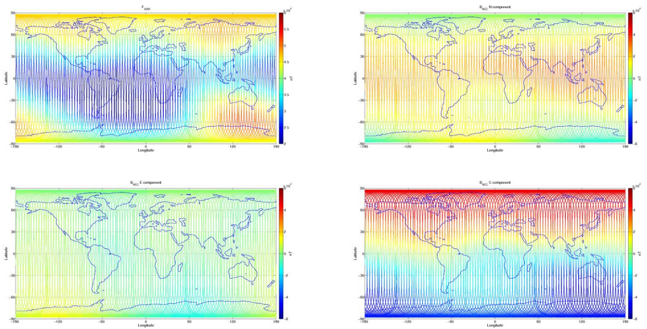
Figure 3-8: S/C B, world map plots of the geomagnetic field and components measured during monitoring period 23/01-29/01. From top to bottom: F-magnetic field from ASM measurement, B_{NEC} components (North, East, and Centre) of magnetic field from VFM measurement.
