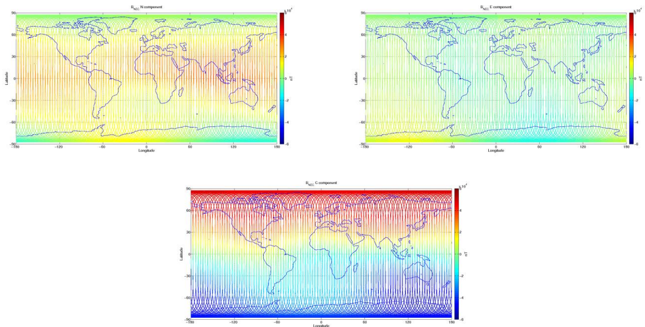
Figure 3-9: S/C C, world map plots of the geomagnetic field and components measured during monitoring period 23/01-29/01. From top to bottom: B_{NEC} components (North, East, and Centre) of magnetic field from VFM measurement.
