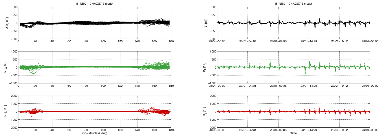
Figure 3-11: S/C B day 23/01: time series of B_{NEC} - B_{Chaos} residuals (right) and B_{NEC} - B_{Chaos} vs colatitude (left).
