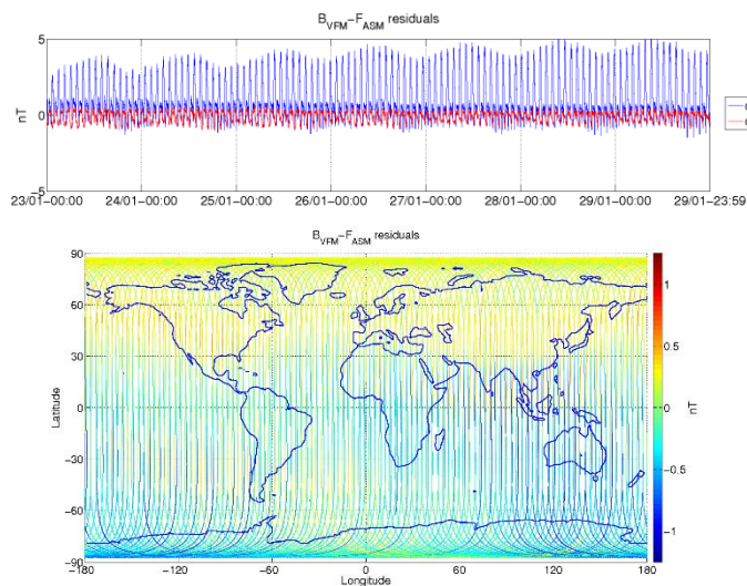
Figure 3-5: ASM-VFM residuals for S/C A, during monitoring period 23/01-29/01. In top figure are plotted: difference between |B_{VFM}| and F_{ASM} (without dB_{Sun} correction) (blue colour), and the residuals with dB_{Sun} corrections (red colour). In bottom figure residuals are presented on the world map.
