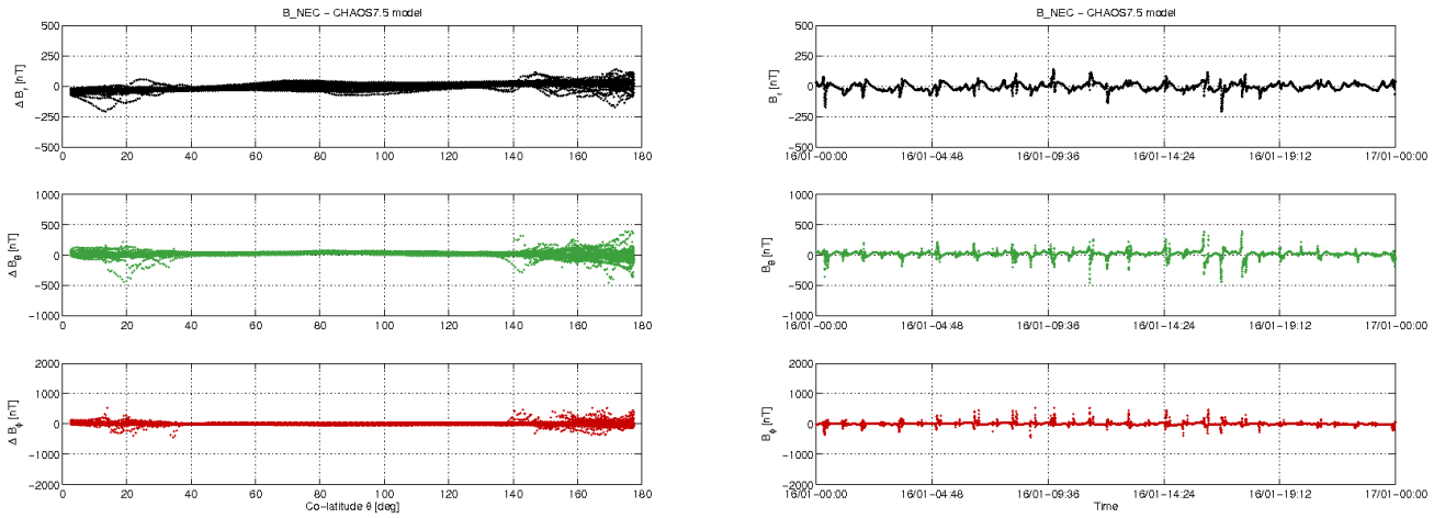
Figure 3-12: S/C C day 16/01: time series of B_{NEC} - B_{Chaos} residuals (right) and B_{NEC} - B_{Chaos} vs colatitude (left)
