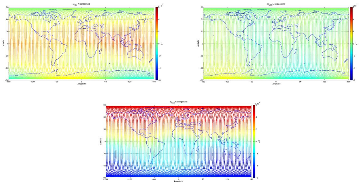
Figure 3-9: S/C C, world map plots of the geomagnetic field and components measured during monitoring period 16/01-22/01. From top to bottom: B_{NEC} components (North, East, and Centre) of magnetic field from VFM measurement.
