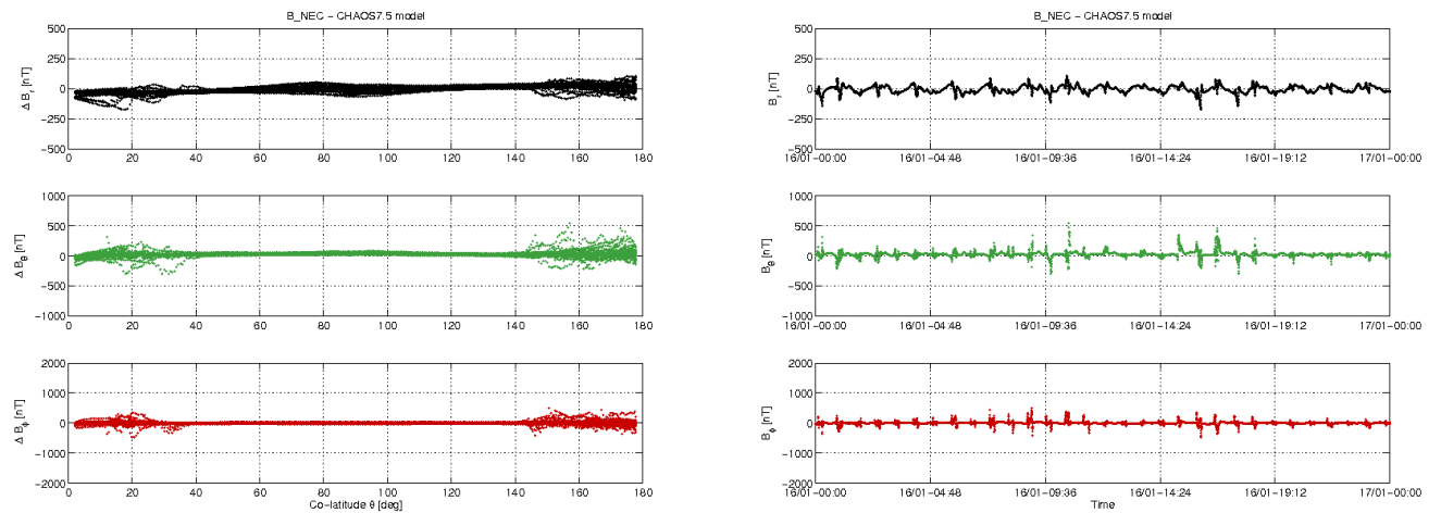
Figure 3-11: S/C B day 16/01: time series of B_{NEC} - B_{Chaos} residuals (right) and B_{NEC} - B_{Chaos} vs colatitude (left).
