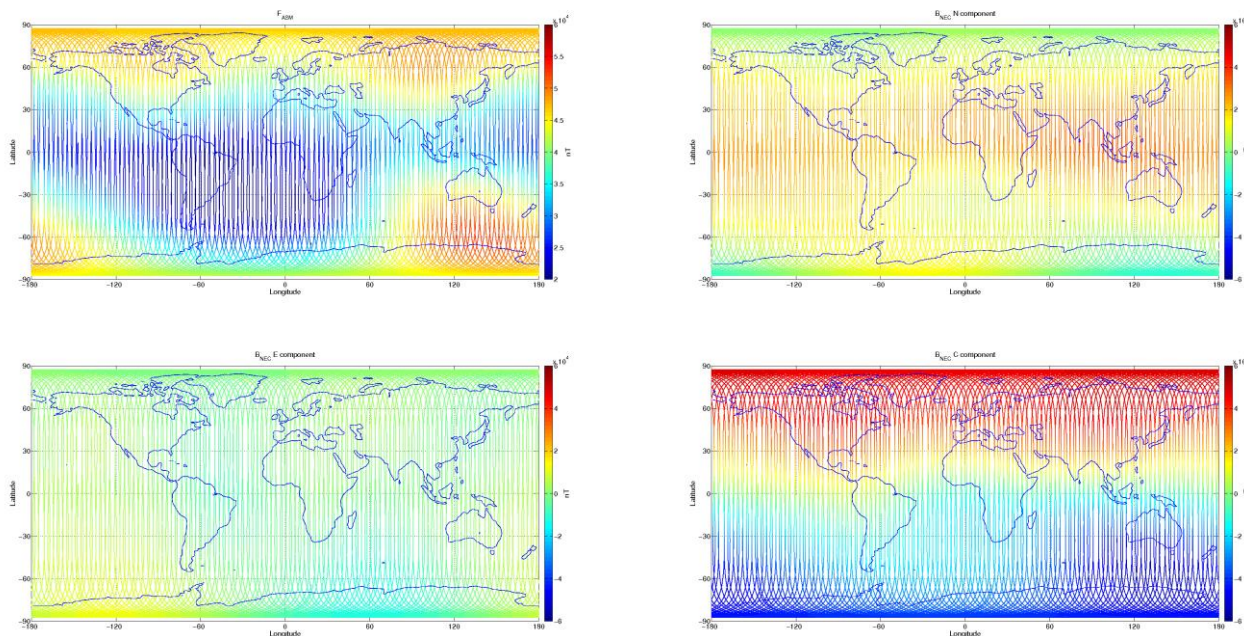
Figure 3-7: S/C A, world map plots of the geomagnetic field and components measured during monitoring period 16/01-22/01. From top to bottom: F-magnetic field from ASM measurement, B_{NEC} components (North, East, and Centre) of magnetic field from VFM measurement.
