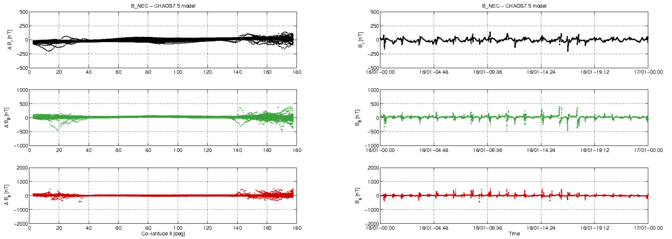
Figure 3-10: S/C A day 16/01: time series of B_{NEC} - B_{Chaos} residuals (right) and B_{NEC} - B_{Chaos} vs colatitude (left).
