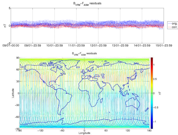
Figure 3-5: ASM-VFM residuals for S/C A, during monitoring period 09/01-15/01. In top figure are plotted: difference between |B_{VFM}| and F_{ASM} (without dB_{Sun} correction) (blue colour), and the residuals with dB_{Sun} corrections (red colour). In bottom figure residuals are presented on the world map.
