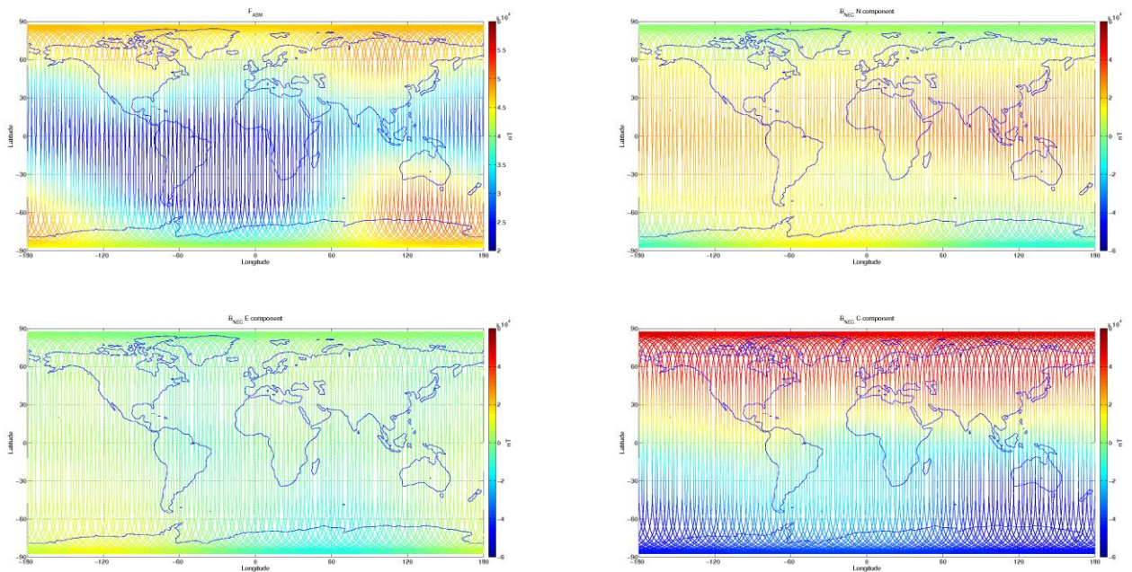
Figure 3-7: S/C A, world map plots of the geomagnetic field and components measured during monitoring period 09/01-15/01. From top to bottom: F-magnetic field from ASM measurement, B_{NEC} components (North, East, and Centre) of magnetic field from VFM measurement.
