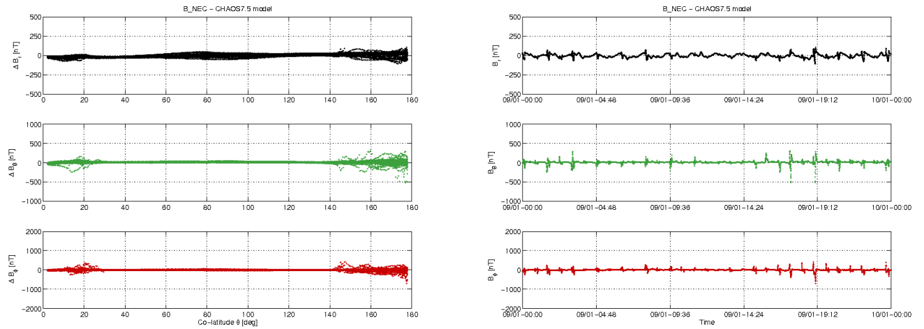
Figure 3-11: S/C B day 09/01: time series of B_{NEC} - B_{Chaos} residuals (right) and B_{NEC} - B_{Chaos} vs colatitude (left).
