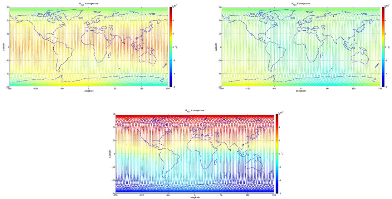
Figure 3-9: S/C C, world map plots of the geomagnetic field and components measured during monitoring period 09/01-15/01. From top to bottom: B_{NEC} components (North, East, and Centre) of magnetic field from VFM measurement.
