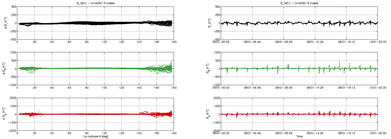
Figure 3-12: S/C C day 09/01: time series of B_{NEC} - B_{Chaos} residuals (right) and B_{NEC} - B_{Chaos} vs colatitude (left)
