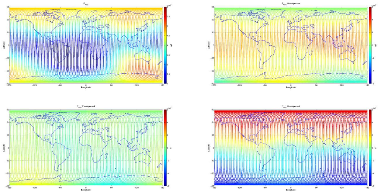
Figure 3-8: S/C B, world map plots of the geomagnetic field and components measured during monitoring period 09/01-15/01. From top to bottom: F-magnetic field from ASM measurement, B_{\text{NEC}} components (North, East, and Centre) of magnetic field from VFM measurement.
