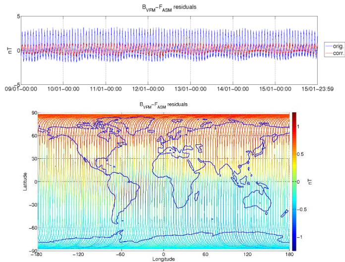
Figure 3-6: ASM-VFM residuals for S/C B, during monitoring period 09/01-15/01. In top figure are plotted: difference between |B_{VFM}| and F_{ASM} (without dB_{Sun} correction) (blue colour), and the residuals with dB_{Sun} corrections (red colour). In bottom figure residuals are presented on the world map.
