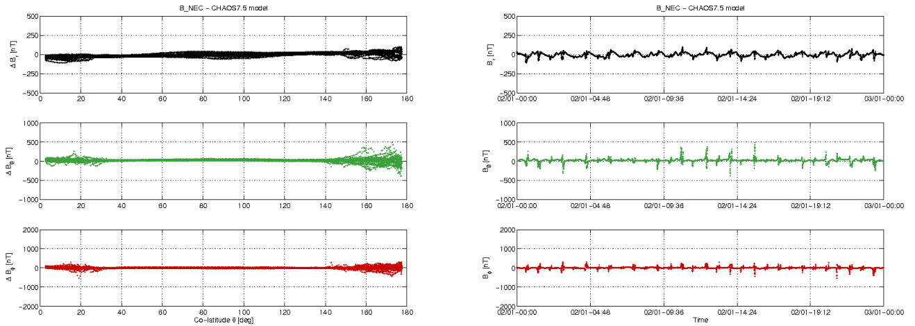
Figure 3-12: S/C C day 02/01: time series of B_{NEC} - B_{Chaos} residuals (right) and B_{NEC} - B_{Chaos} vs colatitude (left)
