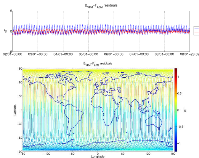
Figure 3-5: ASM-VFM residuals for S/C A, during monitoring period 02/01-08/01. In top figure are plotted: difference between |B_{VFM}| and F_{ASM} (without dB_{Sun} correction) (blue colour), and the residuals with dB_{Sun} corrections (red colour). In bottom figure residuals are presented on the world map.
