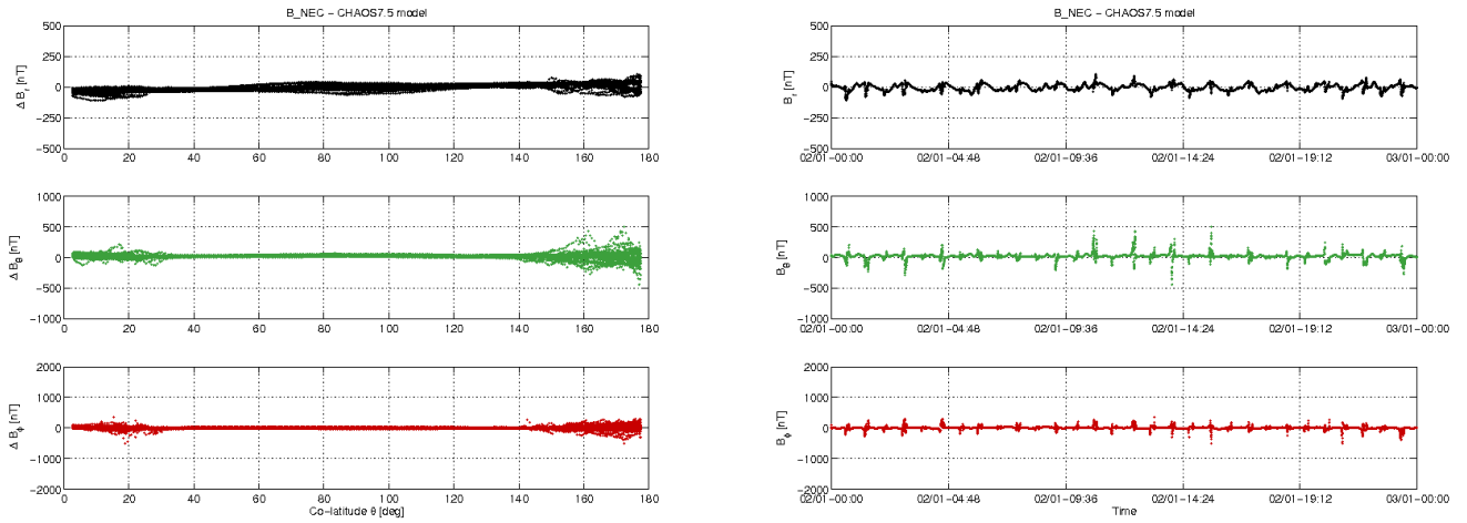
Figure 3-10: S/C A day 02/01: time series of B_{NEC} - B_{Chaos} residuals (right) and B_{NEC} - B_{Chaos} vs colatitude (left).
