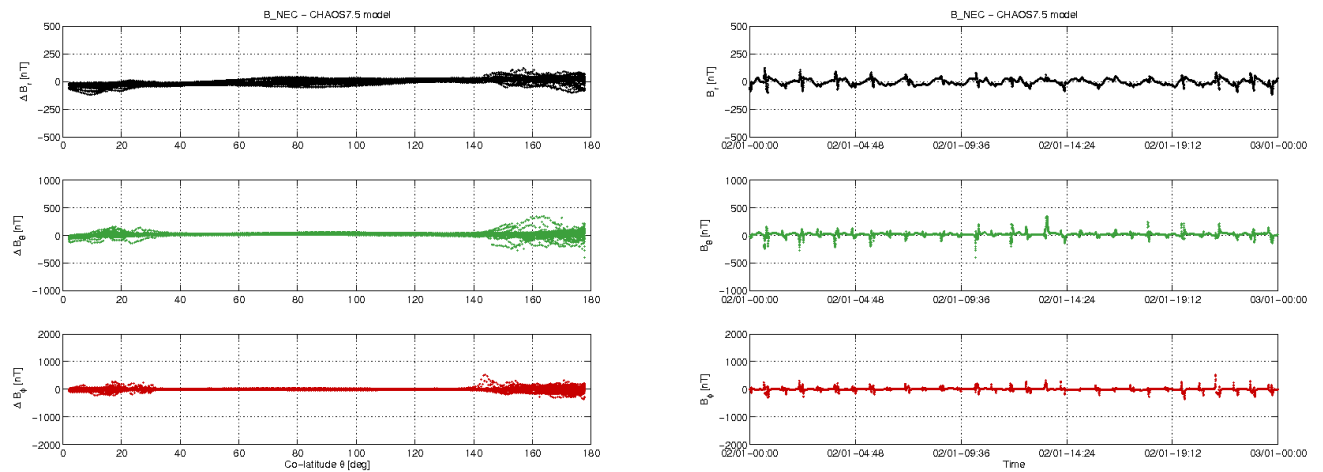
Figure 3-11: S/C B day 02/01: time series of B_{NEC} - B_{Chaos} residuals (right) and B_{NEC} - B_{Chaos} vs colatitude (left).
