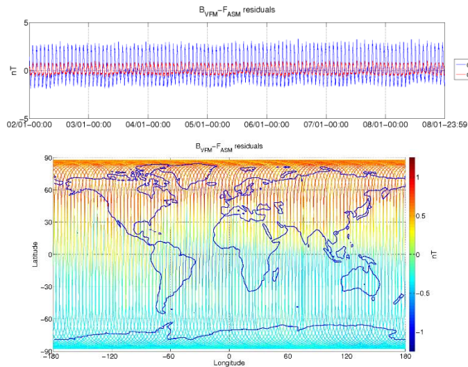
Figure 3-6: ASM-VFM residuals for S/C B, during monitoring period 02/01-08/01. In top figure are plotted: difference between |B_{VFM}| and F_{ASM} (without dB_{Sun} correction) (blue colour), and the residuals with dB_{Sun} corrections (red colour). In bottom figure residuals are presented on the world map.
