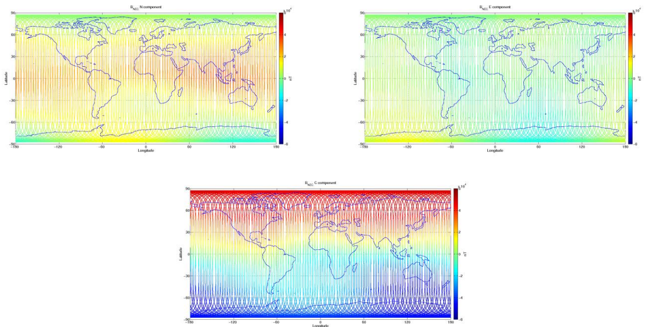
Figure 3-9: S/C C, world map plots of the geomagnetic field and components measured during monitoring period 02/01-08/01. From top to bottom: B_{NEC} components (North, East, and Centre) of magnetic field from VFM measurement.
