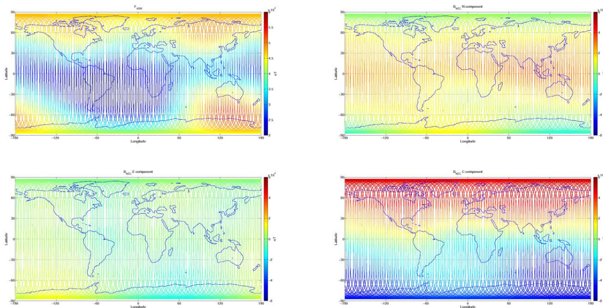
Figure 3-7: S/C A, world map plots of the geomagnetic field and components measured during monitoring period 02/01-08/01. From top to bottom: F-magnetic field from ASM measurement, B_{NEC} components (North, East, and Centre) of magnetic field from VFM measurement.
