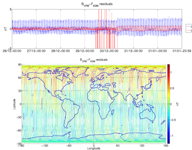
Figure 3-6: ASM-VFM residuals for S/C B, during monitoring period 26/12-01/01. In top figure are plotted: difference between |B_{VFM}| and F_{ASM} (without dB_{Sun} correction) (blue colour), and the residuals with dB_{Sun} corrections (red colour). In bottom figure residuals are presented on the world map.
