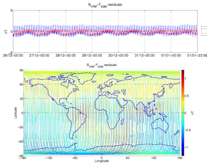
Figure 3-5: ASM-VFM residuals for S/C A, during monitoring period 26/12-01/01. In top figure are plotted: difference between |B_{VFM}| and F_{ASM} (without dB_{Sun} correction) (blue colour), and the residuals with dB_{Sun} corrections (red colour). In bottom figure residuals are presented on the world map.
