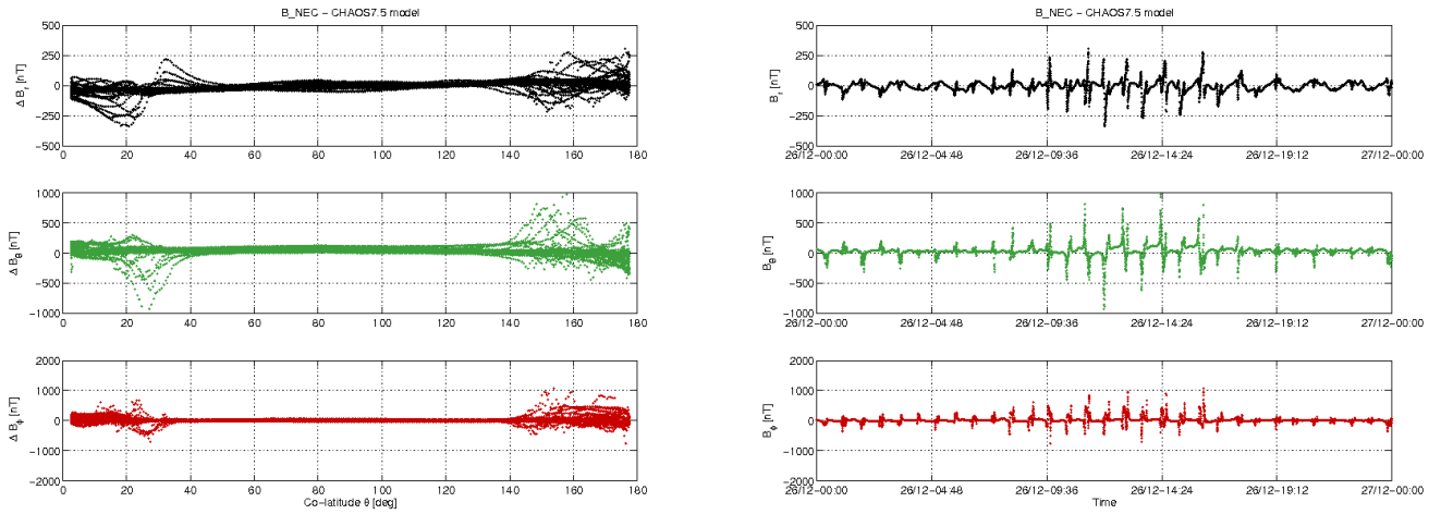
Figure 3-10: S/C A day 26/12: time series of B_{NEC} - B_{Chaos} residuals (right) and B_{NEC} - B_{Chaos} vs colatitude (left).
