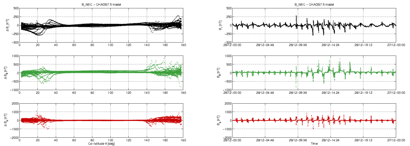
Figure 3-11: S/C B day 26/12: time series of B_{NEC} - B_{Chaos} residuals (right) and B_{NEC} - B_{Chaos} vs colatitude (left).
