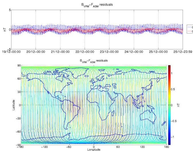
Figure 3-5: ASM-VFM residuals for S/C A, during monitoring period 19/12-25/12. In top figure are plotted: difference between |B_{VFM}| and F_{ASM} (without dB_Sun correction) (blue colour), and the residuals with dB_Sun corrections (red colour). In bottom figure residuals are presented on the world map.
