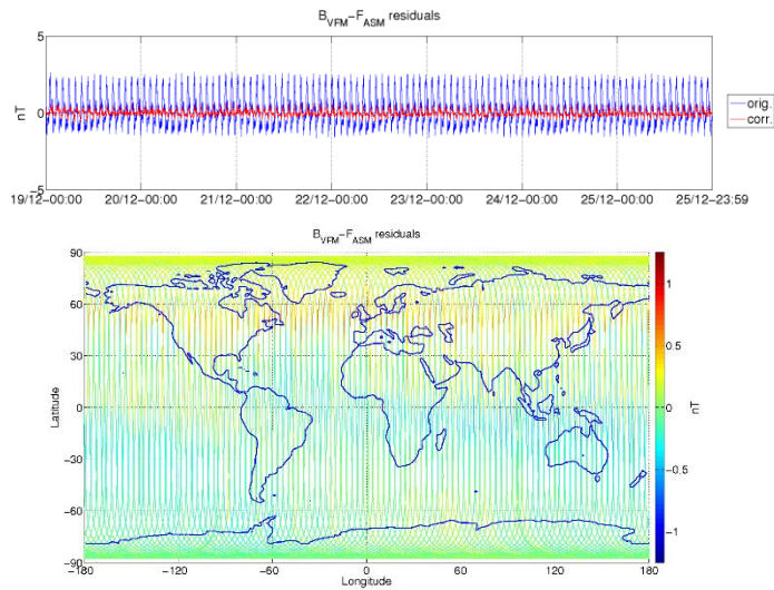
Figure 3-6: ASM-VFM residuals for S/C B, during monitoring period 19/12-25/12. In top figure are plotted: difference between |B_{VFM}| and F_{ASM} (without dB_{Sun} correction) (blue colour), and the residuals with dB_{Sun} corrections (red colour). In bottom figure residuals are presented on the world map.
