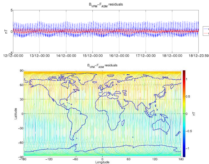
Figure 3-6: ASM-VFM residuals for S/C B, during monitoring period 12/12-18/12. In top figure are plotted: difference between |B_{VFM}| and F_{ASM} (without dB_{Sun} correction) (blue colour), and the residuals with dB_{Sun} corrections (red colour). In bottom figure residuals are presented on the world map.
