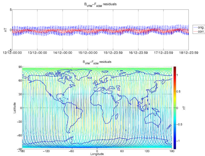
Figure 3-5: ASM-VFM residuals for S/C A, during monitoring period 12/12-18/12. In top figure are plotted: difference between |B_{VFM}| and F_{ASM} (without dB_{Sun} correction) (blue colour), and the residuals with dB_{Sun} corrections (red colour). In bottom figure residuals are presented on the world map.
