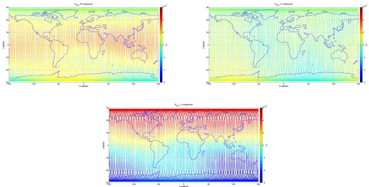
Figure 3-9: S/C C, world map plots of the geomagnetic field and components measured during monitoring period 12/12-18/12. From top to bottom: B_{NEC} components (North, East, and Centre) of magnetic field from VFM measurement.
