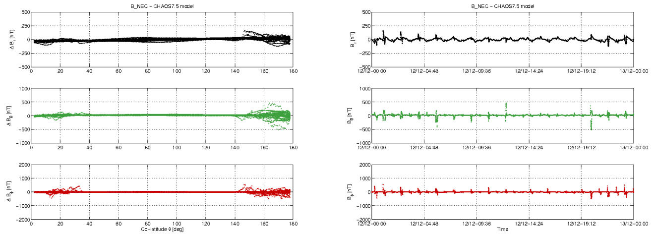
Figure 3-11: S/C B day 12/12: time series of B_{NEC} - B_{Chaos} residuals (right) and B_{NEC} - B_{Chaos} vs colatitude (left).
