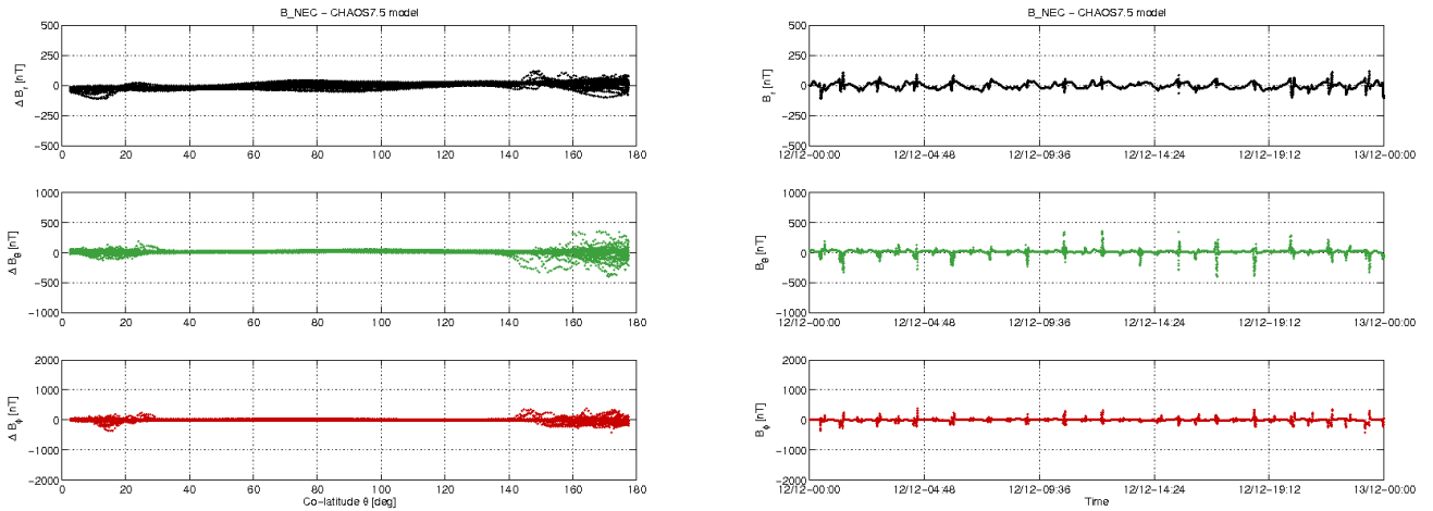
Figure 3-12: S/C C day 12/12: time series of B_{NEG} - B_{Chaos} residuals (right) and B_{NEG} - B_{Chaos} vs colatitude (left)
