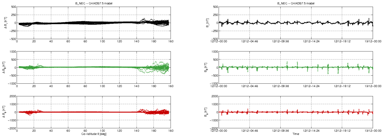
Figure 3-10: S/C A day 12/12: time series of B_{NEC} - B_{Chaos} residuals (right) and B_{NEC} - B_{Chaos} vs colatitude (left).
