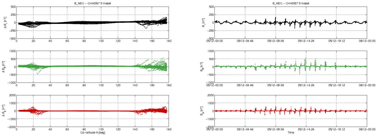
Figure 3-12: S/C C day 05/12: time series of B_{NEC} - B_{Chaos} residuals (right) and B_{NEC} - B_{Chaos} vs colatitude (left)
