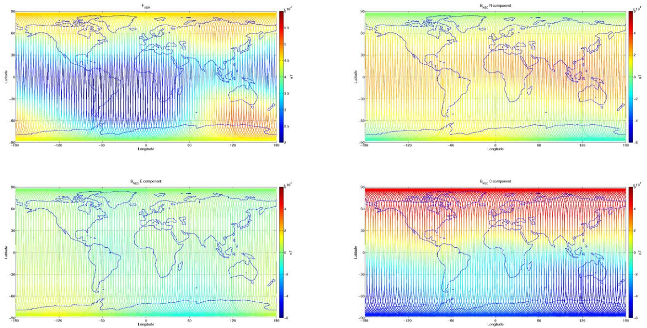
Figure 3-8: S/C B, world map plots of the geomagnetic field and components measured during monitoring period 05/12-11/12. From top to bottom: F-magnetic field from ASM measurement, B_{NEC} components (North, East, and Centre) of magnetic field from VFM measurement.
