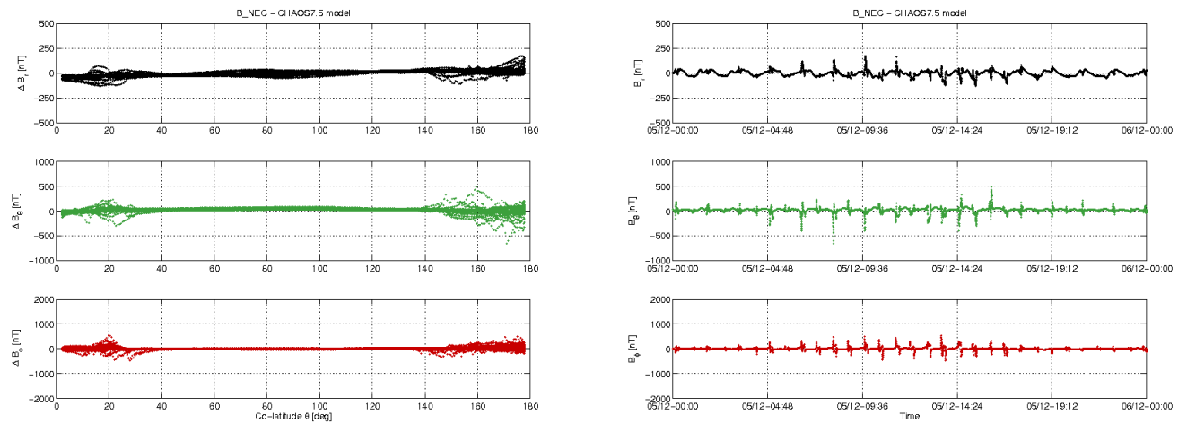
Figure 3-11: S/C B day 05/12: time series of B_{NEC} - B_{Chaos} residuals (right) and B_{NEC} - B_{Chaos} vs colatitude (left).
