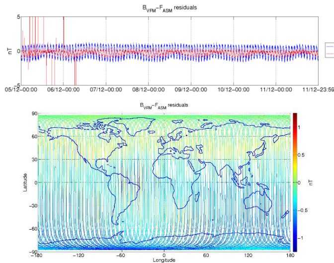
Figure 3-5: ASM-VFM residuals for S/C A, during monitoring period 05/12-11/12. In top figure are plotted: difference between |B_{VFM}| and F_{ASM} (without dB_Sun correction) (blue colour), and the residuals with dB_Sun corrections (red colour). In bottom figure residuals are presented on the world map.
