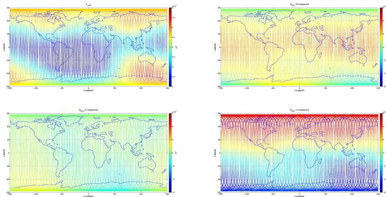
Figure 3-7: S/C A, world map plots of the geomagnetic field and components measured during monitoring period 05/12-11/12. From top to bottom: F-magnetic field from ASM measurement, B_{NEC} components (North, East, and Centre) of magnetic field from VFM measurement.
