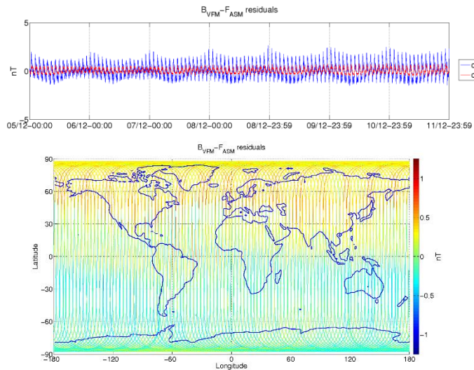
Figure 3-6: ASM-VFM residuals for S/C B, during monitoring period 05/12-11/12. In top figure are plotted: difference between |B_{VFM}| and F_{ASM} (without dB_{Sun} correction) (blue colour), and the residuals with dB_{Sun} corrections (red colour). In bottom figure residuals are presented on the world map.
