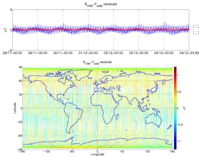
Figure 3-6: ASM-VFM residuals for S/C B, during monitoring period 28/11-04/12. In top figure are plotted: difference between |B_{VFM}| and F_{ASM} (without dB_{Sun} correction) (blue colour), and the residuals with dB_{Sun} corrections (red colour). In bottom figure residuals are presented on the world map.
