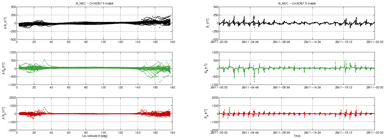
Figure 3-12: S/C C day 28/11: time series of B_{NEC} - B_{Chaos} residuals (right) and B_{NEC} - B_{Chaos} vs colatitude (left)
