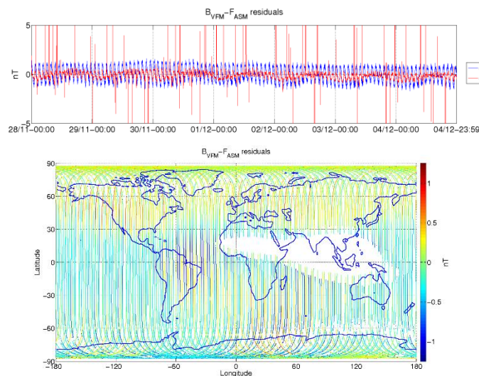
Figure 3-5: ASM-VFM residuals for S/C A, during monitoring period 28/11-04/12. In top figure are plotted: difference between |B_{VFM}| and F_{ASM} (without dB_Sun correction) (blue colour), and the residuals with dB_Sun corrections (red colour). In bottom figure residuals are presented on the world map.
