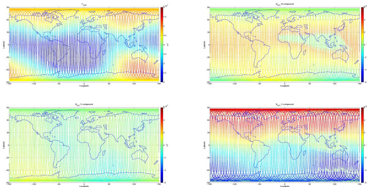
Figure 3-7: S/C A, world map plots of the geomagnetic field and components measured during monitoring period 28/11-04/12. From top to bottom: F-magnetic field from ASM measurement, B_{NEC} components (North, East, and Centre) of magnetic field from VFM measurement.
