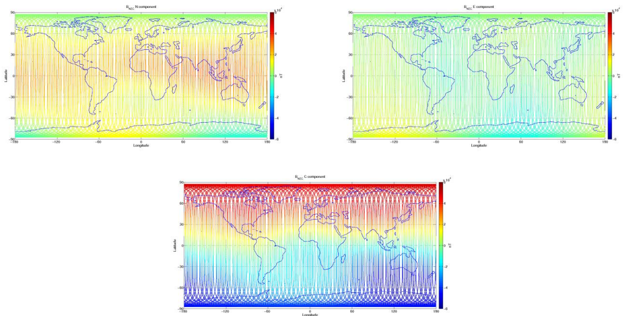
Figure 3-9: S/C C, world map plots of the geomagnetic field and components measured during monitoring period 28/11-04/12. From top to bottom: B_{NEC} components (North, East, and Centre) of magnetic field from VFM measurement.
