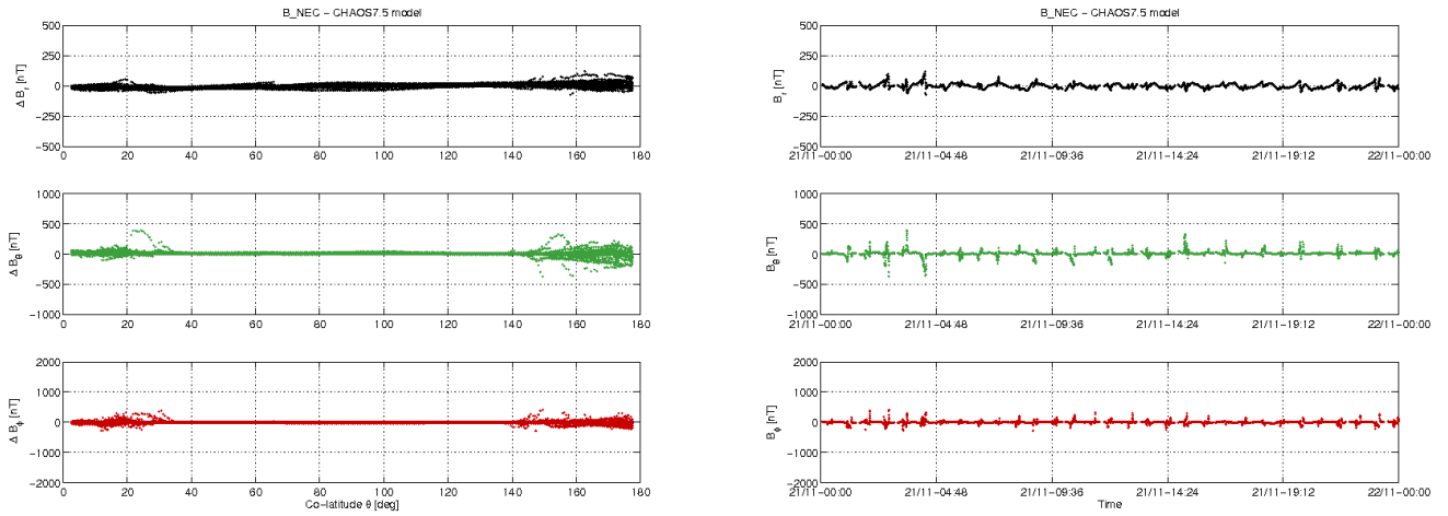
Figure 3-10: S/C A day 21/11: time series of B_{NEC} - B_{Chaos} residuals (right) and B_{NEC} - B_{Chaos} vs colatitude (left).
