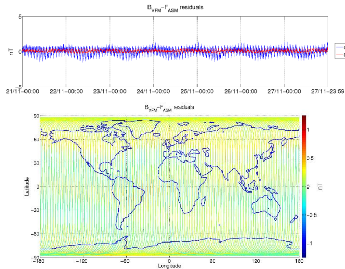
Figure 3-6: ASM-VFM residuals for S/C B, during monitoring period 21/11-27/11. In top figure are plotted: difference between |B_{VFM}| and F_{ASM} (without dB_{Sun} correction) (blue colour), and the residuals with dB_{Sun} corrections (red colour). In bottom figure residuals are presented on the world map.
