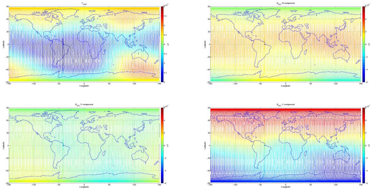
Figure 3-8: S/C B, world map plots of the geomagnetic field and components measured during monitoring period 21/11-27/11. From top to bottom: F-magnetic field from ASM measurement, B_{NEC} components (North, East, and Centre) of magnetic field from VFM measurement.
