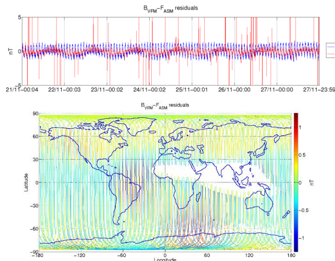
Figure 3-5: ASM-VFM residuals for S/C A, during monitoring period 21/11-27/11. In top figure are plotted: difference between |B_{VFM}| and F_{ASM} (without dB_{Sun} correction) (blue colour), and the residuals with dB_{Sun} corrections (red colour). In bottom figure residuals are presented on the world map.
