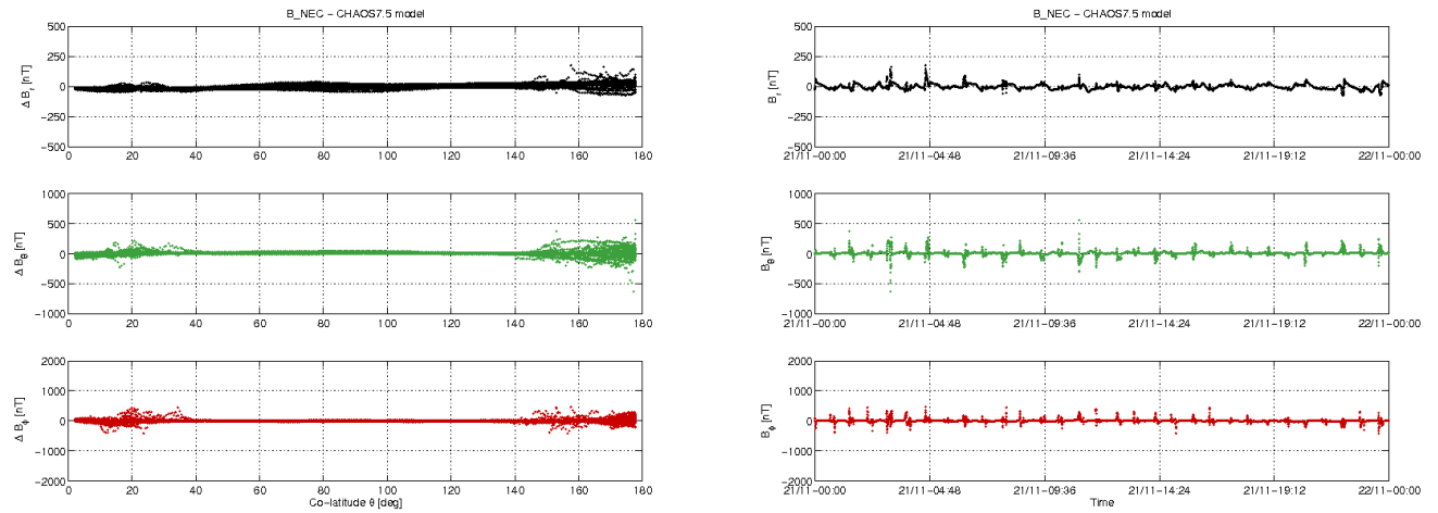
Figure 3-11: S/C B day 21/11: time series of B_{NEC} - B_{Chaos} residuals (right) and B_{NEC} - B_{Chaos} vs colatitude (left).
