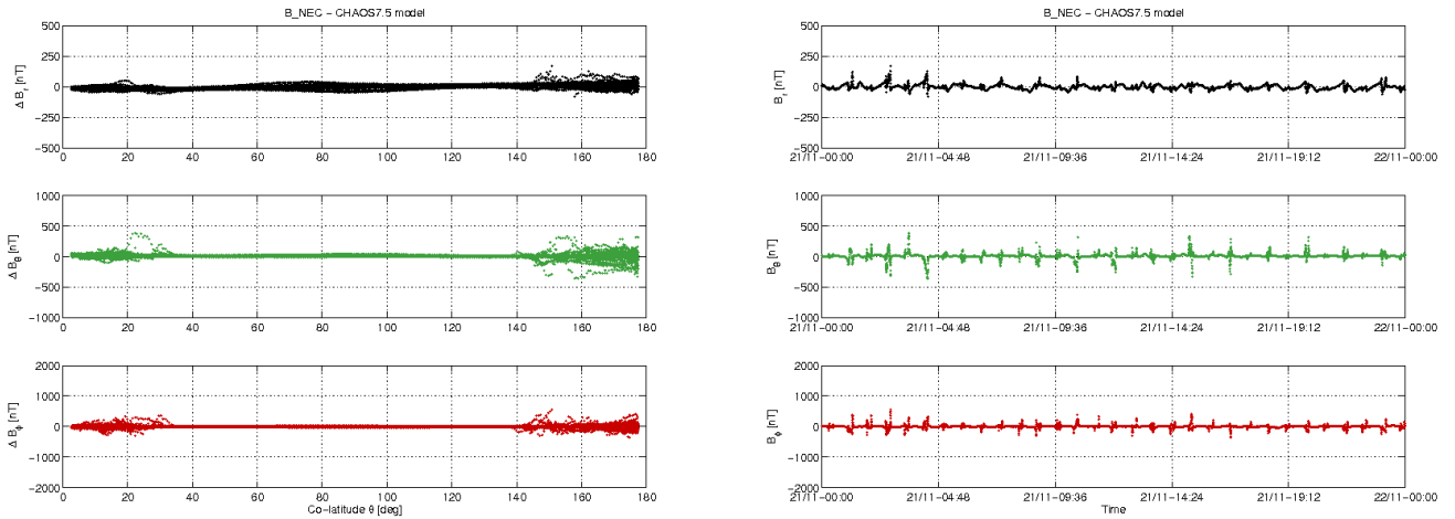
Figure 3-12: S/C C day 21/11: time series of B_{NEC} - B_{Chaos} residuals (right) and B_{NEC} - B_{Chaos} vs colatitude (left)
