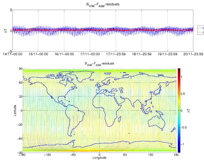
Figure 3-6: ASM-VFM residuals for S/C B, during monitoring period 14/11-20/11. In top figure are plotted: difference between |B_{VFM}| and F_{ASM} (without dB_{Sun} correction) (blue colour), and the residuals with dB_{Sun} corrections (red colour). In bottom figure residuals are presented on the world map.
