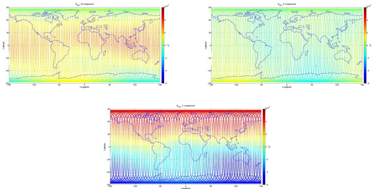
Figure 3-9: S/C C, world map plots of the geomagnetic field and components measured during monitoring period 14/11-20/11. From top to bottom: B_{NEC} components (North, East, and Centre) of magnetic field from VFM measurement.
