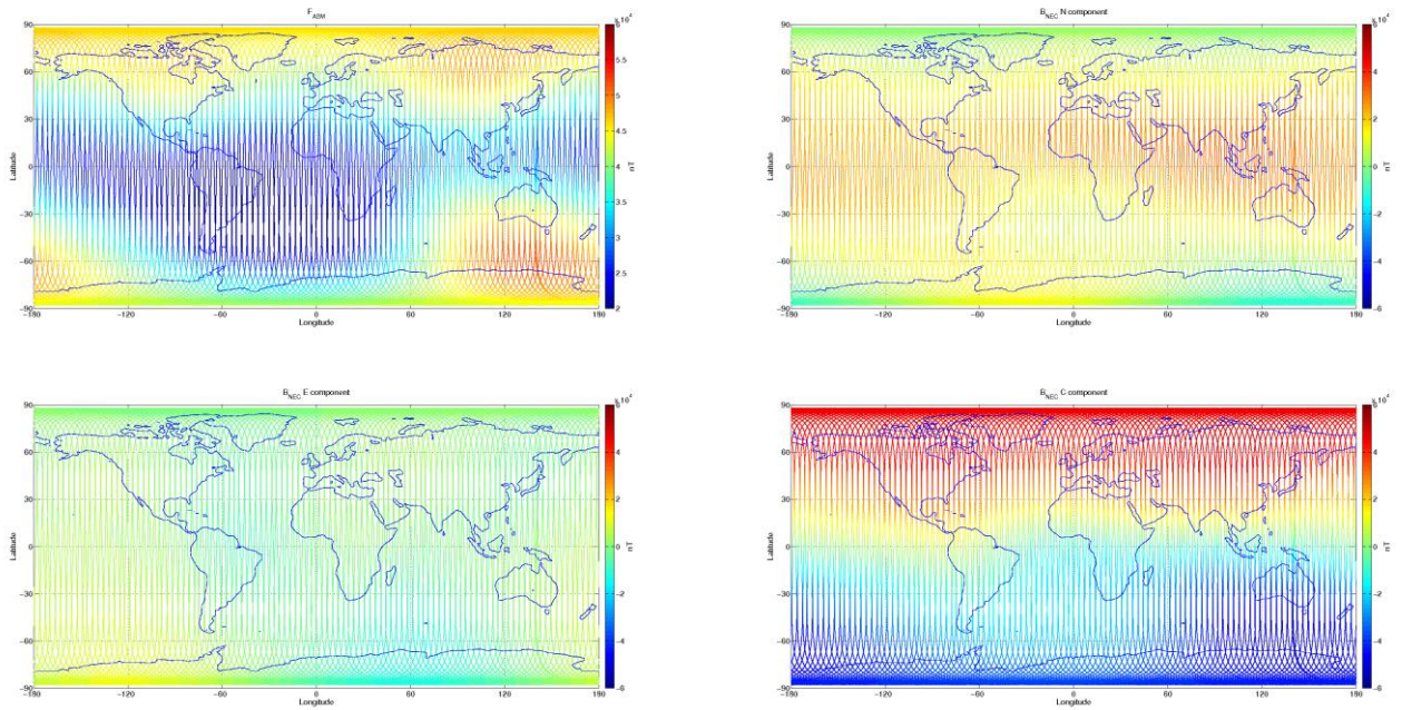
Figure 3-8: S/C B, world map plots of the geomagnetic field and components measured during monitoring period 14/11-20/11. From top to bottom: F-magnetic field from ASM measurement, B_{NEC} components (North, East, and Centre) of magnetic field from VFM measurement.
