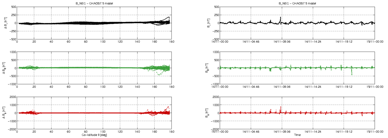
Figure 3-10: S/C A day 14/11: time series of B_{NEC} - B_{Chaos} residuals (right) and B_{NEC} - B_{Chaos} vs colatitude (left).
