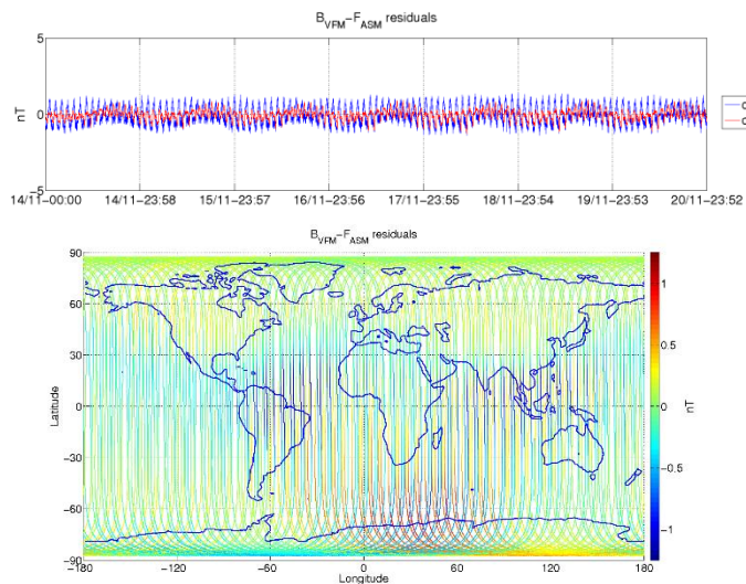
Figure 3-5: ASM-VFM residuals for S/C A, during monitoring period 14/11-20/11. In top figure are plotted: difference between |B_{VFM}| and F_{ASM} (without dB_{Sun} correction) (blue colour), and the residuals with dB_{Sun} corrections (red colour). In bottom figure residuals are presented on the world map.
