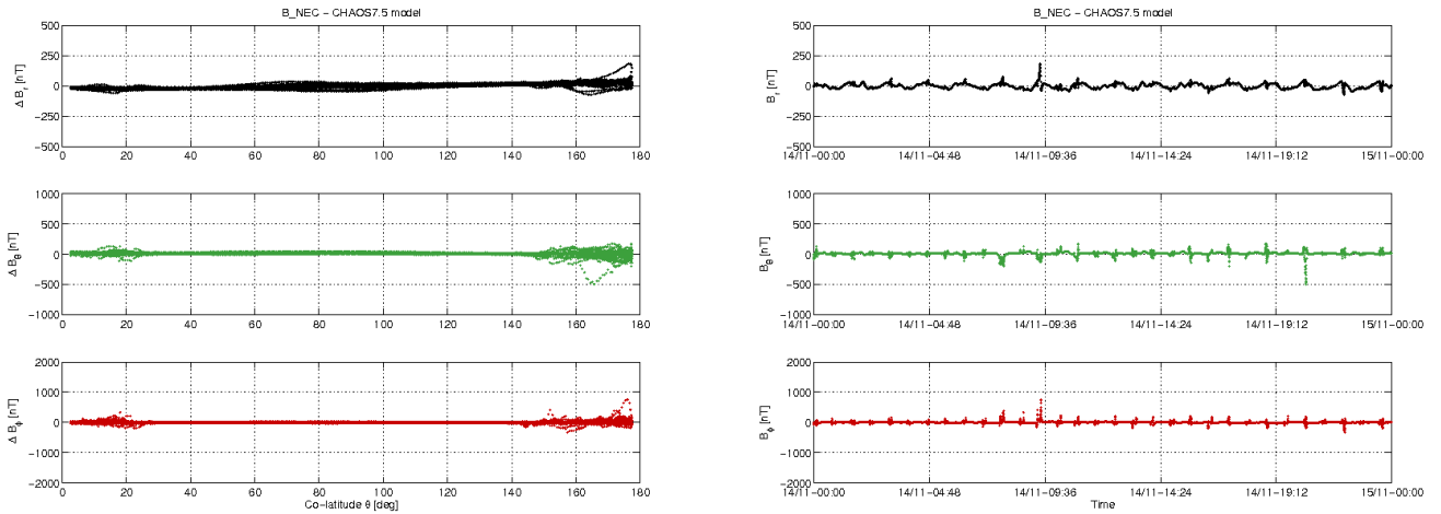
Figure 3-12: S/C C day 14/11: time series of B_{NEC} - B_{Chaos} residuals (right) and B_{NEC} - B_{Chaos} vs colatitude (left)
