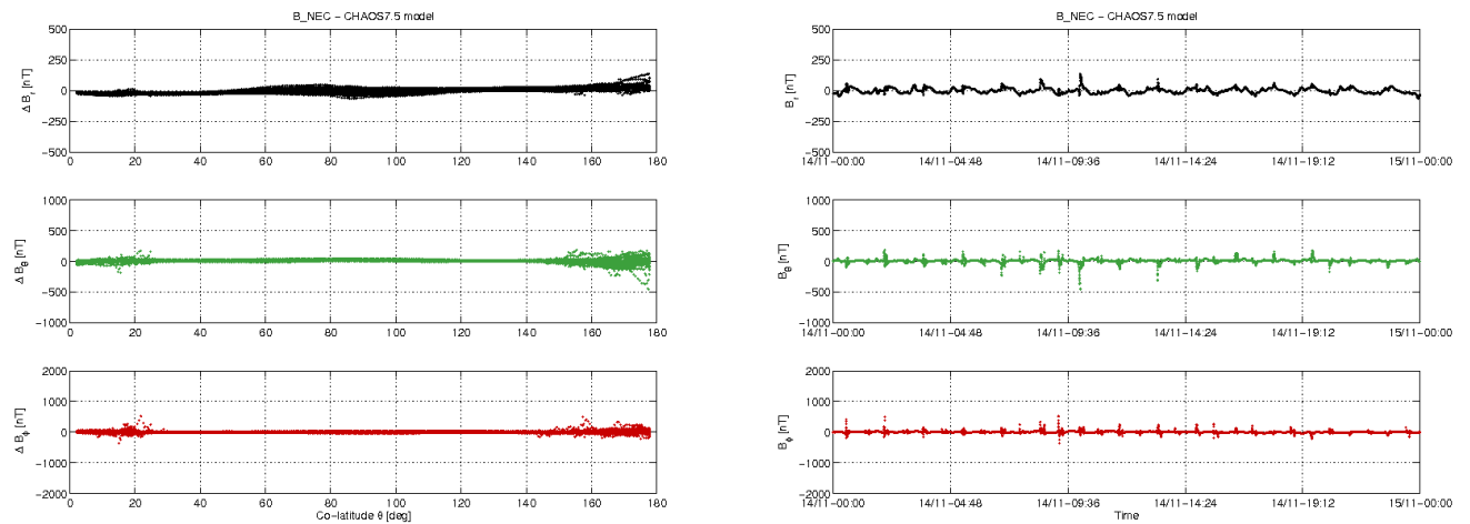
Figure 3-11: S/C B day 14/11: time series of B_{NEC} - B_{Chaos} residuals (right) and B_{NEC} - B_{Chaos} vs colatitude (left).
