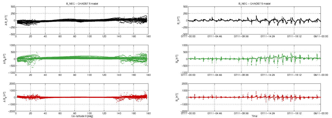
Figure 3-11: S/C B day 07/11: time series of B_{NEC} - B_{Chaos} residuals (right) and B_{NEC} - B_{Chaos} vs colatitude (left).
