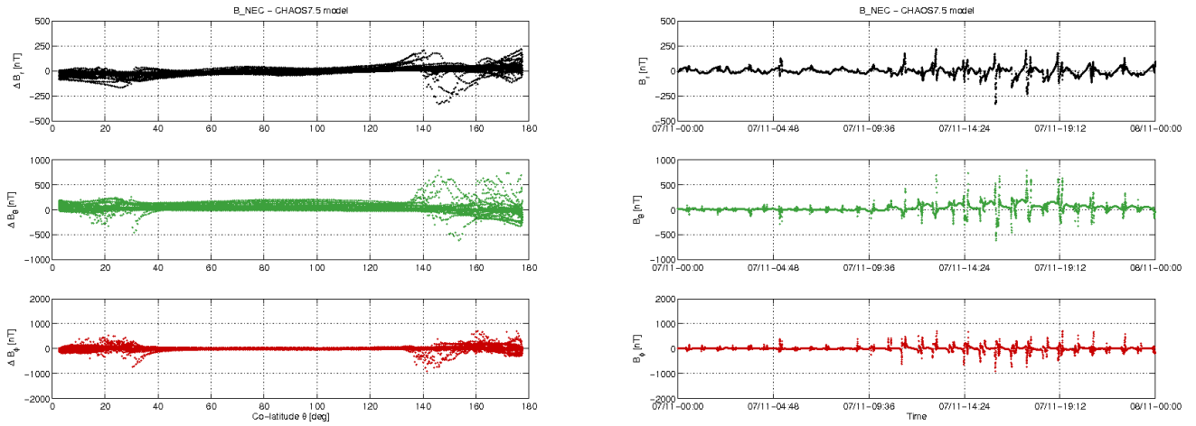
Figure 3-10: S/C A day 07/11: time series of B_{NEC} - B_{Chaos} residuals (right) and B_{NEC} - B_{Chaos} vs colatitude (left).
