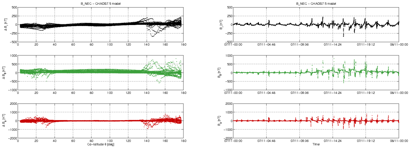
Figure 3-12: S/C C day 07/11: time series of B_{NEC} - B_{Chaos} residuals (right) and B_{NEC} - B_{Chaos} vs colatitude (left)
