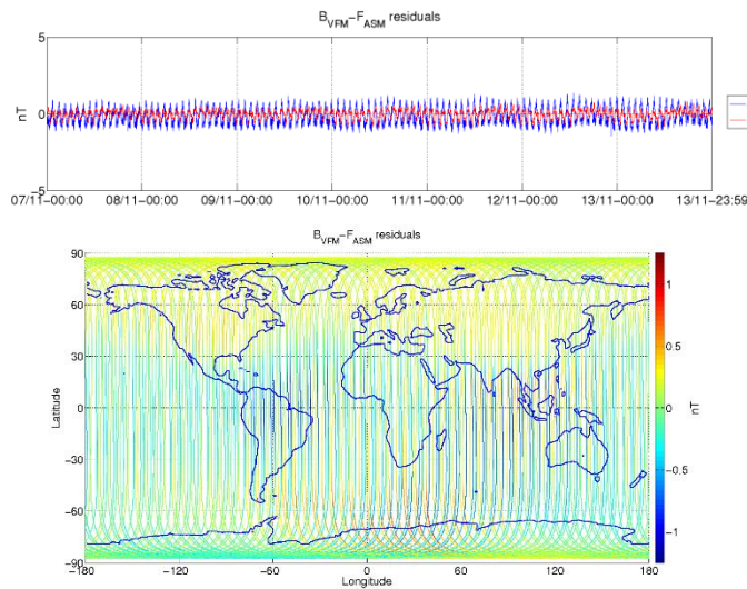
Figure 3-5: ASM-VFM residuals for S/C A, during monitoring period 07/11-13/11. In top figure are plotted: difference between |B_{VFM}| and F_{ASM} (without dB_{Sun} correction) (blue colour), and the residuals with dB_{Sun} corrections (red colour). In bottom figure residuals are presented on the world map.
