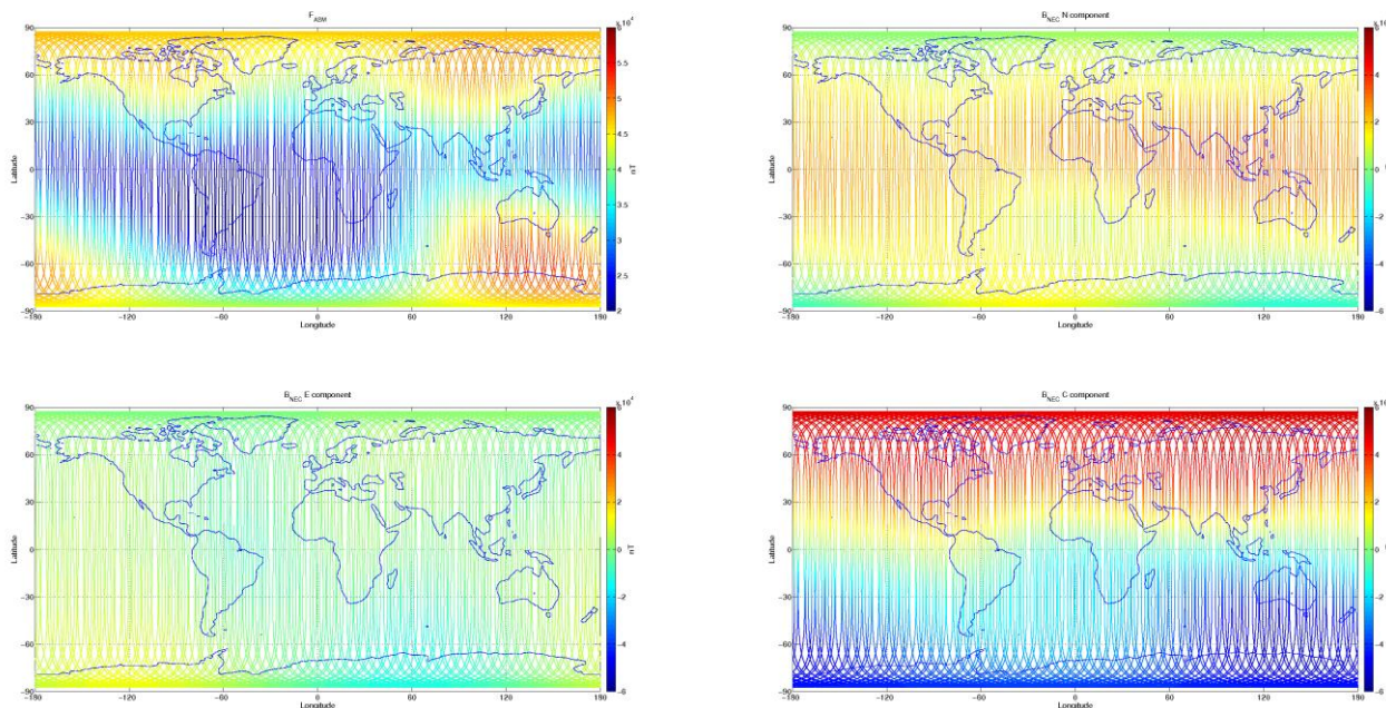
Figure 3-7: S/C A, world map plots of the geomagnetic field and components measured during monitoring period 07/11-13/11. From top to bottom: F-magnetic field from ASM measurement, B_{NEC} components (North, East, and Centre) of magnetic field from VFM measurement.
