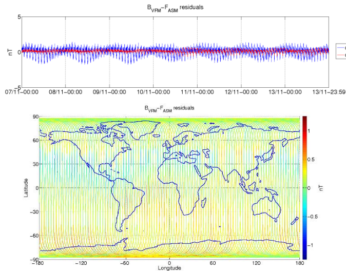
Figure 3-6: ASM-VFM residuals for S/C B, during monitoring period 07/11-13/11. In top figure are plotted: difference between |B_{VFM}| and F_{ASM} (without dB_{Sun} correction) (blue colour), and the residuals with dB_{Sun} corrections (red colour). In bottom figure residuals are presented on the world map.
