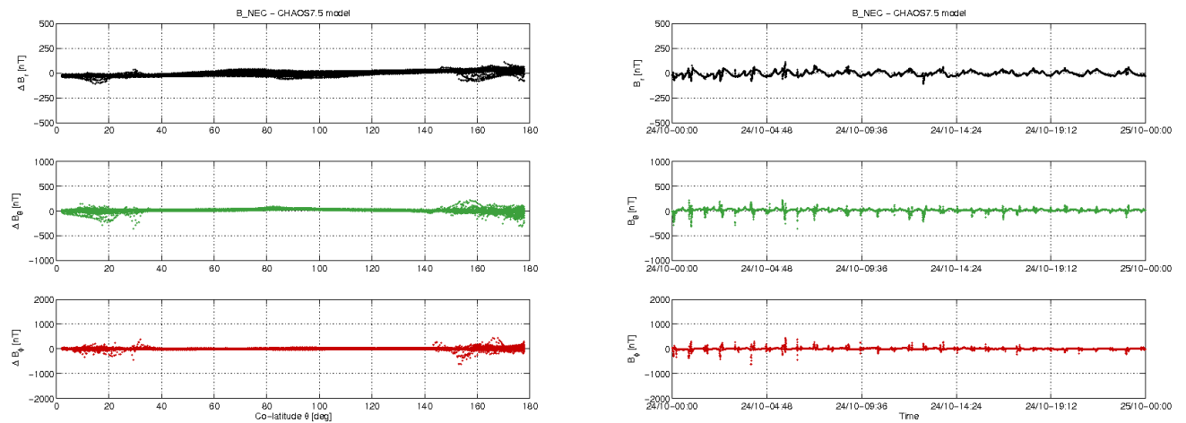
Figure 3-11: S/C B day 24/10: time series of B_{NEC} - B_{Chaos} residuals (right) and B_{NEC} - B_{Chaos} vs colatitude (left).
