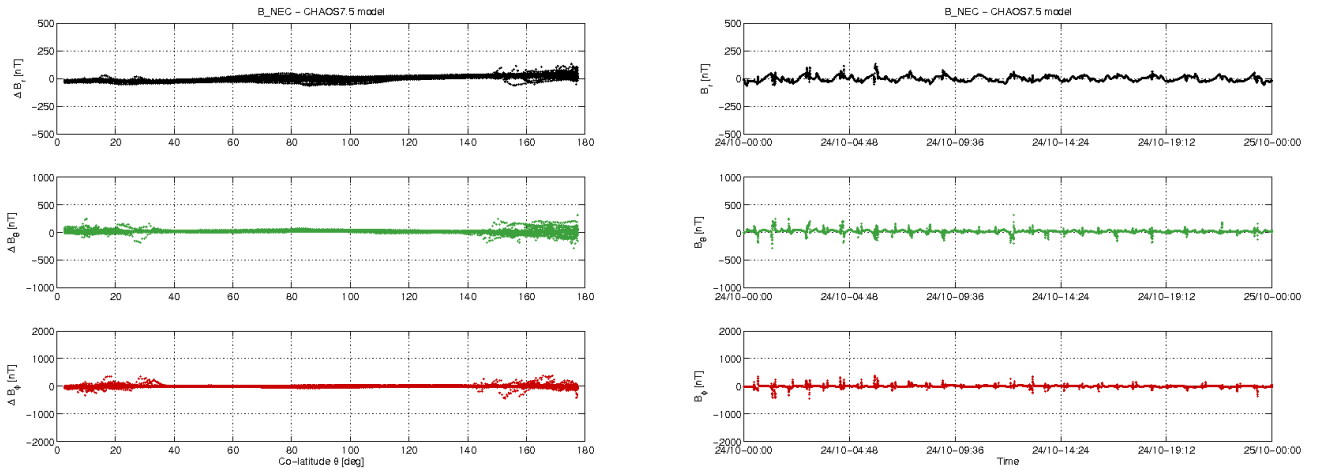
Figure 3-12: S/C C day 24/10: time series of B_{NEC} - B_{Chaos} residuals (right) and B_{NEC} - B_{Chaos} vs colatitude (left)
