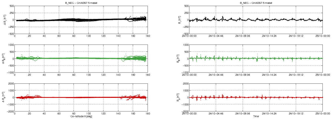
Figure 3-10: S/C A day 24/10: time series of B_{NEC} - B_{Chaos} residuals (right) and B_{NEC} - B_{Chaos} vs colatitude (left).
