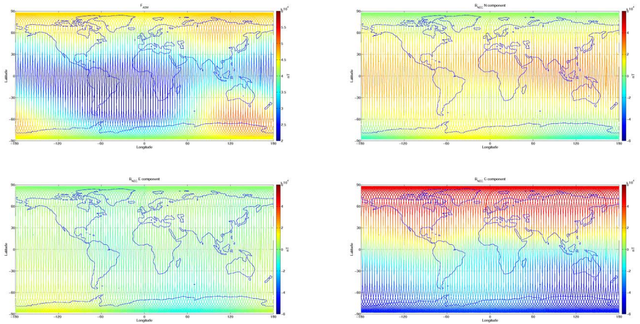
Figure 3-8: S/C B, world map plots of the geomagnetic field and components measured during monitoring period 24/10-30/10. From top to bottom: F-magnetic field from ASM measurement, B_{NEC} components (North, East, and Centre) of magnetic field from VFM measurement.
