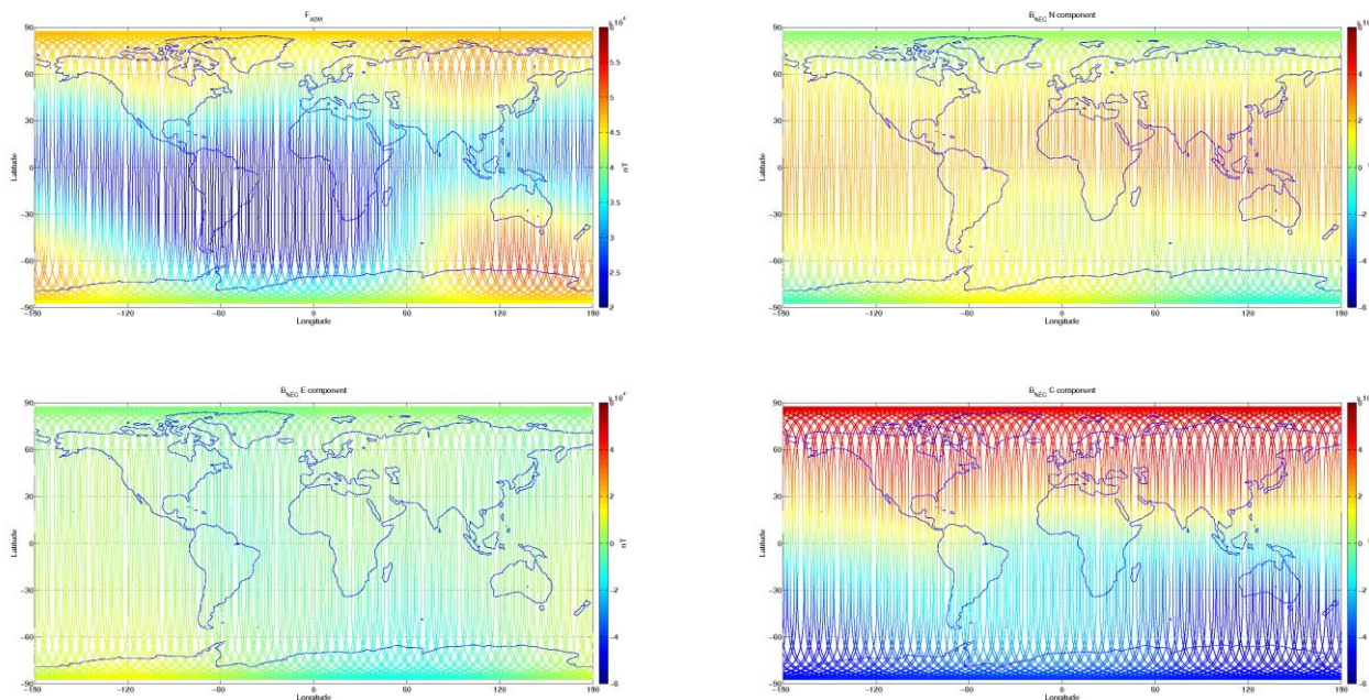
Figure 3-7: S/C A, world map plots of the geomagnetic field and components measured during monitoring period 24/10-30/10. From top to bottom: F-magnetic field from ASM measurement, B_{NEC} components (North, East, and Centre) of magnetic field from VFM measurement.
