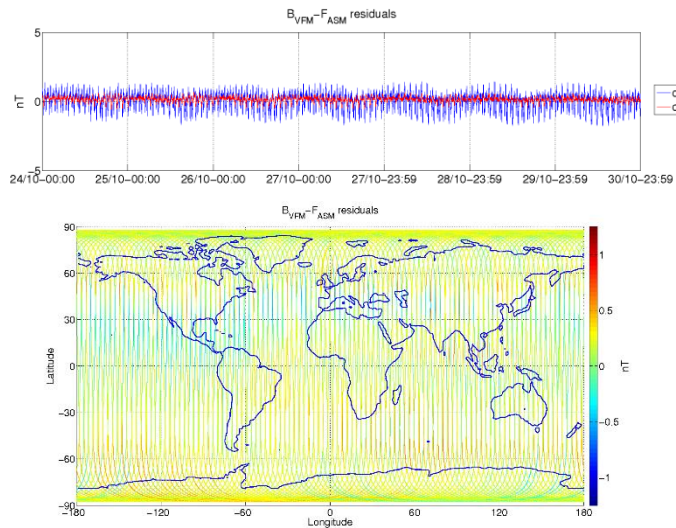
Figure 3-6: ASM-VFM residuals for S/C B, during monitoring period 24/10-30/10. In top figure are plotted: difference between |B_{VFM}| and F_{ASM} (without dB_{Sun} correction) (blue colour), and the residuals with dB_{Sun} corrections (red colour). In bottom figure residuals are presented on the world map.
