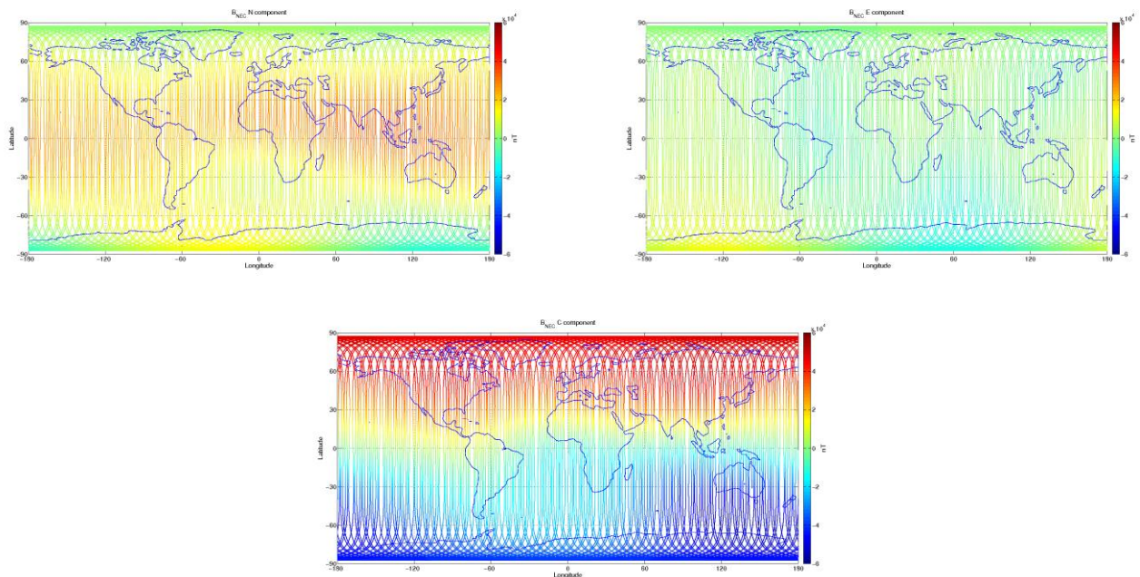
Figure 3-9: S/C C, world map plots of the geomagnetic field and components measured during monitoring period 24/10-30/10. From top to bottom: B_{NEC} components (North, East, and Centre) of magnetic field from VFM measurement.
