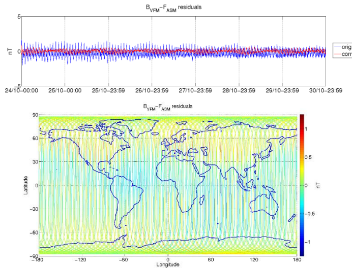
Figure 3-5: ASM-VFM residuals for S/C A, during monitoring period 24/10-30/10. In top figure are plotted: difference between |B_{VFM}| and F_{ASM} (without dB_{Sun} correction) (blue colour), and the residuals with dB_{Sun} corrections (red colour). In bottom figure residuals are presented on the world map.
