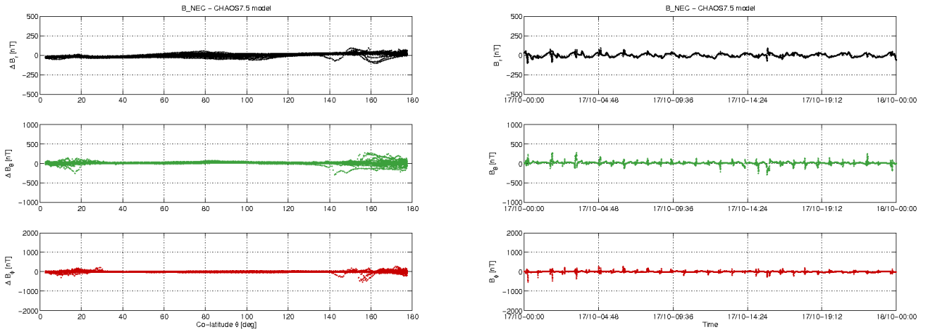
Figure 3-12: S/C C day 17/10: time series of B_{NEC} - B_{Chaos} residuals (right) and B_{NEC} - B_{Chaos} vs colatitude (left)
