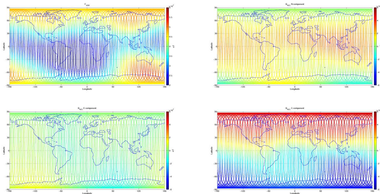
Figure 3-7: S/C A, world map plots of the geomagnetic field and components measured during monitoring period 17/10-23/10. From top to bottom: F-magnetic field from ASM measurement, B_{NEC} components (North, East, and Centre) of magnetic field from VFM measurement.
