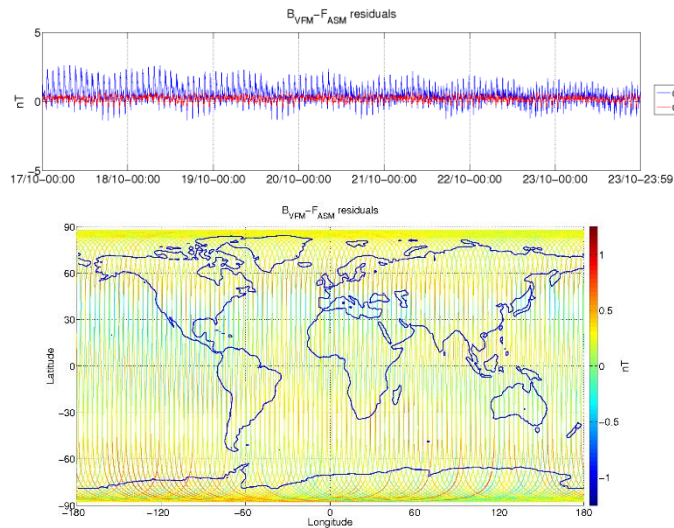
Figure 3-6: ASM-VFM residuals for S/C B, during monitoring period 17/10-23/10. In top figure are plotted: difference between |B_{VFM}| and F_{ASM} (without dB_{Sun} correction) (blue colour), and the residuals with dB_{Sun} corrections (red colour). In bottom figure residuals are presented on the world map.
