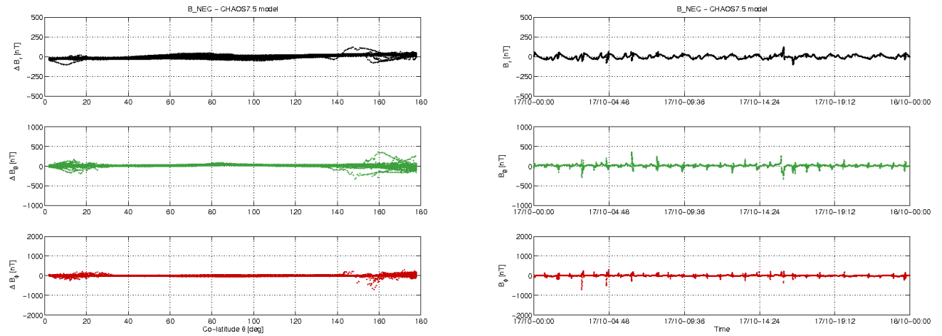
Figure 3-11: S/C B day 17/10: time series of B_{NEC} - B_{Chaos} residuals (right) and B_{NEC} - B_{Chaos} vs colatitude (left).
