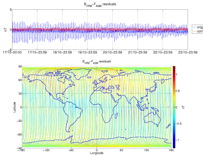
Figure 3-5: ASM-VFM residuals for S/C A, during monitoring period 17/10-23/10. In top figure are plotted: difference between |B_{VFM}| and F_{ASM} (without dB_{Sun} correction) (blue colour), and the residuals with dB_{Sun} corrections (red colour). In bottom figure residuals are presented on the world map.
