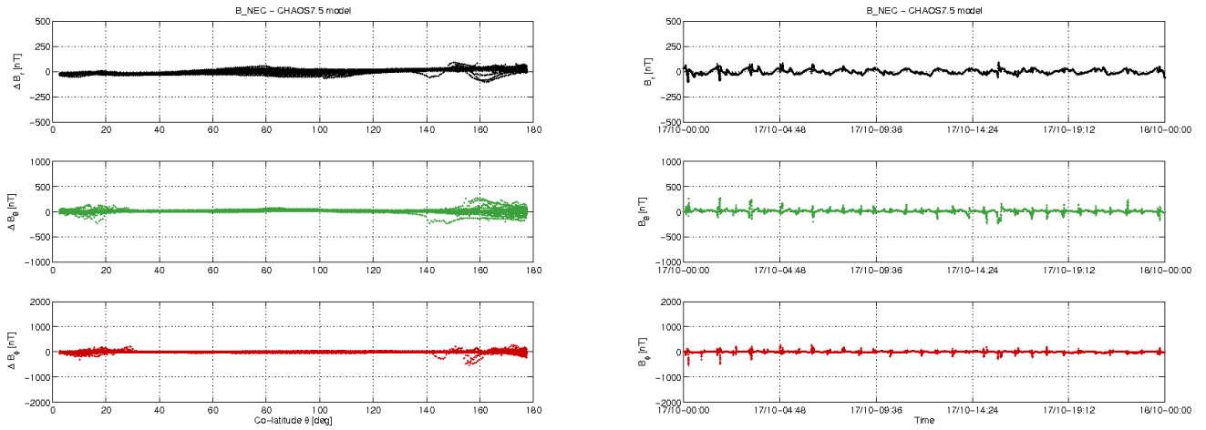
Figure 3-10: S/C A day 17/10: time series of B_{NEC} - B_{Chaos} residuals (right) and B_{NEC} - B_{Chaos} vs colatitude (left).
