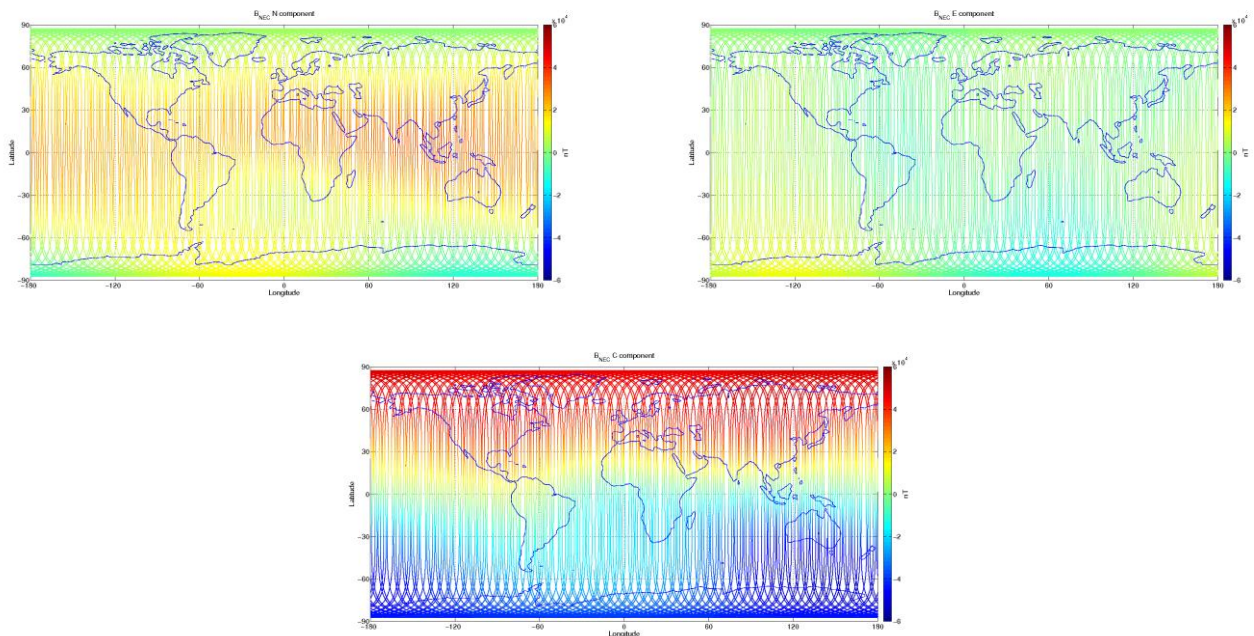
Figure 3-9: S/C C, world map plots of the geomagnetic field and components measured during monitoring period 17/10-23/10. From top to bottom: B_{NEC} components (North, East, and Centre) of magnetic field from VFM measurement.
