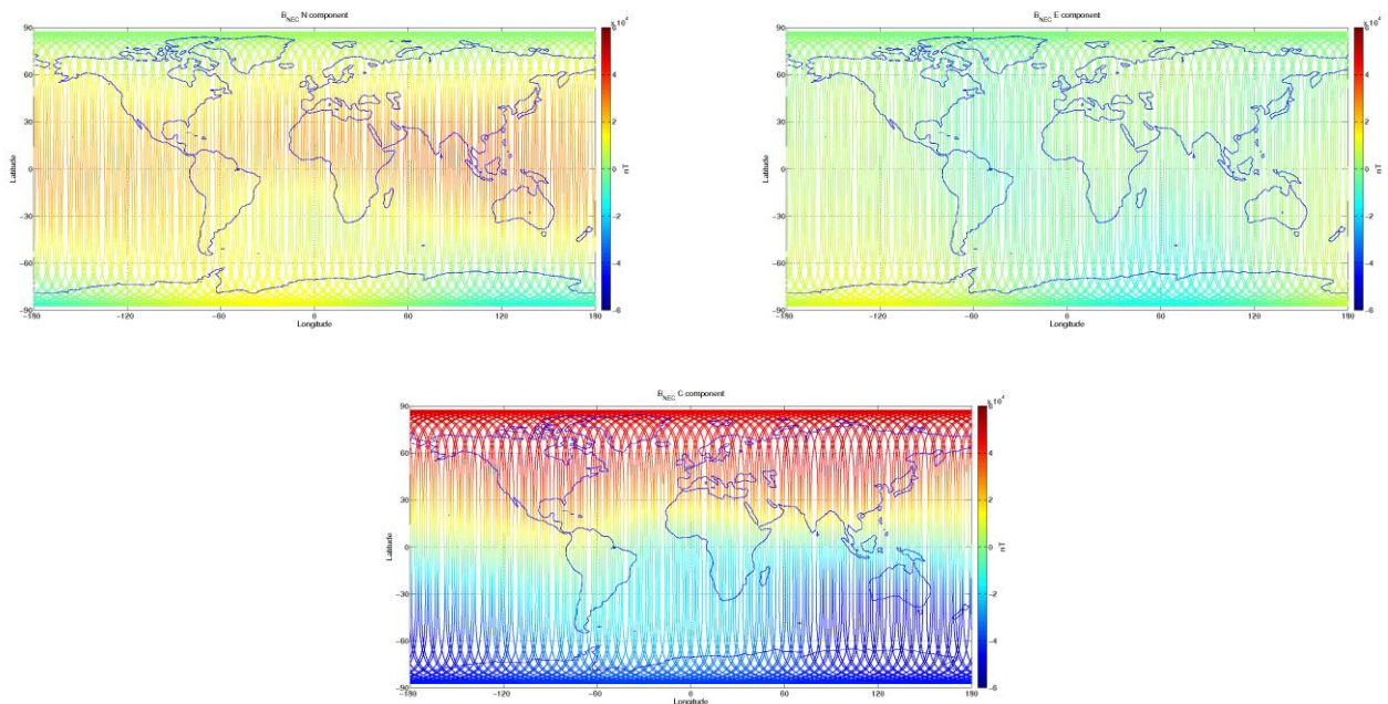
Figure 3-9: S/C C, world map plots of the geomagnetic field and components measured during monitoring period 03/10-09/10. From top to bottom: B_{NEC} components (North, East, and Centre) of magnetic field from VFM measurement.
