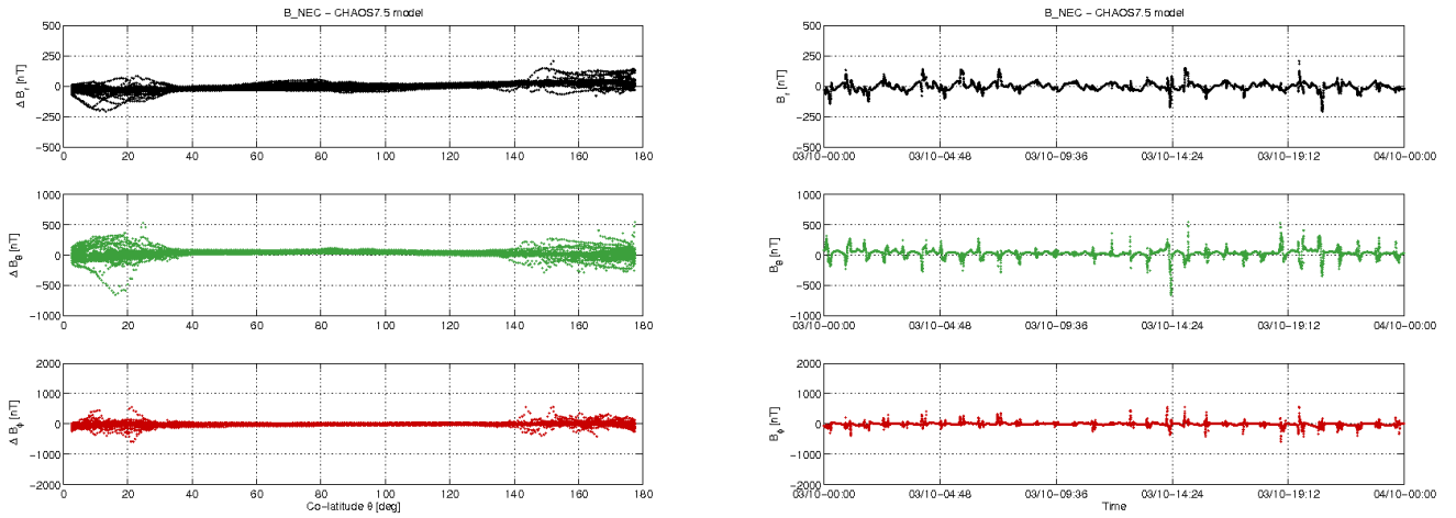
Figure 3-10: S/C A day 03.10: time series of B_{NEC} - B_{Chaos} residuals (right) and B_{NEC} - B_{Chaos} vs colatitude (left).
