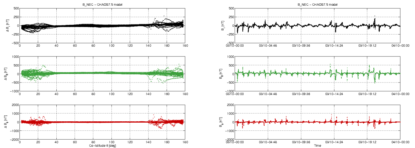
Figure 3-11: S/C B day 03.10: time series of B_{NEC} - B_{Chaos} residuals (right) and B_{NEC} - B_{Chaos} vs colatitude (left).
