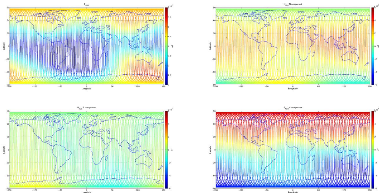
Figure 3-7: S/C A, world map plots of the geomagnetic field and components measured during monitoring period 03/10-09/10. From top to bottom: F-magnetic field from ASM measurement, B_{NEC} components (North, East, and Centre) of magnetic field from VFM measurement.
