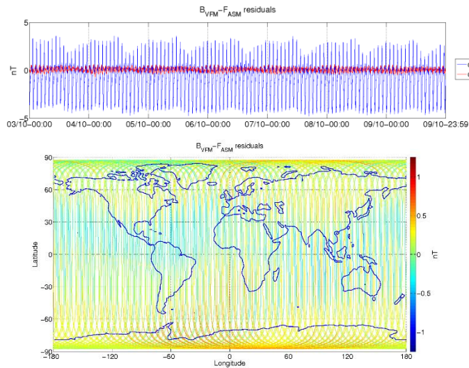
Figure 3-5: ASM-VFM residuals for S/C A, during monitoring period 03/10-09/10. In top figure are plotted: difference between |B_{VFM}| and F_{ASM} (without dB_{Sun} correction) (blue colour), and the residuals with dB_{Sun} corrections (red colour). In bottom figure residuals are presented on the world map.
