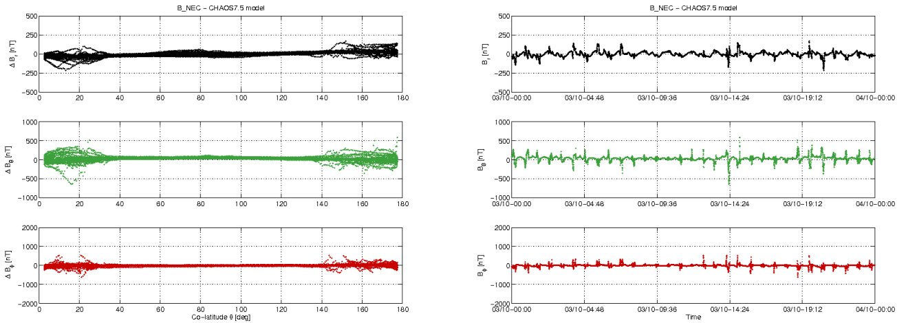
Figure 3-12: S/C C day 03.10: time series of B_{NEC} - B_{Chaos} residuals (right) and B_{NEC} - B_{Chaos} vs colatitude (left)
