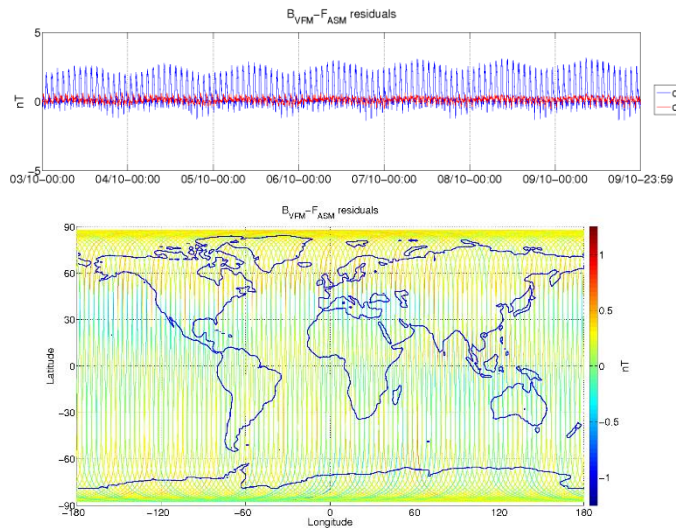
Figure 3-6: ASM-VFM residuals for S/C B, during monitoring period 03/10-09/10. In top figure are plotted: difference between |B_{VFM}| and F_{ASM} (without dB_{Sun} correction) (blue colour), and the residuals with dB_{Sun} corrections (red colour). In bottom figure residuals are presented on the world map.
