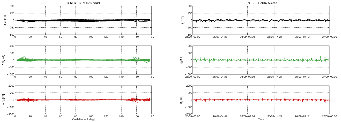
Figure 3-12: S/C C day 26.09: time series of B_{NEC} - B_{Chaos} residuals (right) and B_{NEC} - B_{Chaos} vs colatitude (left)
