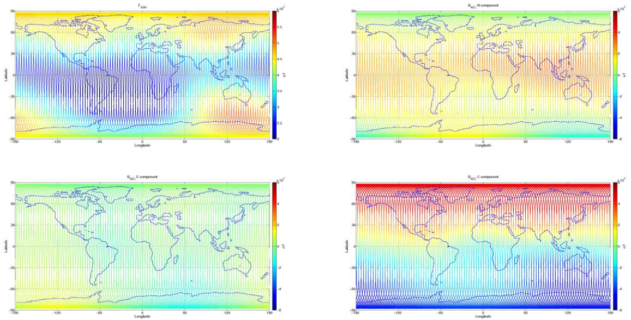
Figure 3-8: S/C B, world map plots of the geomagnetic field and components measured during monitoring period 26/09-02/10. From top to bottom: F-magnetic field from ASM measurement, B_{NEC} components (North, East, and Centre) of magnetic field from VFM measurement.
