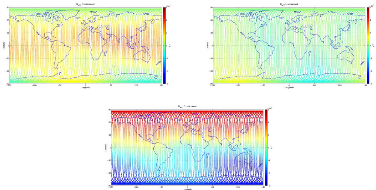
Figure 3-9: S/C C, world map plots of the geomagnetic field and components measured during monitoring period 26/09-02/10. From top to bottom: B_{NEC} components (North, East, and Centre) of magnetic field from VFM measurement.
