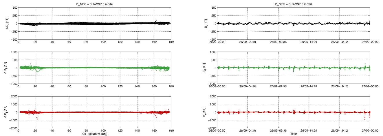
Figure 3-11: S/C B day 26.09: time series of B_{NEC} - B_{Chaos} residuals (right) and B_{NEC} - B_{Chaos} vs colatitude (left).
