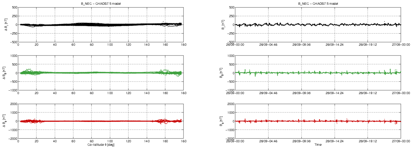
Figure 3-10: S/C A day 26.09: time series of B_{NEC} - B_{Chaos} residuals (right) and B_{NEC} - B_{Chaos} vs colatitude (left).
