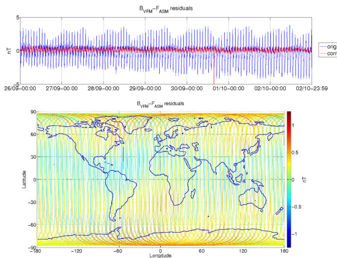
Figure 3-5: ASM-VFM residuals for S/C A, during monitoring period 26/09-02/10. In top figure are plotted: difference between |B_{VFM}| and F_{ASM} (without dB_{Sun} correction) (blue colour), and the residuals with dB_{Sun} corrections (red colour). In bottom figure residuals are presented on the world map.
