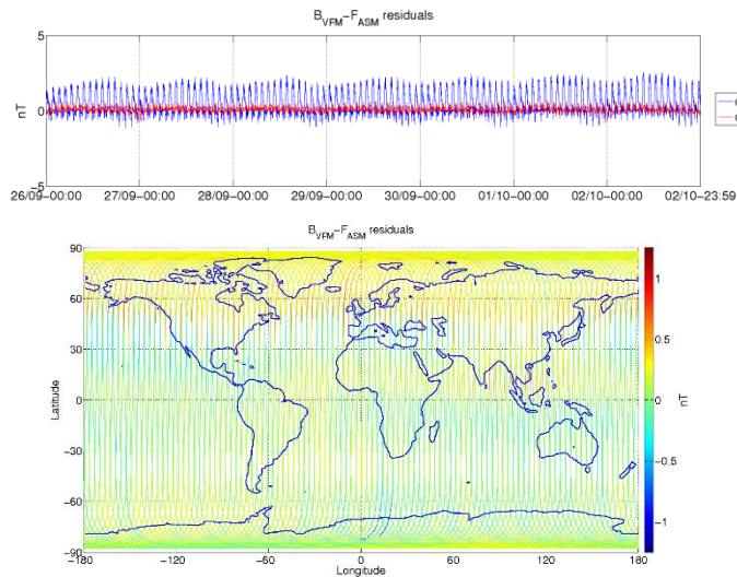
Figure 3-6: ASM-VFM residuals for S/C B, during monitoring period 26/09-02/10. In top figure are plotted: difference between |B_{VFM}| and F_{ASM} (without dB_{Sun} correction) (blue colour), and the residuals with dB_{Sun} corrections (red colour). In bottom figure residuals are presented on the world map.
