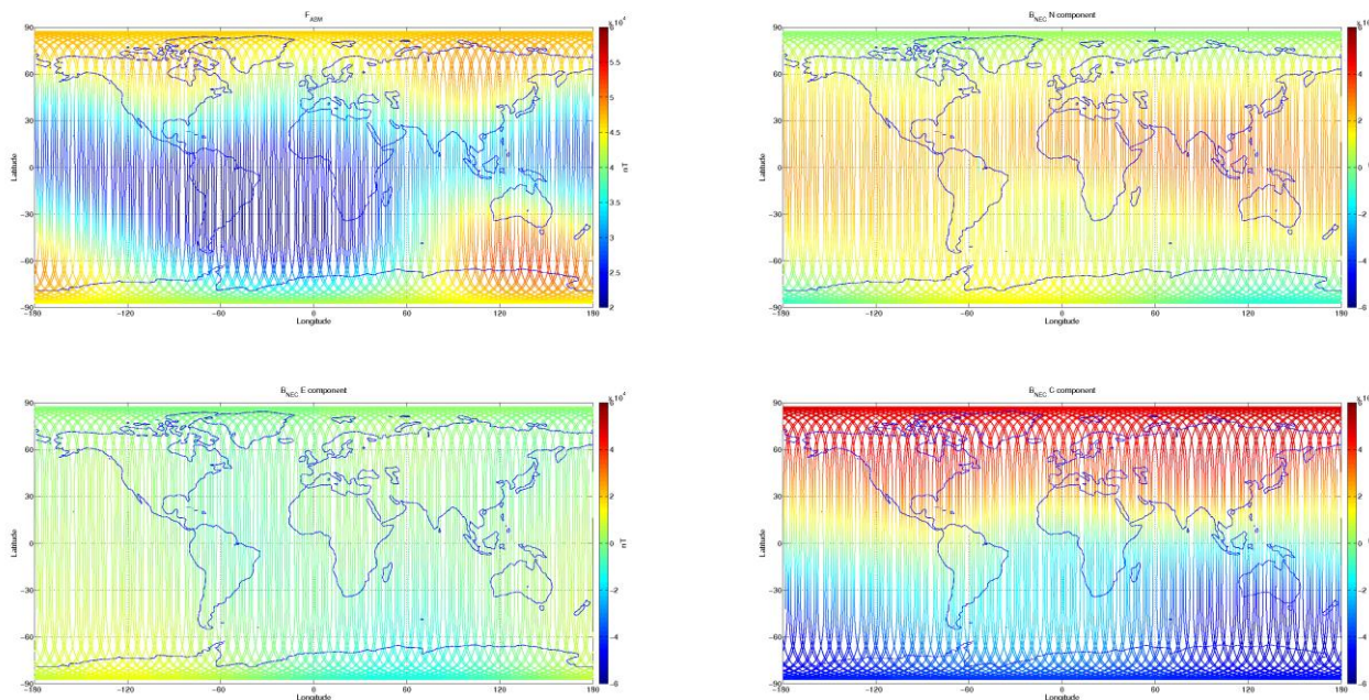
Figure 3-7: S/C A, world map plots of the geomagnetic field and components measured during monitoring period 26/09-02/10. From top to bottom: F-magnetic field from ASM measurement, B_{NEC} components (North, East, and Centre) of magnetic field from VFM measurement.
