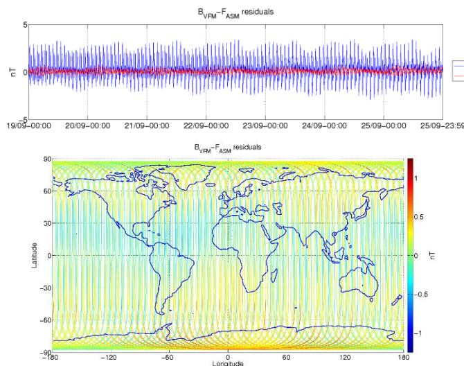
Figure 3-5: ASM-VFM residuals for S/C A, during monitoring period 19/09-25/09. In top figure are plotted: difference between |B_{VFM}| and F_{ASM} (without dB_{Sun} correction) (blue colour), and the residuals with dB_{Sun} corrections (red colour). In bottom figure residuals are presented on the world map.
