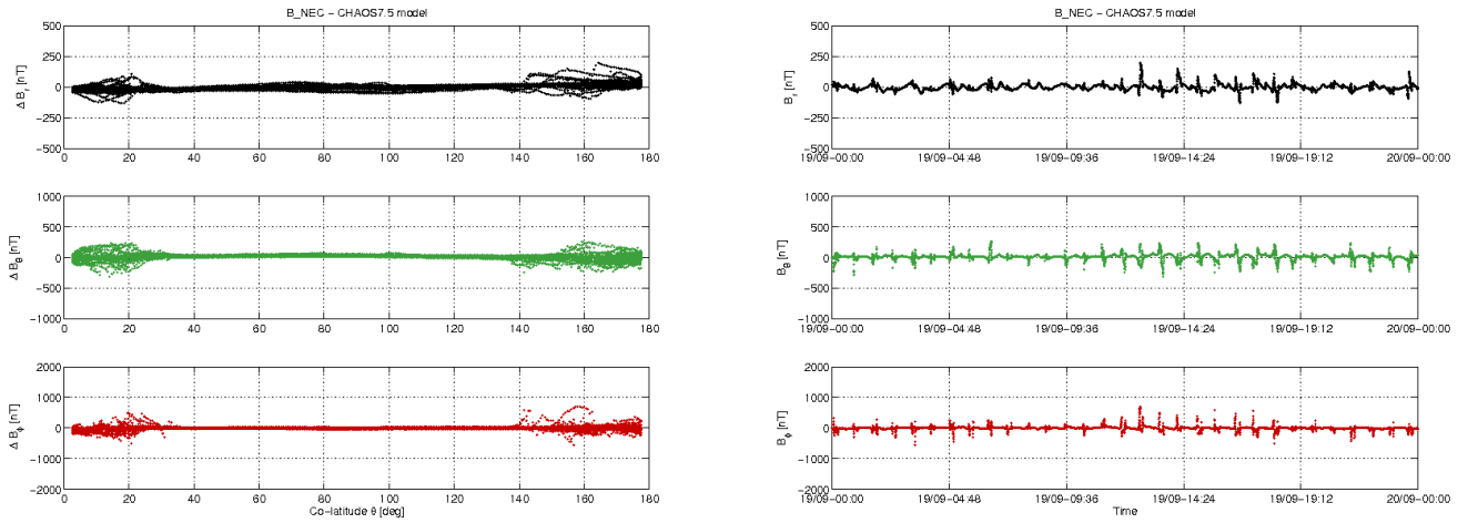
Figure 3-10: S/C A day 19.09: time series of B_{NEC} - B_{Chaos} residuals (right) and B_{NEC} - B_{Chaos} vs colatitude (left).
