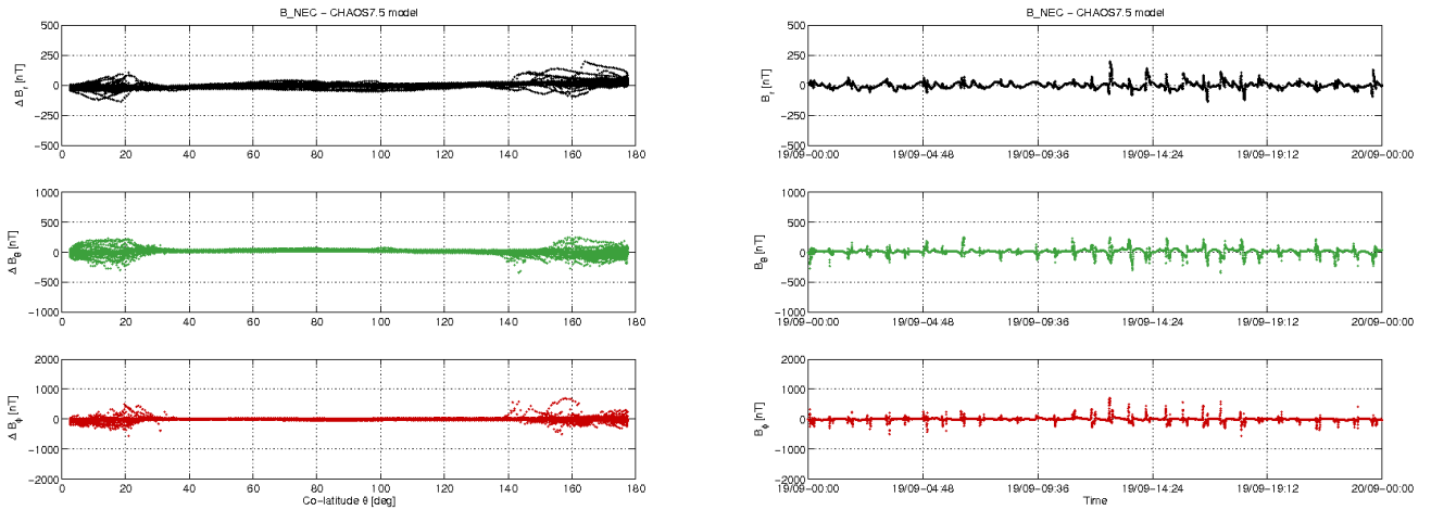
Figure 3-12: S/C C day 19:09: time series of B_{NEC} - B_{Chaos} residuals (right) and B_{NEC} - B_{Chaos} vs colatitude (left)
