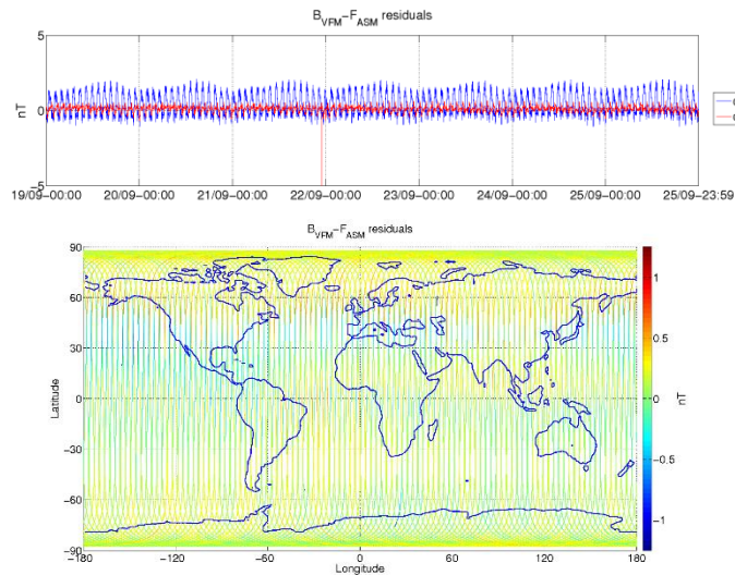
Figure 3-6: ASM-VFM residuals for S/C B, during monitoring period 19/09-25/09. In top figure are plotted: difference between |B_{VFM}| and F_{ASM} (without dB_{Sun} correction) (blue colour), and the residuals with dB_{Sun} corrections (red colour). In bottom figure residuals are presented on the world map.
