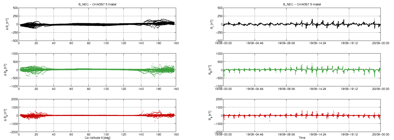
Figure 3-11: S/C B day 19.09: time series of B_{NEC} - B_{Chaos} residuals (right) and B_{NEC} - B_{Chaos} vs colatitude (left).
