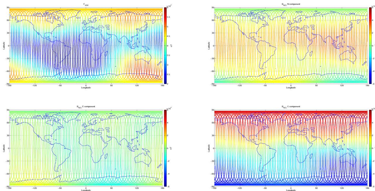
Figure 3-7: S/C A, world map plots of the geomagnetic field and components measured during monitoring period 19/09-25/09. From top to bottom: F-magnetic field from ASM measurement, B_{NEC} components (North, East, and Centre) of magnetic field from VFM measurement.
