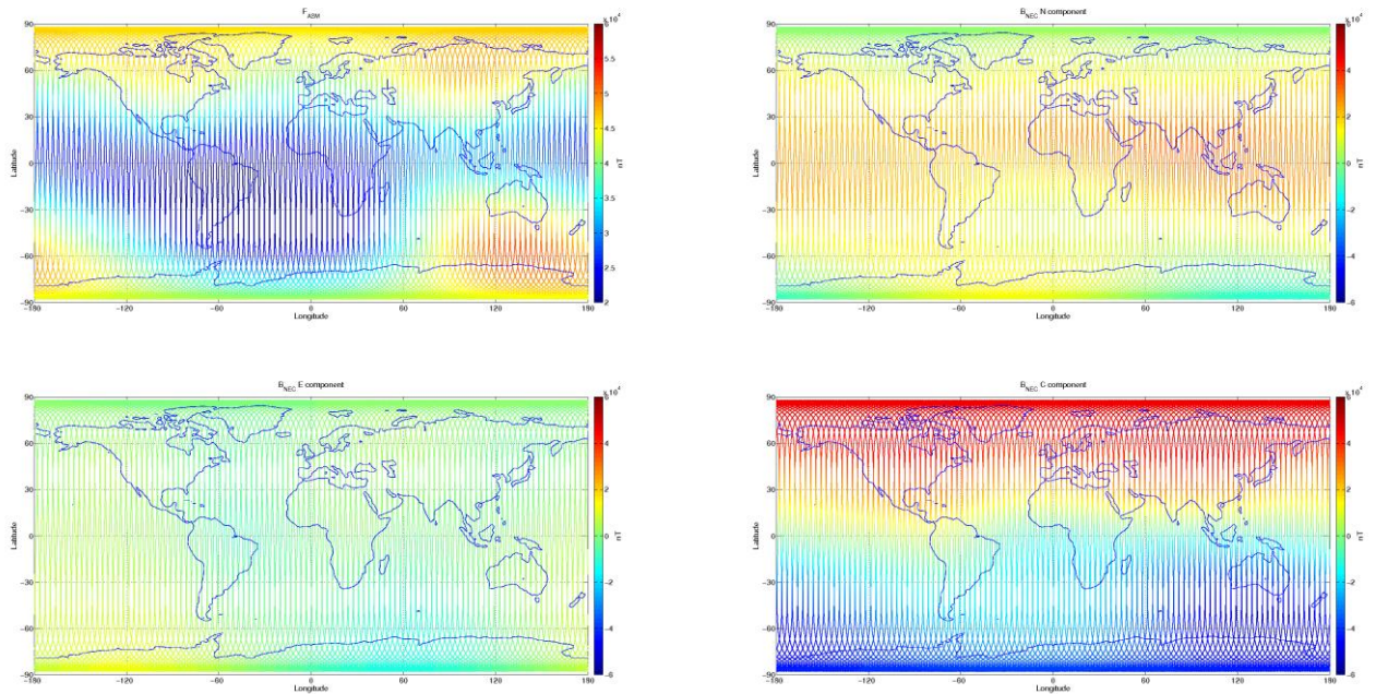
Figure 3-8: S/C B, world map plots of the geomagnetic field and components measured during monitoring period 19/09-25/09. From top to bottom: F-magnetic field from ASM measurement, B_{NEC} components (North, East, and Centre) of magnetic field from VFM measurement.
