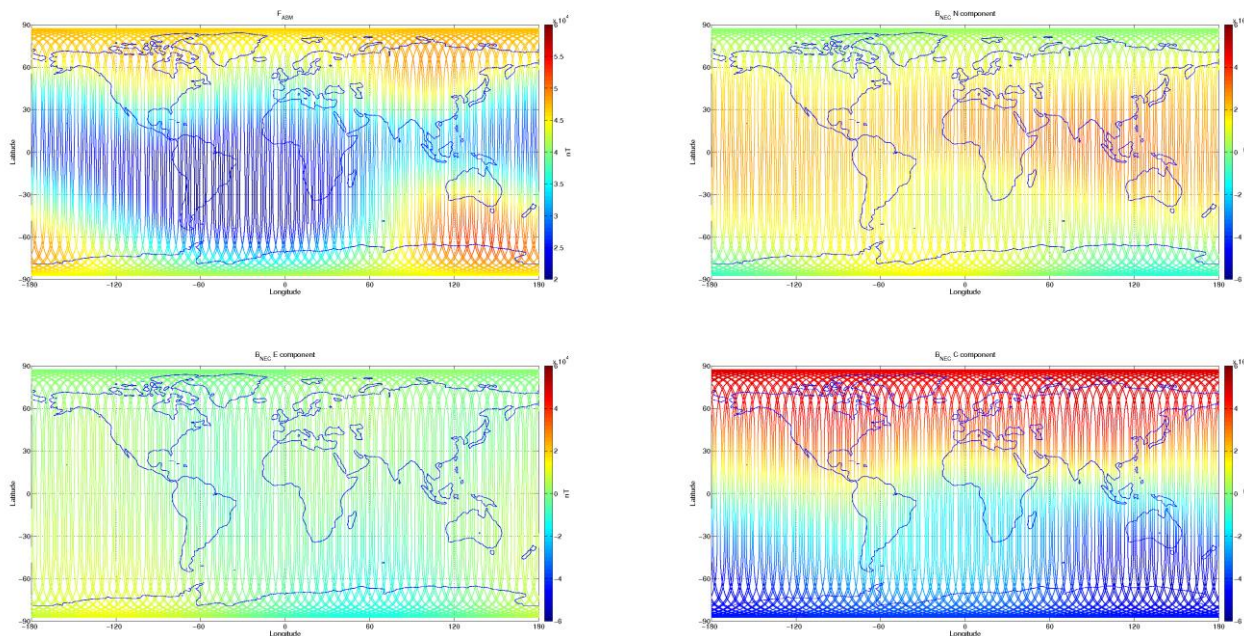
Figure 3-7: S/C A, world map plots of the geomagnetic field and components measured during monitoring period 12/09-18/09. From top to bottom: F-magnetic field from ASM measurement, B_{NEC} components (North, East, and Centre) of magnetic field from VFM measurement.
