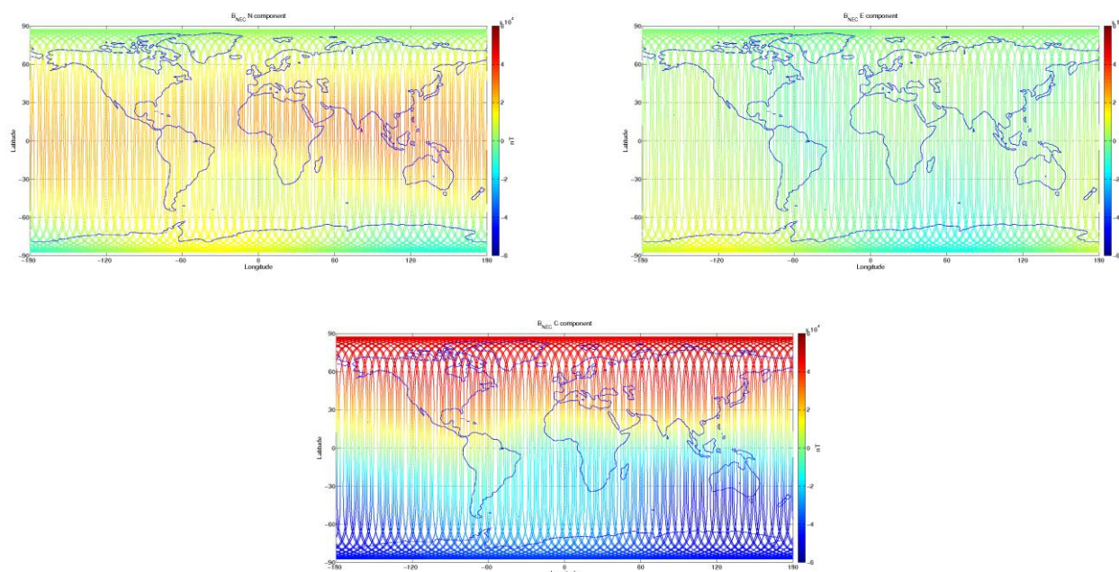
Figure 3-9: S/C C, world map plots of the geomagnetic field and components measured during monitoring period 12/09-18/09. From top to bottom: B_{NEC} components (North, East, and Centre) of magnetic field from VFM measurement.
