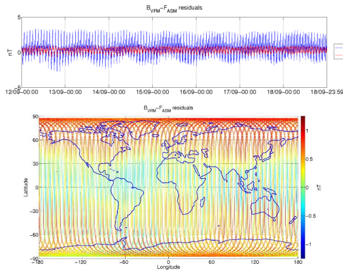
Figure 3-5: ASM-VFM residuals for S/C A, during monitoring period 12/09-18/09. In top figure are plotted: difference between |B_{VFM}| and F_{ASM} (without dB_{Sun} correction) (blue colour), and the residuals with dB_{Sun} corrections (red colour). In bottom figure residuals are presented on the world map.
