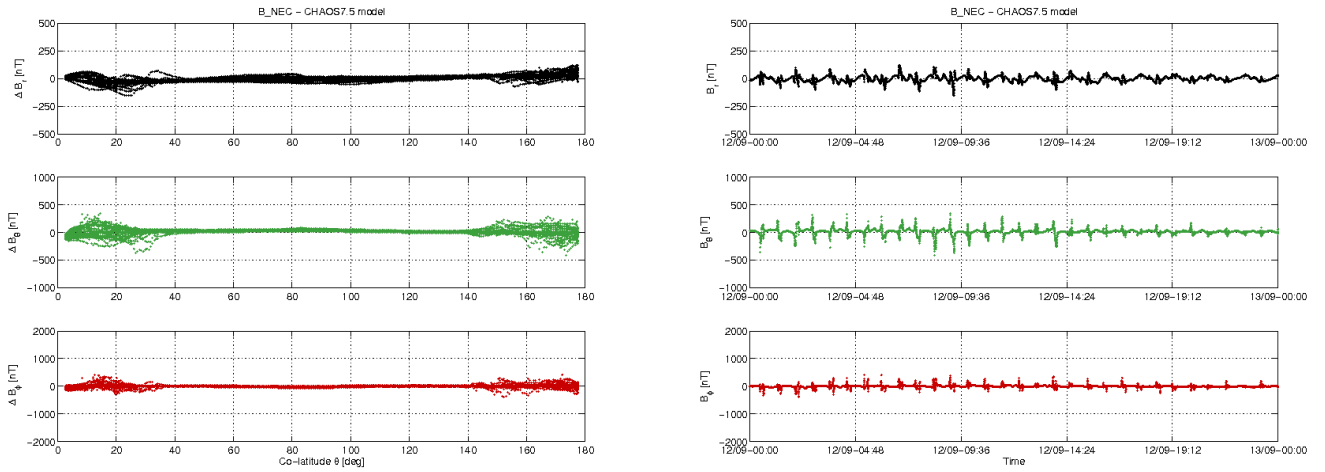
Figure 3-10: S/C A day 12/09: time series of B_{NEC} - B_{Chaos} residuals (right) and B_{NEC} - B_{Chaos} vs colatitude (left).
