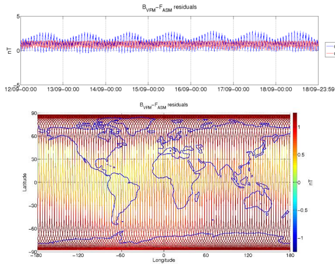
Figure 3-6: ASM-VFM residuals for S/C B, during monitoring period 12/09-18/09. In top figure are plotted: difference between |B_{VFM}| and F_{ASM} (without dB_{Sun} correction) (blue colour), and the residuals with dB_{Sun} corrections (red colour). In bottom figure residuals are presented on the world map.
