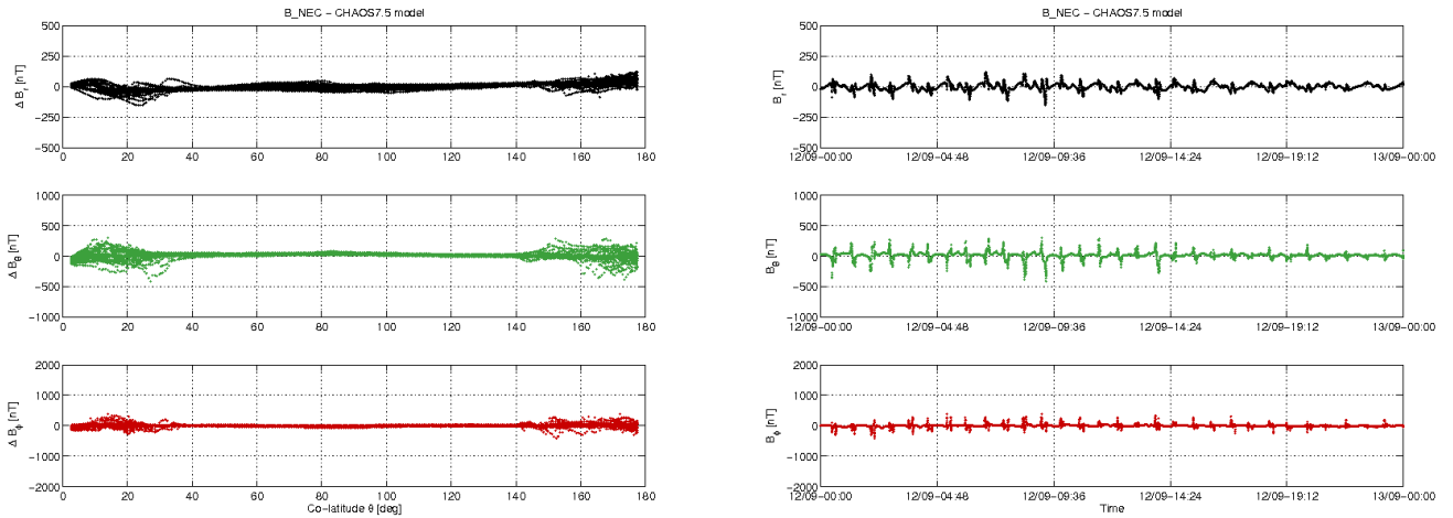
Figure 3-12: S/C C day 12/09: time series of B_{NEC} - B_{Chaos} residuals (right) and B_{NEC} - B_{Chaos} vs colatitude (left)
