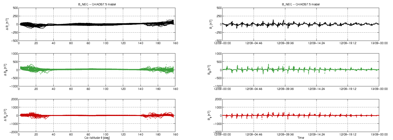
Figure 3-11: S/C B day 12/09: time series of B_{NEC} - B_{Chaos} residuals (right) and B_{NEC} - B_{Chaos} vs colatitude (left).
