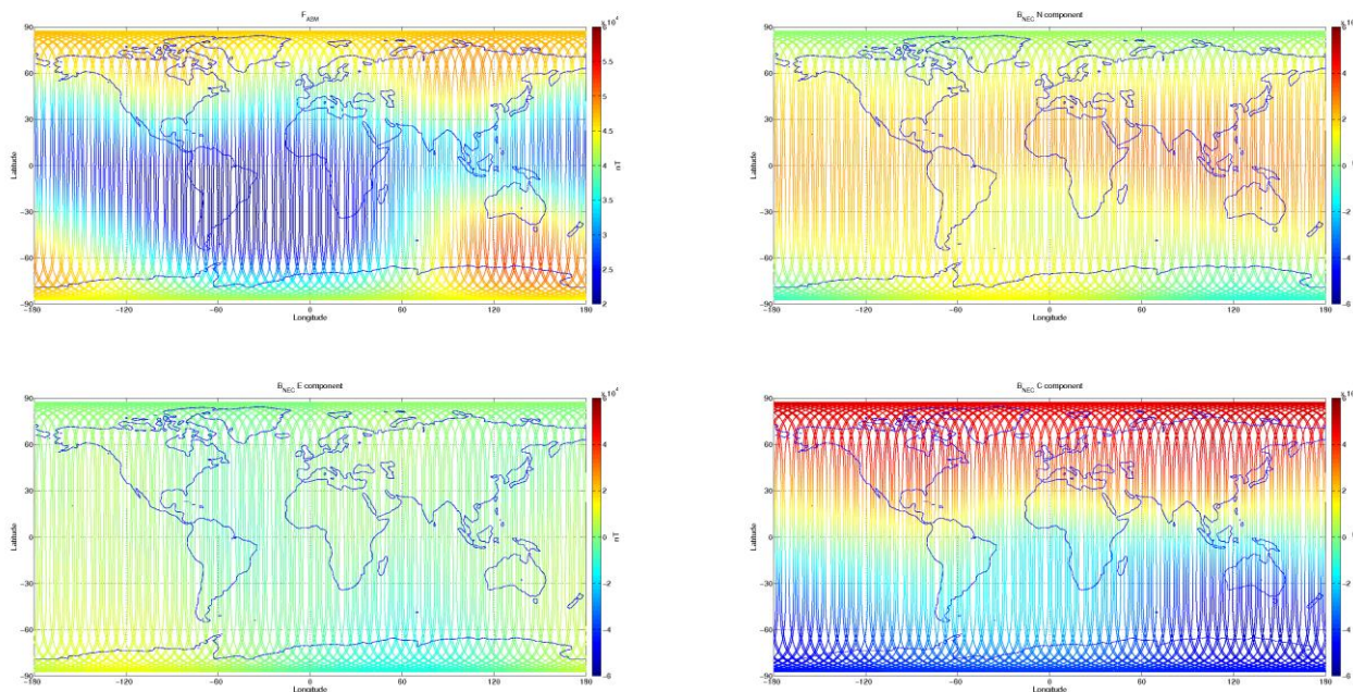
Figure 3-7: S/C A, world map plots of the geomagnetic field and components measured during monitoring period 05/09-11/09. From top to bottom: F-magnetic field from ASM measurement, B_{NEC} components (North, East, and Centre) of magnetic field from VFM measurement.
