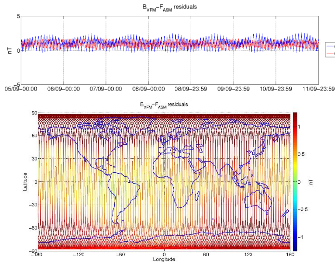
Figure 3-6: ASM-VFM residuals for S/C B, during monitoring period 05/09-11/09. In top figure are plotted: difference between |B_{VFM}| and F_{ASM} (without dB_{Sun} correction) (blue colour), and the residuals with dB_{Sun} corrections (red colour). In bottom figure residuals are presented on the world map.
