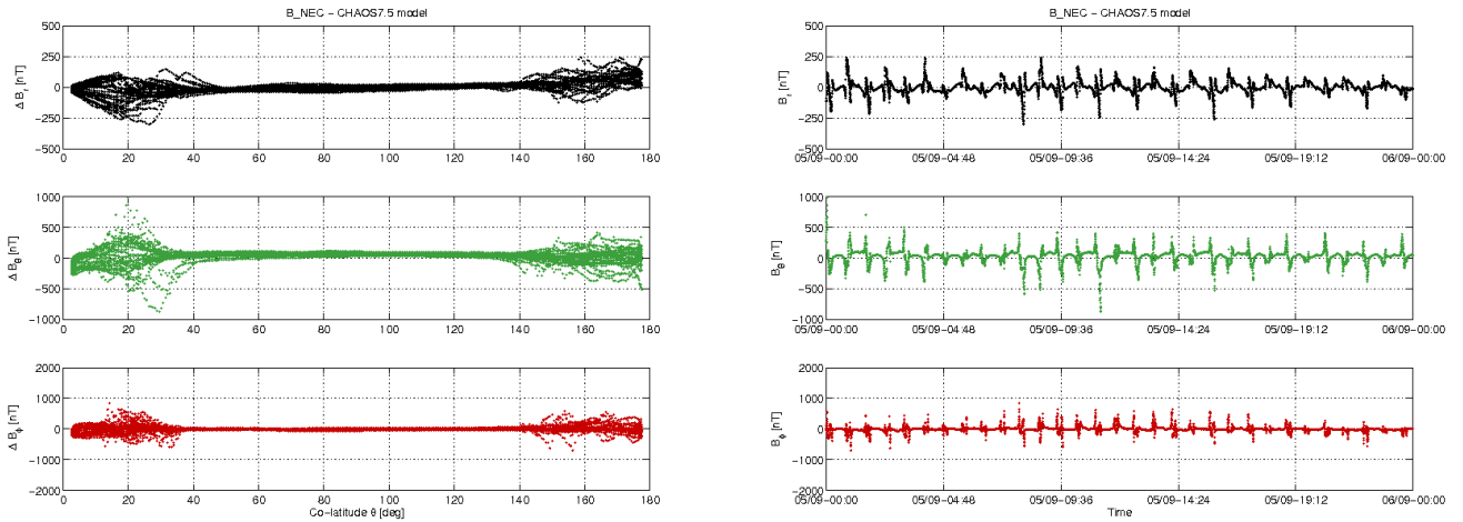
Figure 3-12: S/C C day 05/09: time series of B_{NEC} - B_{Chaos} residuals (right) and B_{NEC} - B_{Chaos} vs colatitude (left)
