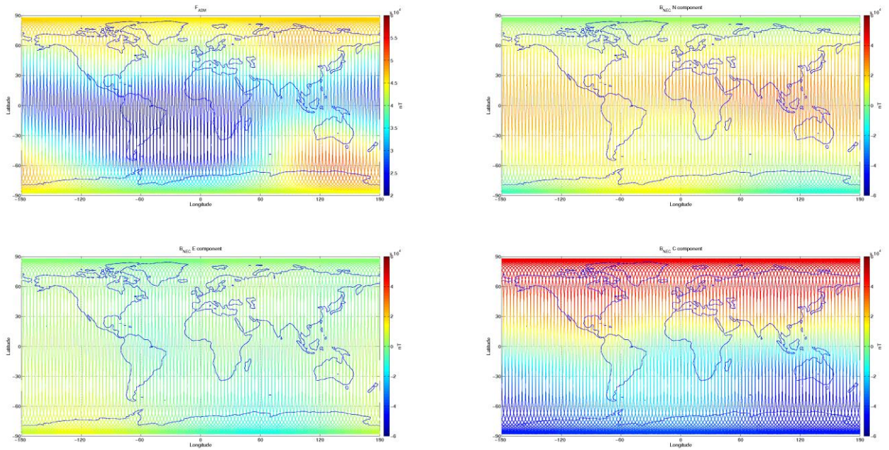
Figure 3-8: S/C B, world map plots of the geomagnetic field and components measured during monitoring period 05/09-11/09. From top to bottom: F-magnetic field from ASM measurement, B_{NEC} components (North, East, and Centre) of magnetic field from VFM measurement.
