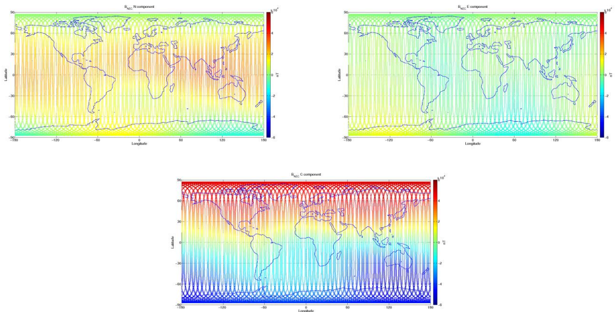
Figure 3-9: S/C C, world map plots of the geomagnetic field and components measured during monitoring period 05/09-11/09. From top to bottom: B_{NEC} components (North, East, and Centre) of magnetic field from VFM measurement.
