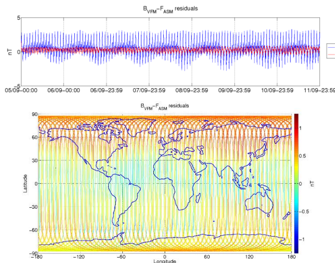
Figure 3-5: ASM-VFM residuals for S/C A, during monitoring period 05/09-11/09. In top figure are plotted: difference between |B_{VFM}| and F_{ASM} (without dB_Sun correction) (blue colour), and the residuals with dB_Sun corrections (red colour). In bottom figure residuals are presented on the world map.
