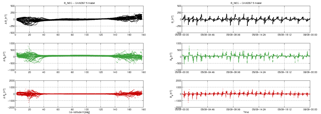
Figure 3-11: S/C B day 05/09: time series of B_{NEC} - B_{Chaos} residuals (right) and B_{NEC} - B_{Chaos} vs colatitude (left).
