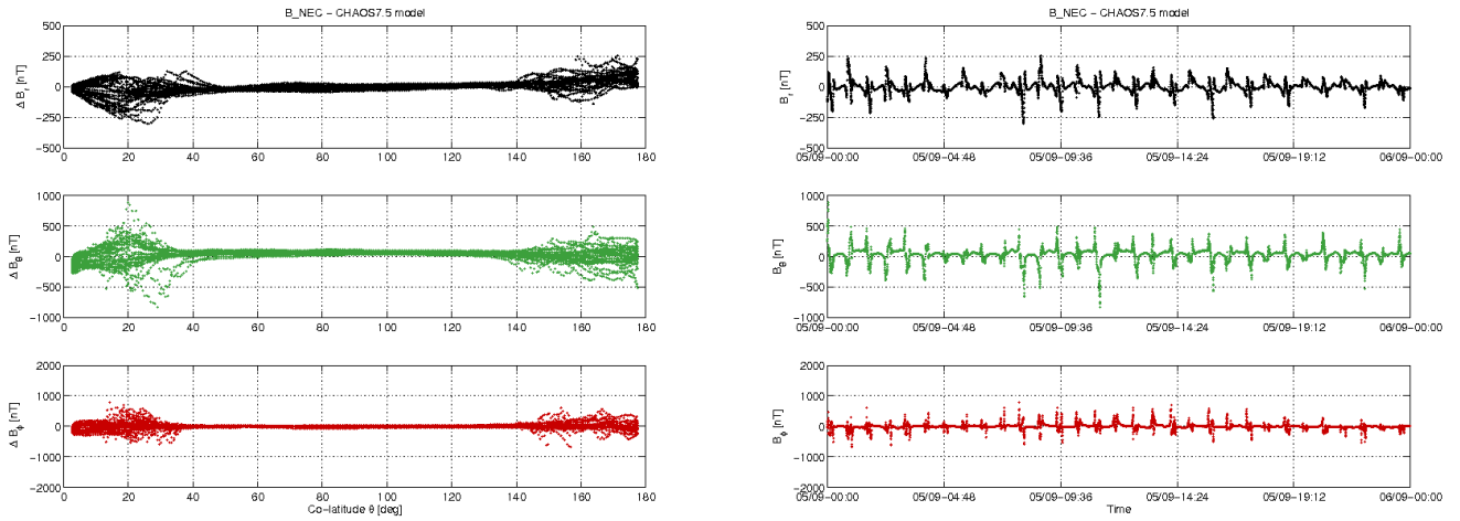
Figure 3-10: S/C A day 05/09: time series of B_{NEC} - B_{Chaos} residuals (right) and B_{NEC} - B_{Chaos} vs colatitude (left).
