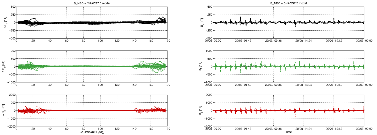
Figure 3-12: S/C C day 29/08: time series of B_{NEC} - B_{Chaos} residuals (right) and B_{NEC} - B_{Chaos} vs colatitude (left)
