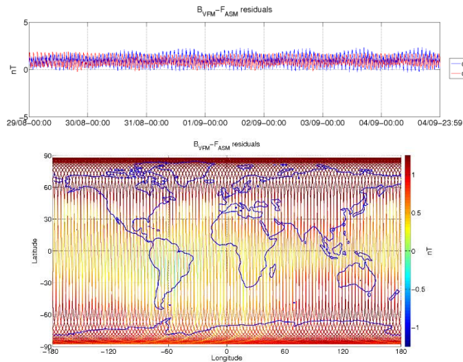
Figure 3-6: ASM-VFM residuals for S/C B, during monitoring period 29/08-04/09. In top figure are plotted: difference between |B_{VFM}| and F_{ASM} (without dB_{Sun} correction) (blue colour), and the residuals with dB_{Sun} corrections (red colour). In bottom figure residuals are presented on the world map.
