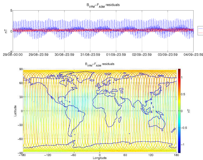
Figure 3-5: ASM-VFM residuals for S/C A, during monitoring period 29/08-04/09. In top figure are plotted: difference between |B_{VFM}| and F_{ASM} (without dB_Sun correction) (blue colour), and the residuals with dB_Sun corrections (red colour). In bottom figure residuals are presented on the world map.
