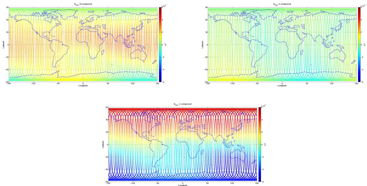
Figure 3-9: S/C C, world map plots of the geomagnetic field and components measured during monitoring period 29/08-04/09. From top to bottom: B_{NEC} components (North, East, and Centre) of magnetic field from VFM measurement.
