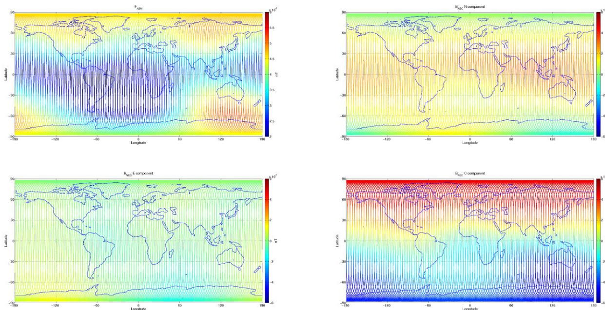
Figure 3-8: S/C B, world map plots of the geomagnetic field and components measured during monitoring period 29/08-04/09. From top to bottom: F-magnetic field from ASM measurement, B_{NEC} components (North, East, and Centre) of magnetic field from VFM measurement.
