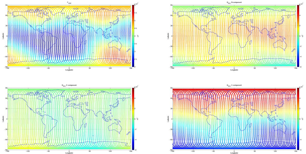
Figure 3-7: S/C A, world map plots of the geomagnetic field and components measured during monitoring period 29/08-04/09. From top to bottom: F-magnetic field from ASM measurement, B_{NEC} components (North, East, and Centre) of magnetic field from VFM measurement.
