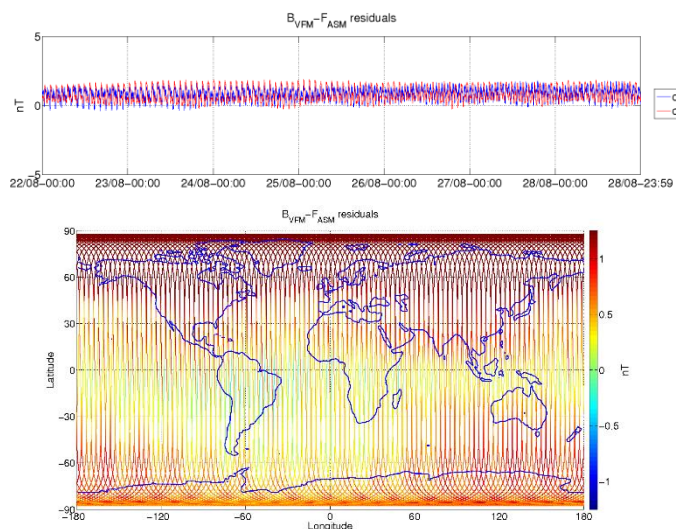
Figure 3-6: ASM-VFM residuals for S/C B, during monitoring period 22/08-28/08. In top figure are plotted: difference between |B_{VFM}| and F_{ASM} (without dB_Sun correction) (blue colour), and the residuals with dB_Sun corrections (red colour). In bottom figure residuals are presented on the world map.
