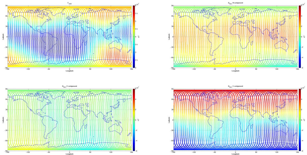
Figure 3-7: S/C A, world map plots of the geomagnetic field and components measured during monitoring period 22/08-28/08. From top to bottom: F-magnetic field from ASM measurement, B_{NEC} components (North, East, and Centre) of magnetic field from VFM measurement.
