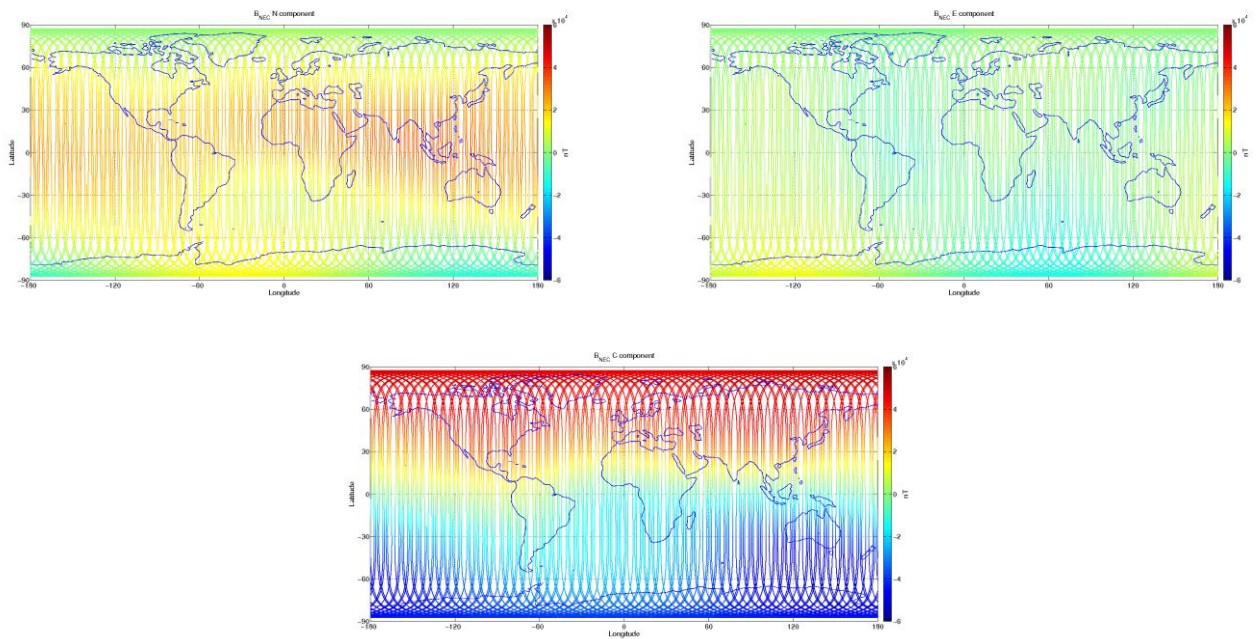
Figure 3-9: S/C C, world map plots of the geomagnetic field and components measured during monitoring period 22/08-28/08. From top to bottom: B_{NEC} components (North, East, and Centre) of magnetic field from VFM measurement.
