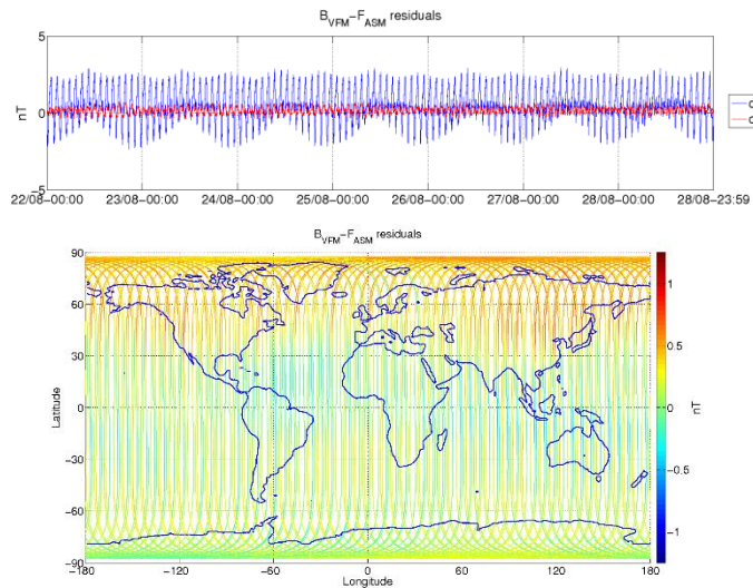
Figure 3-5: ASM-VFM residuals for S/C A, during monitoring period 22/08-28/08. In top figure are plotted: difference between |B_{VFM}| and F_{ASM} (without dB_Sun correction) (blue colour), and the residuals with dB_Sun corrections (red colour). In bottom figure residuals are presented on the world map.
