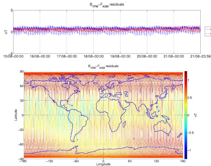
Figure 3-6: ASM-VFM residuals for S/C B, during monitoring period 15/08-21/08. In top figure are plotted: difference between |B_{VFM}| and F_{ASM} (without dB_{Sun} correction) (blue colour), and the residuals with dB_{Sun} corrections (red colour). In bottom figure residuals are presented on the world map.
