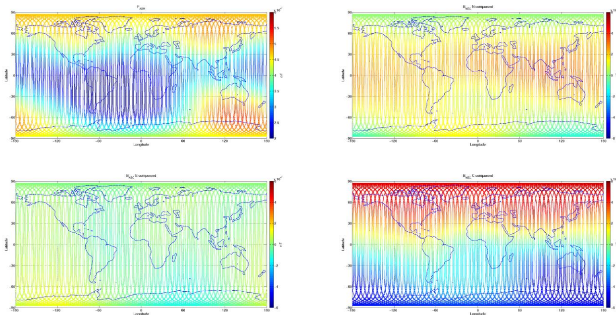
Figure 3-7: S/C A, world map plots of the geomagnetic field and components measured during monitoring period 15/08-21/08. From top to bottom: F-magnetic field from ASM measurement, B_{NEC} components (North, East, and Centre) of magnetic field from VFM measurement.
