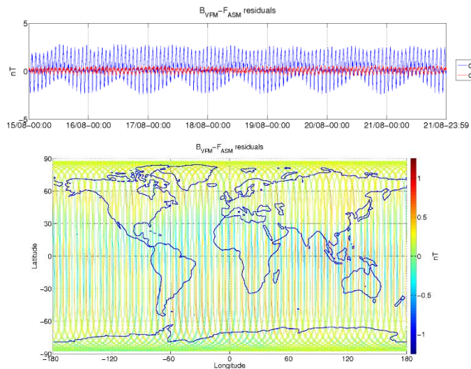
Figure 3-5: ASM-VFM residuals for S/C A, during monitoring period 15/08-21/08. In top figure are plotted: difference between |B_{VFM}| and F_{ASM} (without dB_{Sun} correction) (blue colour), and the residuals with dB_{Sun} corrections (red colour). In bottom figure residuals are presented on the world map.
