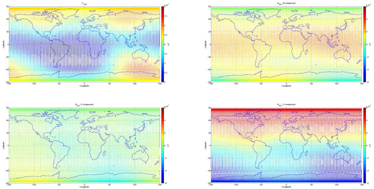
Figure 3-8: S/C B, world map plots of the geomagnetic field and components measured during monitoring period 15/08-21/08. From top to bottom: F-magnetic field from ASM measurement, B_{NEC} components (North, East, and Centre) of magnetic field from VFM measurement.
