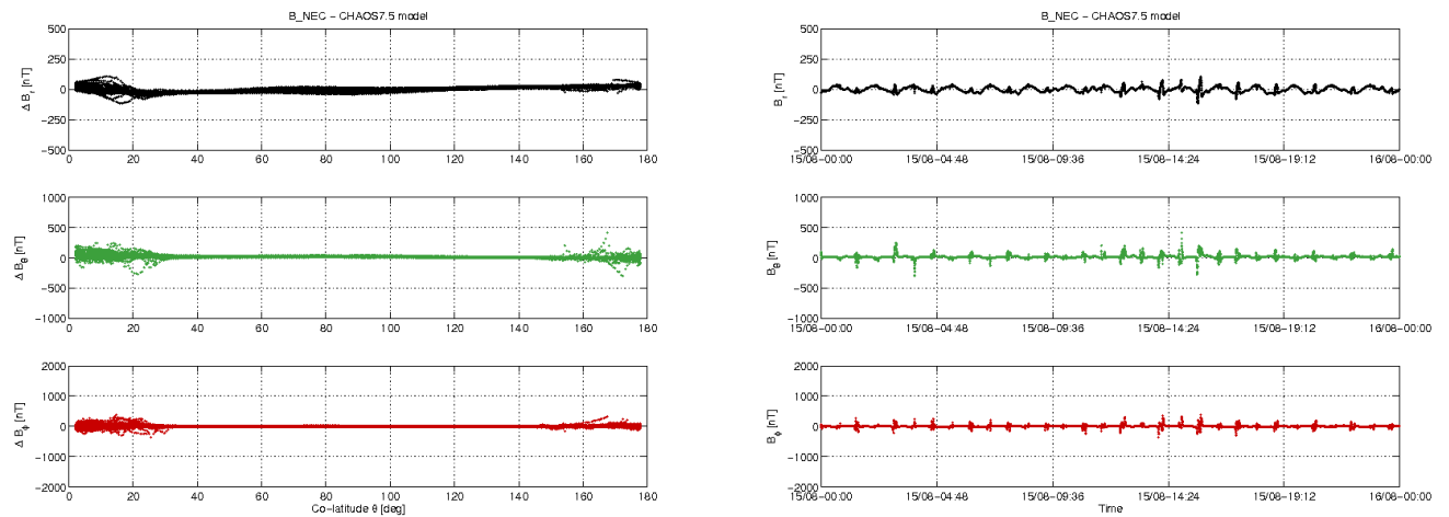
Figure 3-11: S/C B day 15.08: time series of B_{NEC} - B_{Chaos} residuals (right) and B_{NEC} - B_{Chaos} vs colatitude (left).
