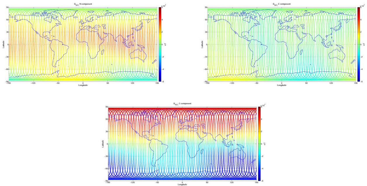
Figure 3-9: S/C C, world map plots of the geomagnetic field and components measured during monitoring period 15/08-21/08. From top to bottom: B_{NEC} components (North, East, and Centre) of magnetic field from VFM measurement.
