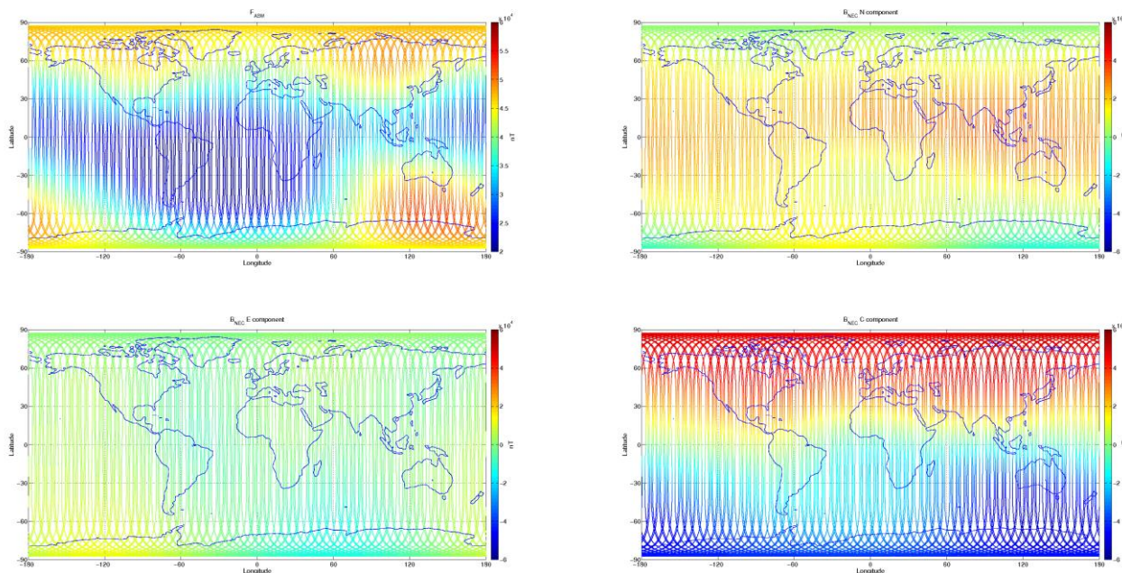
Figure 3-7: S/C A, world map plots of the geomagnetic field and components measured during monitoring period 08/08-14/08. From top to bottom: F-magnetic field from ASM measurement, B_{NEC} components (North, East, and Centre) of magnetic field from VFM measurement.
