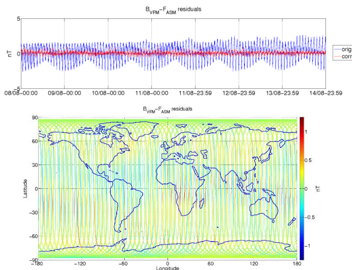
Figure 3-5: ASM-VFM residuals for S/C A, during monitoring period 08/08-14/08. In top figure are plotted: difference between |B_{VFM}| and F_{ASM} (without dB_{Sun} correction) (blue colour), and the residuals with dB_{Sun} corrections (red colour). In bottom figure residuals are presented on the world map.
