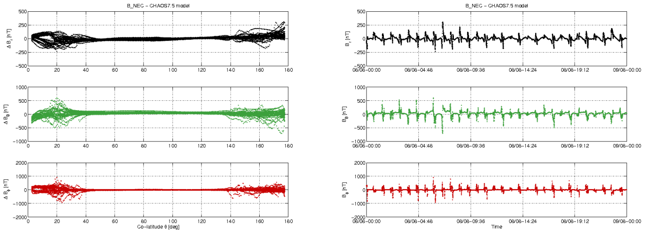
Figure 3-12: S/C C day 08.08: time series of B_{NEC} - B_{Chaos} residuals (right) and B_{NEC} - B_{Chaos} vs colatitude (left)
