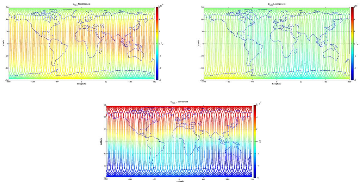
Figure 3-9: S/C C, world map plots of the geomagnetic field and components measured during monitoring period 08/08-14/08. From top to bottom: B_{NEC} components (North, East, and Centre) of magnetic field from VFM measurement.
