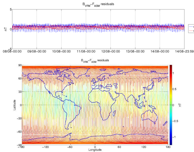
Figure 3-6: ASM-VFM residuals for S/C B, during monitoring period 08/08-14/08. In top figure are plotted: difference between |B_{VFM}| and F_{ASM} (without dB_{Sun} correction) (blue colour), and the residuals with dB_{Sun} corrections (red colour). In bottom figure residuals are presented on the world map.
