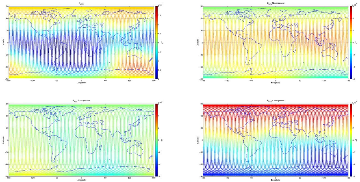
Figure 3-8: S/C B, world map plots of the geomagnetic field and components measured during monitoring period 08/08-14/08. From top to bottom: F-magnetic field from ASM measurement, B_{NEC} components (North, East, and Centre) of magnetic field from VFM measurement.
