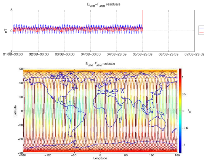
Figure 3-6: ASM-VFM residuals for S/C B, during monitoring period 01/08-07/08. In top figure are plotted: difference between |B_{VFM}| and F_{ASM} (without dB_{Sun} correction) (blue colour), and the residuals with dB_{Sun} corrections (red colour). In bottom figure residuals are presented on the world map.
