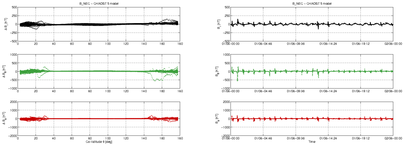
Figure 3-10: S/C A day 01.08: time series of B_{NEC} - B_{Chaos} residuals (right) and B_{NEC} - B_{Chaos} vs colatitude (left).
