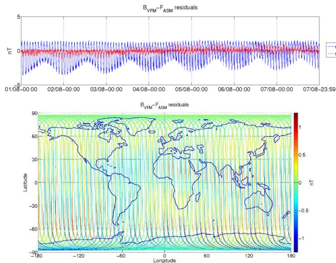
Figure 3-5: ASM-VFM residuals for S/C A, during monitoring period 01/08-07/08. In top figure are plotted: difference between |B_{VFM}| and F_{ASM} (without dB_{Sun} correction) (blue colour), and the residuals with dB_{Sun} corrections (red colour). In bottom figure residuals are presented on the world map.
