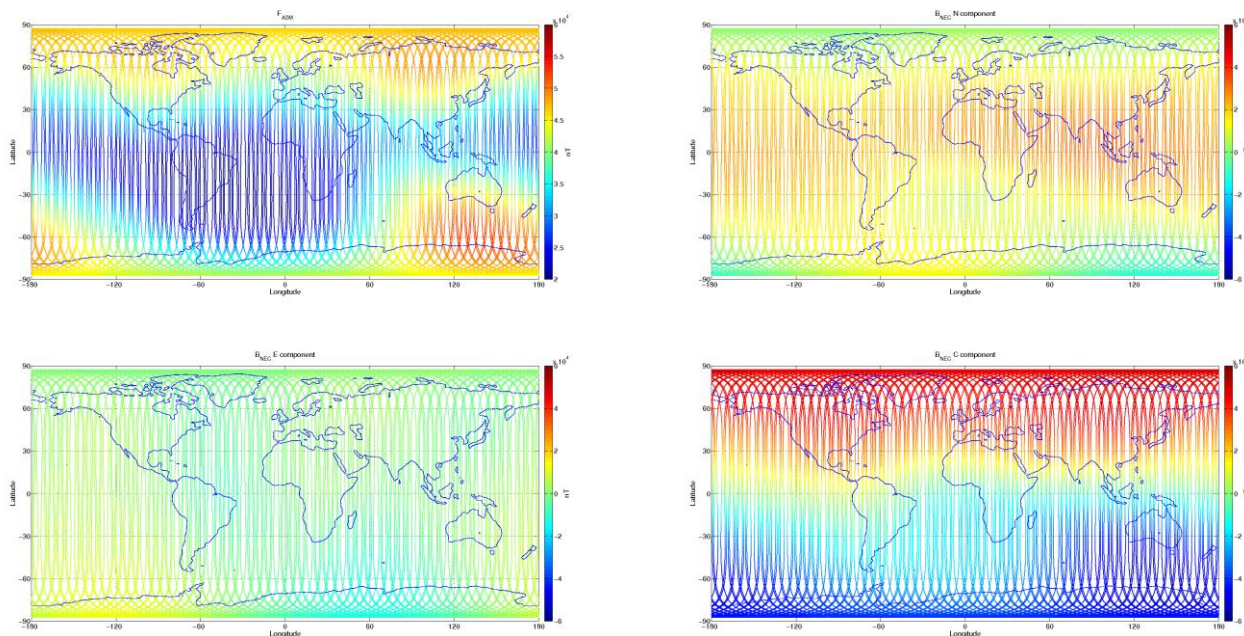
Figure 3-7: S/C A, world map plots of the geomagnetic field and components measured during monitoring period 01/08-07/08. From top to bottom: F-magnetic field from ASM measurement, B_{NEC} components (North, East, and Centre) of magnetic field from VFM measurement.
