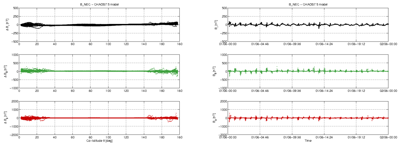
Figure 3-11: S/C B day 01.08: time series of B_{NEC} - B_{Chaos} residuals (right) and B_{NEC} - B_{Chaos} vs colatitude (left).
