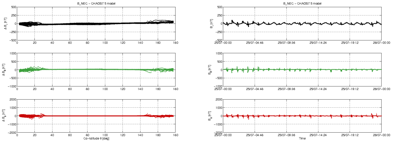
Figure 3-12: S/C C day 25/07: time series of B_{NEC} - B_{Chaos} residuals (right) and B_{NEC} - B_{Chaos} vs colatitude (left)
