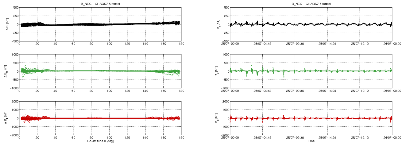
Figure 3-11: S/C B day 25/07: time series of B_{NEC} - B_{Chaos} residuals (right) and B_{NEC} - B_{Chaos} vs colatitude (left).
