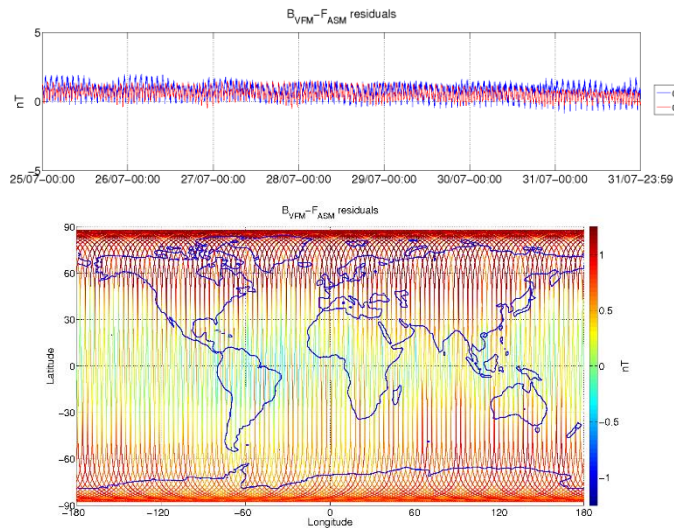
Figure 3-6: ASM-VFM residuals for S/C B, during monitoring period 25/07-31/07. In top figure are plotted: difference between |B_{VFM}| and F_{ASM} (without dB_{Sun} correction) (blue colour), and the residuals with dB_{Sun} corrections (red colour). In bottom figure residuals are presented on the world map.
