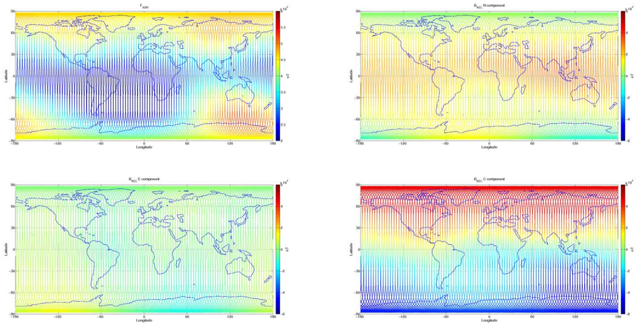
Figure 3-8: S/C B, world map plots of the geomagnetic field and components measured during monitoring period 25/07-31/07. From top to bottom: F-magnetic field from ASM measurement, B_{NEC} components (North, East, and Centre) of magnetic field from VFM measurement.
