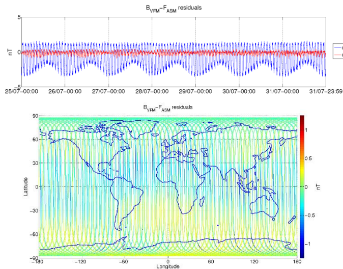
Figure 3-5: ASM-VFM residuals for S/C A, during monitoring period 25/07-31/07. In top figure are plotted: difference between |B_{VFM}| and F_{ASM} (without dB_{Sun} correction) (blue colour), and the residuals with dB_{Sun} corrections (red colour). In bottom figure residuals are presented on the world map.
