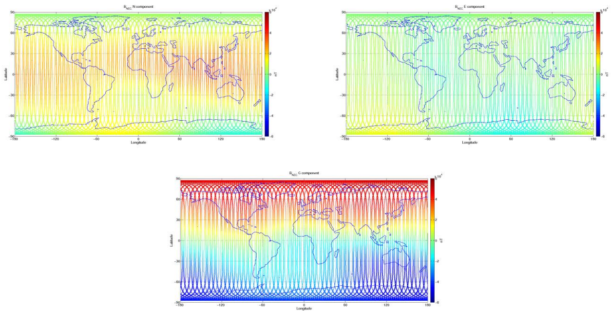
Figure 3-9: S/C C, world map plots of the geomagnetic field and components measured during monitoring period 25/07-31/07. From top to bottom: B_{NEC} components (North, East, and Centre) of magnetic field from VFM measurement.
