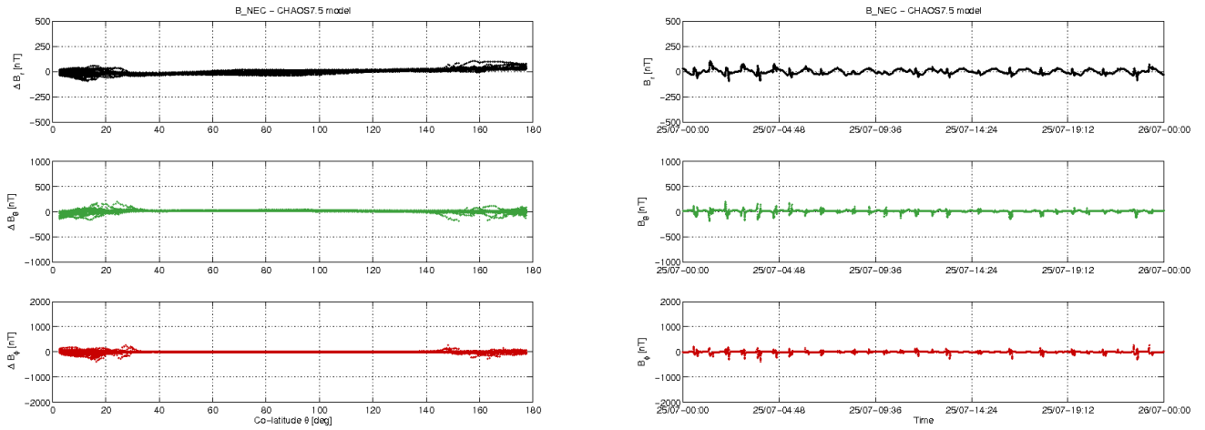
Figure 3-10: S/C A day 25/07: time series of B_{NEC} - B_{Chaos} residuals (right) and B_{NEC} - B_{Chaos} vs colatitude (left).
