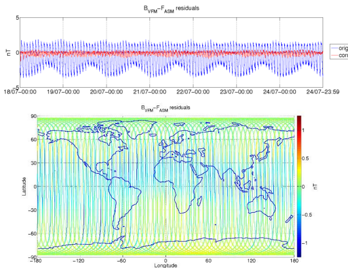
Figure 3-5: ASM-VFM residuals for S/C A, during monitoring period 18/07-24/07. In top figure are plotted: difference between |B_{VFM}| and F_{ASM} (without dB_{Sun} correction) (blue colour), and the residuals with dB_{Sun} corrections (red colour). In bottom figure residuals are presented on the world map.
