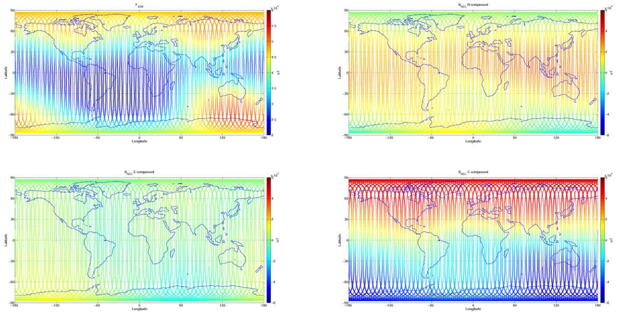
Figure 3-7: S/C A, world map plots of the geomagnetic field and components measured during monitoring period 18/07-24/07. From top to bottom: F_{ASM} magnetic field from ASM measurement, B_{NEC} components (North, East, and Centre) of magnetic field from VFM measurement.
