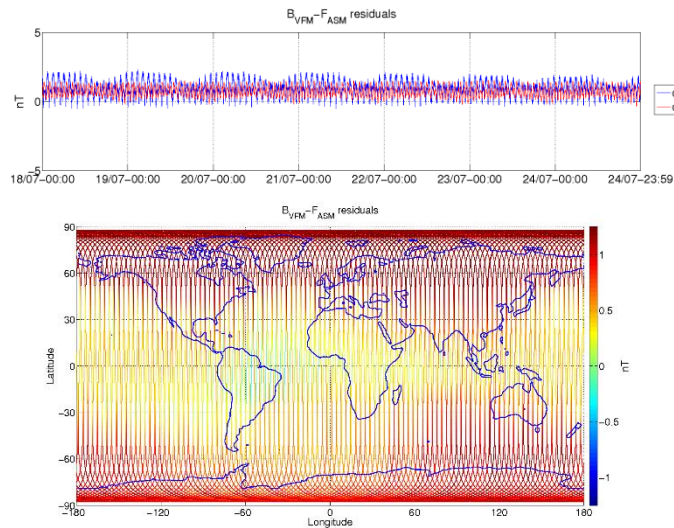
Figure 3-6: ASM-VFM residuals for S/C B, during monitoring period 18/07-24/07. In top figure are plotted: difference between |B_{VFM}| and F_{ASM} (without dB_{Sun} correction) (blue colour), and the residuals with dB_{Sun} corrections (red colour). In bottom figure residuals are presented on the world map.
