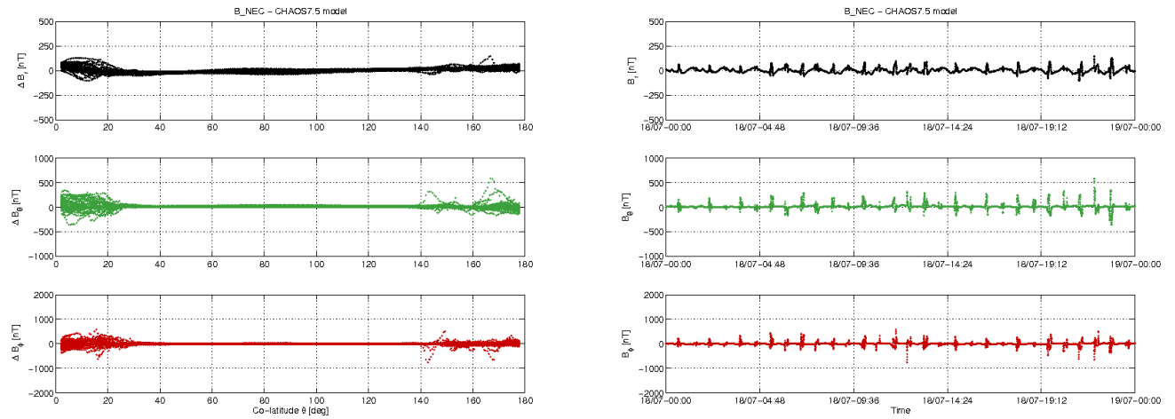
Figure 3-11: S/C B day 18/07: time series of B_{NEC} - B_{Chaos} residuals (right) and B_{NEC} - B_{Chaos} vs colatitude (left).
