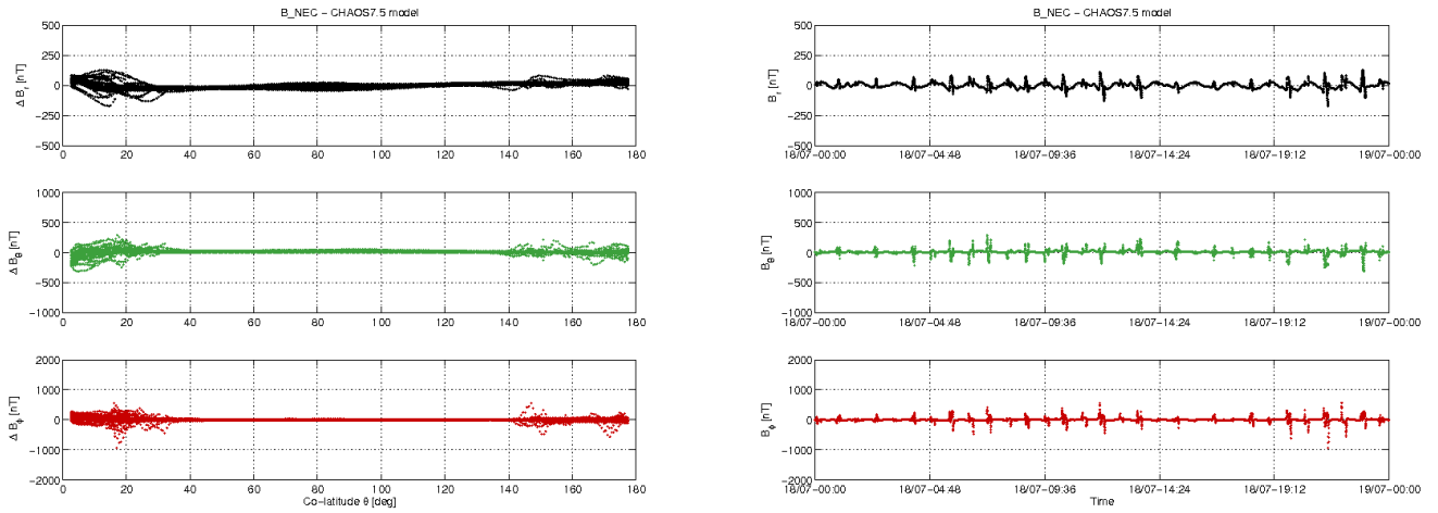
Figure 3-10: S/C A day 18/07: time series of B_{NEC} - B_{Chaos} residuals (right) and B_{NEC} - B_{Chaos} vs colatitude (left).
