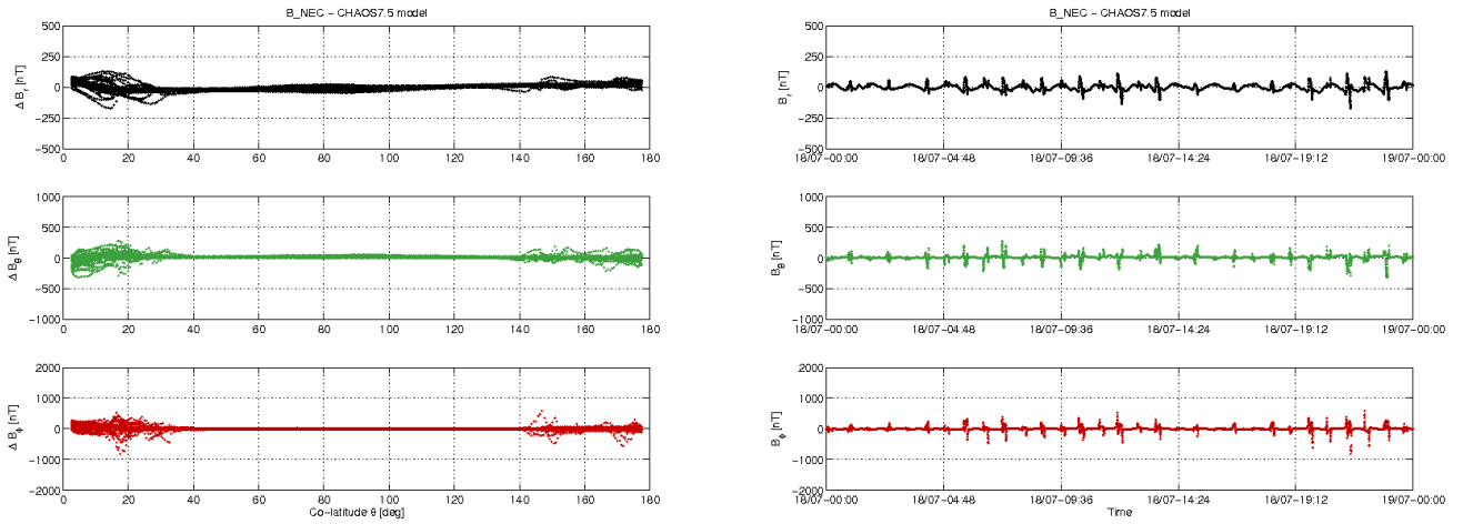
Figure 3-12: S/C C day 18/07: time series of B_{NEC} - B_{Chaos} residuals (right) and B_{NEC} - B_{Chaos} vs colatitude (left)
