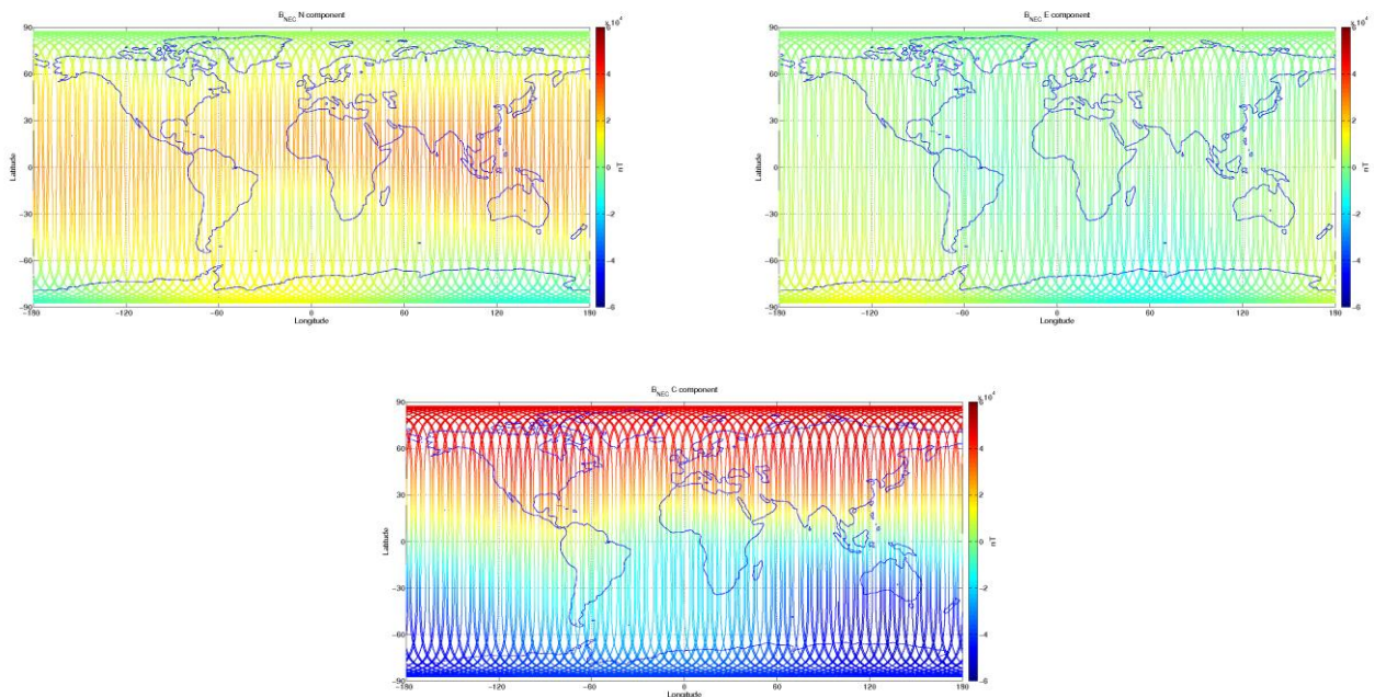
Figure 3-9: S/C C, world map plots of the geomagnetic field and components measured during monitoring period 18/07-24/07. From top to bottom: B_{NEC} components (North, East, and Centre) of magnetic field from VFM measurement.
