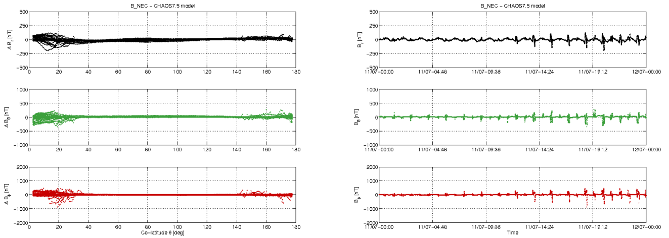
Figure 3-10: S/C A day 11/07: time series of B_{NEC} - B_{Chaos} residuals (right) and B_{NEC} - B_{Chaos} vs colatitude (left).
