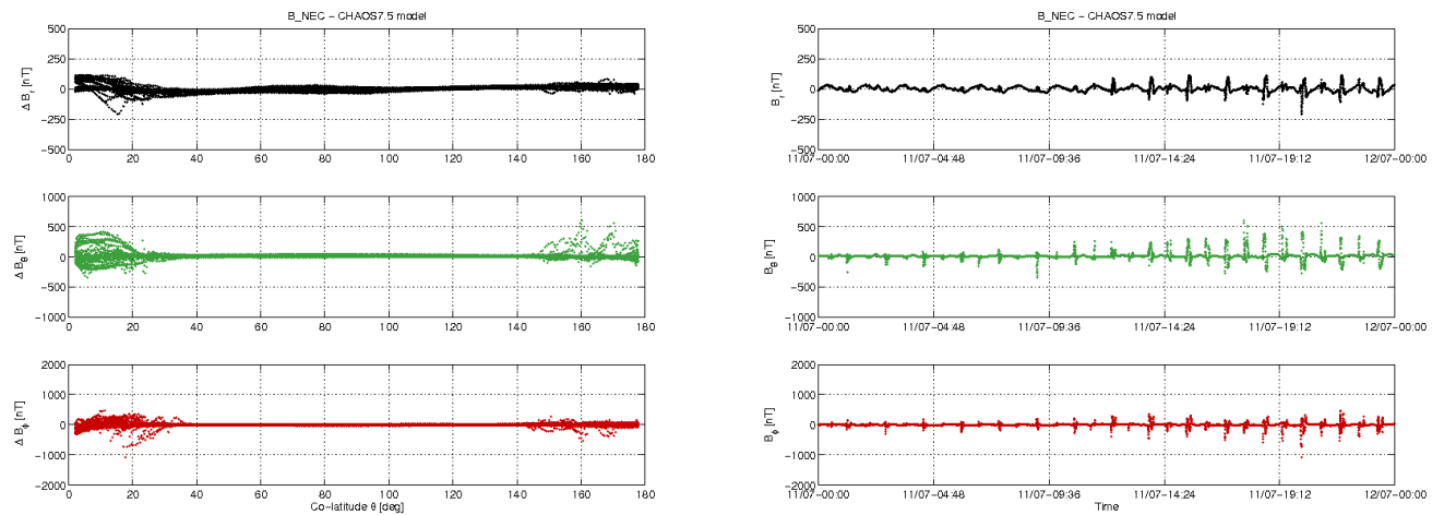
Figure 3-11: S/C B day 11/07: time series of B_{NEC} - B_{Chaos} residuals (right) and B_{NEC} - B_{Chaos} vs colatitude (left).
