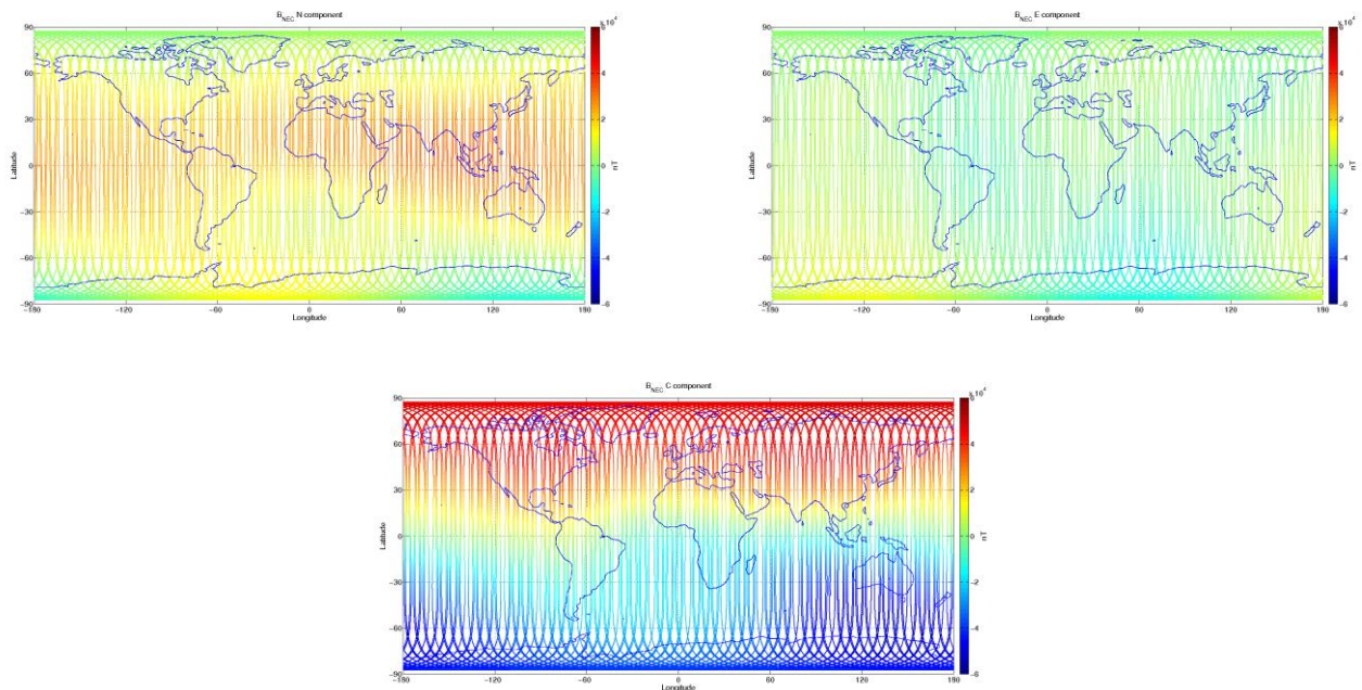
Figure 3-9: S/C C, world map plots of the geomagnetic field and components measured during monitoring period 11/07-17/07. From top to bottom: B_{NEC} components (North, East, and Centre) of magnetic field from VFM measurement.
