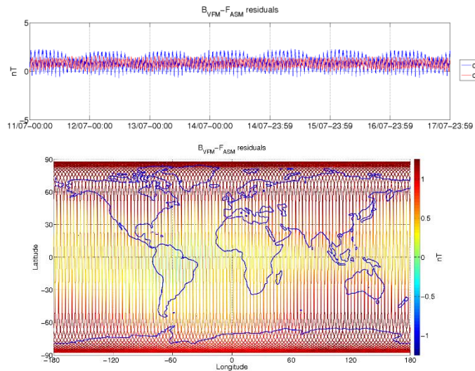
Figure 3-6: ASM-VFM residuals for S/C B, during monitoring period 11/07-17/07. In top figure are plotted: difference between |B_{VFM}| and F_{ASM} (without dB_{Sun} correction) (blue colour), and the residuals with dB_{Sun} corrections (red colour). In bottom figure residuals are presented on the world map.
