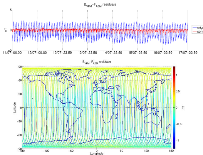
Figure 3-5: ASM-VFM residuals for S/C A, during monitoring period 11/07-17/07. In top figure are plotted: difference between |B_{VFM}| and F_{ASM} (without dB_{Sun} correction) (blue colour), and the residuals with dB_{Sun} corrections (red colour). In bottom figure residuals are presented on the world map.
