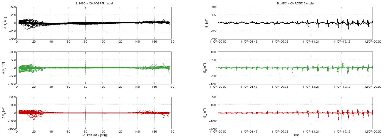
Figure 3-12: S/C C day 11/07: time series of B_{NEG} - B_{Chaos} residuals (right) and B_{NEG} - B_{Chaos} vs colatitude (left)
