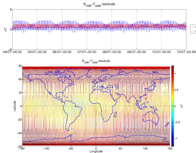
Figure 3-6: ASM-VFM residuals for S/C B, during monitoring period 04/07-10/07. In top figure are plotted: difference between |B_{VFM}| and F_{ASM} (without dB_{Sun} correction) (blue colour), and the residuals with dB_{Sun} corrections (red colour). In bottom figure residuals are presented on the world map.
