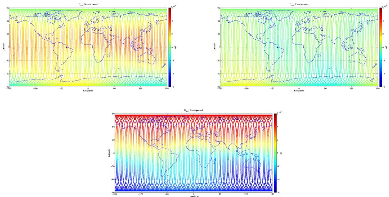
Figure 3-9: S/C C, world map plots of the geomagnetic field and components measured during monitoring period 04/07-10/07. From top to bottom: B_{NEC} components (North, East, and Centre) of magnetic field from VFM measurement.
