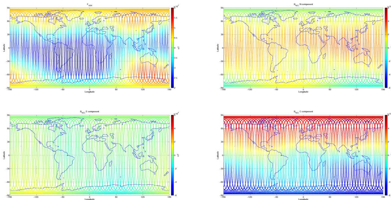
Figure 3-7: S/C A, world map plots of the geomagnetic field and components measured during monitoring period 04/07-10/07. From top to bottom: F-magnetic field from ASM measurement, B_{NEC} components (North, East, and Centre) of magnetic field from VFM measurement.
