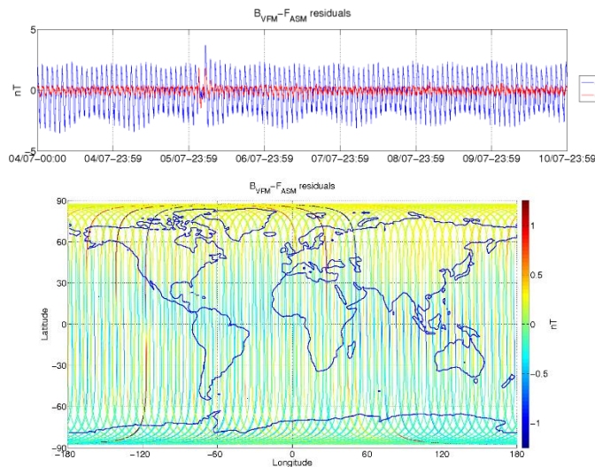
Figure 3-5: ASM-VFM residuals for S/C A, during monitoring period 04/07-10/07. In top figure are plotted: difference between |B_{VFM}| and F_{ASM} (without dB_{Sun} correction) (blue colour), and the residuals with dB_{Sun} corrections (red colour). In bottom figure residuals are presented on the world map.
