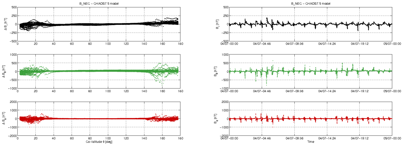
Figure 3-12: S/C C day 04/07: time series of B_{NEC} - B_{Chaos} residuals (right) and B_{NEC} - B_{Chaos} vs colatitude (left)
