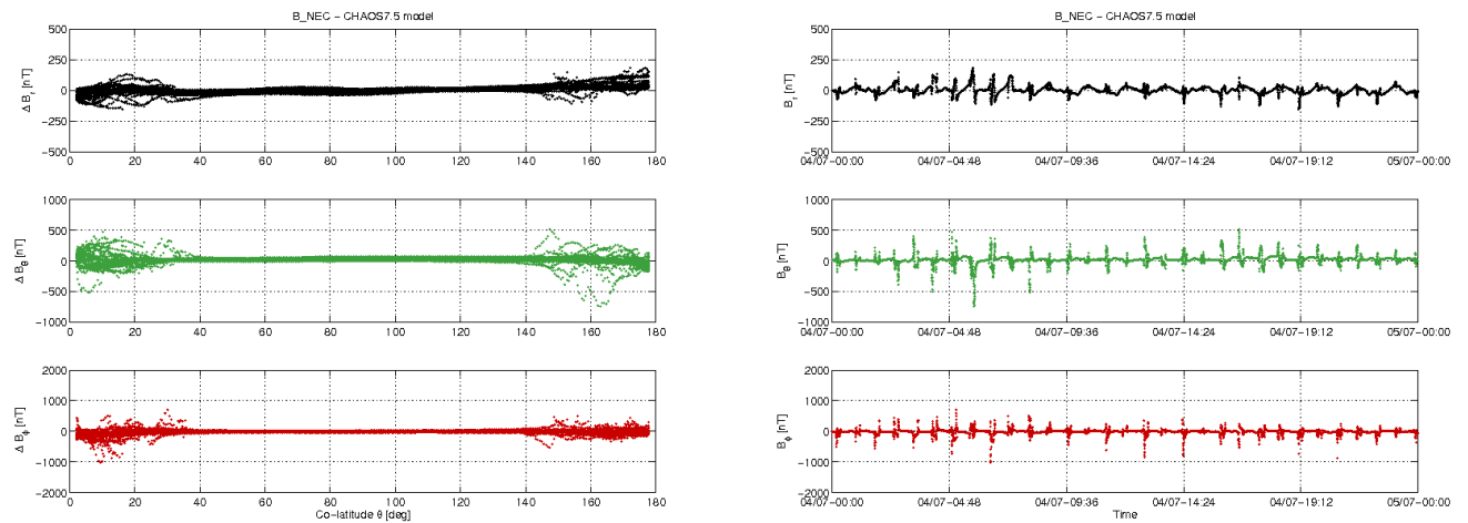
Figure 3-11: S/C B day 04/07: time series of B_{NEC} - B_{Chaos} residuals (right) and B_{NEC} - B_{Chaos} vs colatitude (left).
