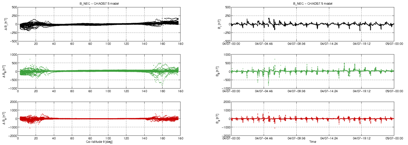
Figure 3-10: S/C A day 04/07: time series of B_{NEC} - B_{Chaos} residuals (right) and B_{NEC} - B_{Chaos} vs colatitude (left).
