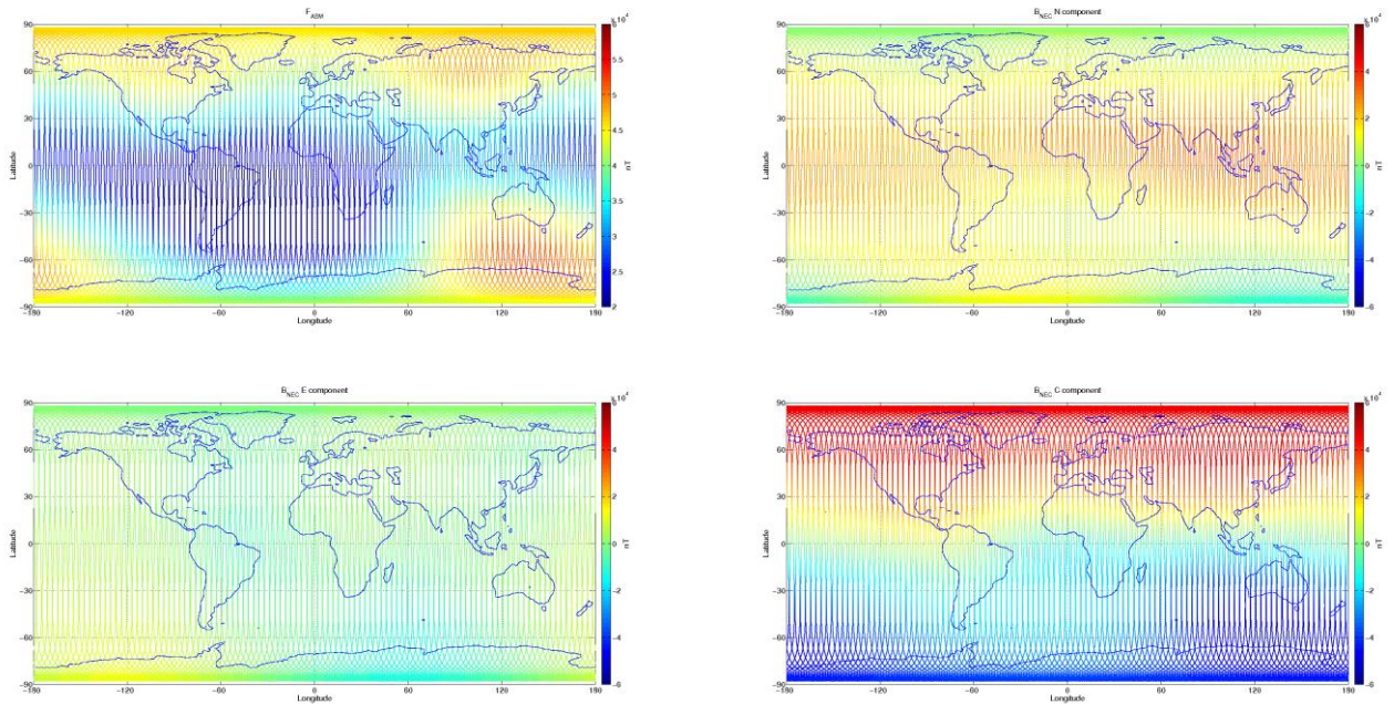
Figure 3-8: S/C B, world map plots of the geomagnetic field and components measured during monitoring period 04/07-10/07. From top to bottom: F-magnetic field from ASM measurement, B_{NEC} components (North, East, and Centre) of magnetic field from VFM measurement.
