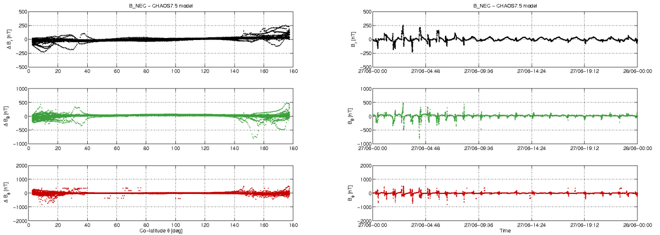
Figure 3-12: S/C C day 27/06: time series of B_{NEC} - B_{Chaos} residuals (right) and B_{NEC} - B_{Chaos} vs colatitude (left)
