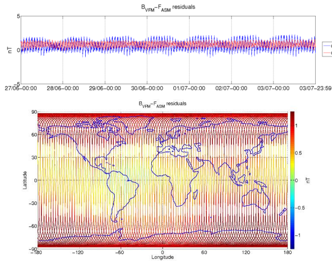
Figure 3-6: ASM-VFM residuals for S/C B, during monitoring period 27/06-03/07. In top figure are plotted: difference between |B_{VFM}| and F_{ASM} (without dB_{Sun} correction) (blue colour), and the residuals with dB_{Sun} corrections (red colour). In bottom figure residuals are presented on the world map.
