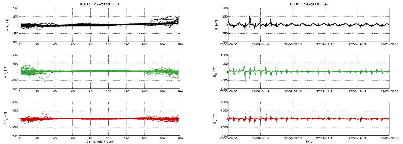
Figure 3-11: S/C B day 27/06: time series of B_{NEC} - B_{Chaos} residuals (right) and B_{NEC} - B_{Chaos} vs colatitude (left).
