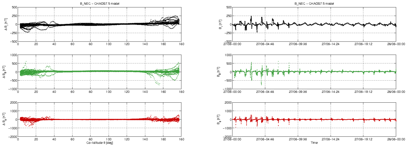
Figure 3-10: S/C A day 27/06: time series of B_{NEC} - B_{Chaos} residuals (right) and B_{NEC} - B_{Chaos} vs colatitude (left).
