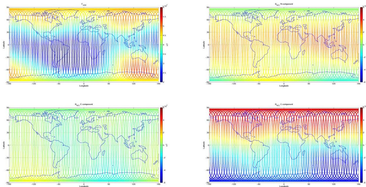
Figure 3-7: S/C A, world map plots of the geomagnetic field and components measured during monitoring period 27/06-03/07. From top to bottom: F-magnetic field from ASM measurement, B_{NEC} components (North, East, and Centre) of magnetic field from VFM measurement.
