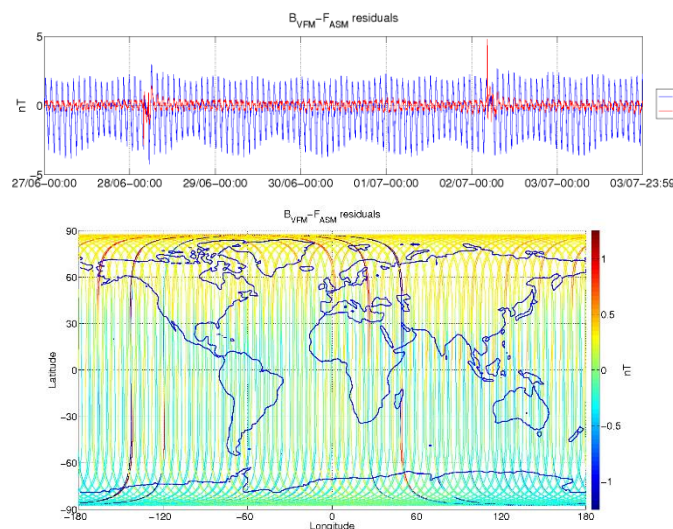
Figure 3-5: ASM-VFM residuals for S/C A, during monitoring period 27/06-03/07. In top figure are plotted: difference between |B_{VFM}| and F_{ASM} (without dB_Sun correction) (blue colour), and the residuals with dB_Sun corrections (red colour). In bottom figure residuals are presented on the world map.
