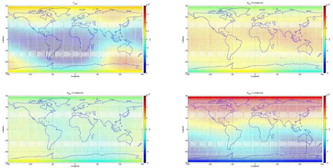
Figure 3-8: S/C B, world map plots of the geomagnetic field and components measured during monitoring period 27/06-03/07. From top to bottom: F-magnetic field from ASM measurement, B_{NEC} components (North, East, and Centre) of magnetic field from VFM measurement.
