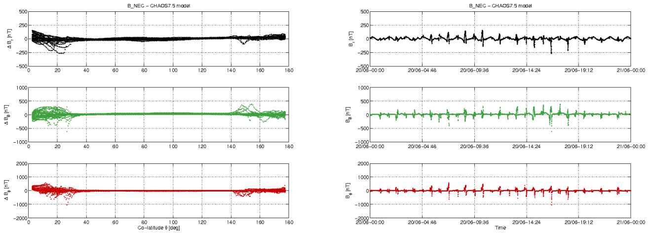
Figure 3-10: S/C A day 20/06: time series of B_{NEC} - B_{Chaos} residuals (right) and B_{NEC} - B_{Chaos} vs colatitude (left).
