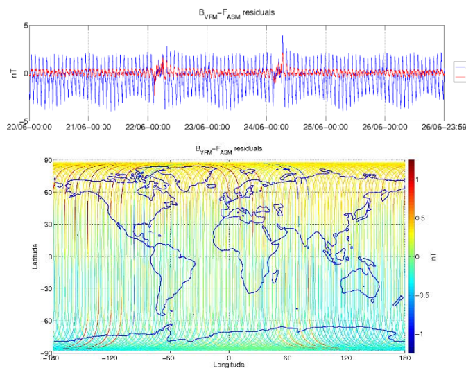
Figure 3-5: ASM-VFM residuals for S/C A, during monitoring period 20/06-26/06. In top figure are plotted: difference between |B_{VFM}| and F_{ASM} (without dB_Sun correction) (blue colour), and the residuals with dB_Sun corrections (red colour). In bottom figure residuals are presented on the world map.
