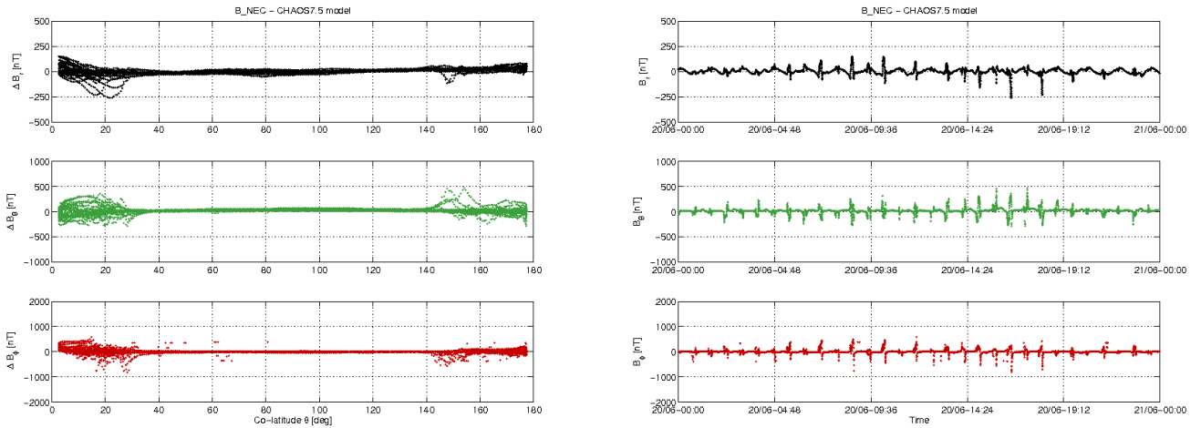
Figure 3-12: S/C C day 20/06: time series of B_{NEC} - B_{Chaos} residuals (right) and B_{NEC} - B_{Chaos} vs colatitude (left)
