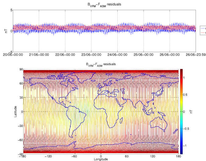
Figure 3-6: ASM-VFM residuals for S/C B, during monitoring period 20/06-26/06. In top figure are plotted: difference between |B_{VFM}| and F_{ASM} (without dB_{Sun} correction) (blue colour), and the residuals with dB_{Sun} corrections (red colour). In bottom figure residuals are presented on the world map.
