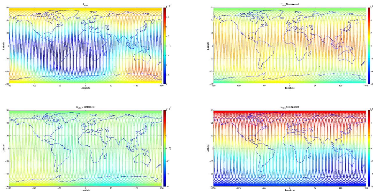
Figure 3-8: S/C B, world map plots of the geomagnetic field and components measured during monitoring period 20/06-26/06. From top to bottom: F-magnetic field from ASM measurement, B_{NEC} components (North, East, and Centre) of magnetic field from VFM measurement.
