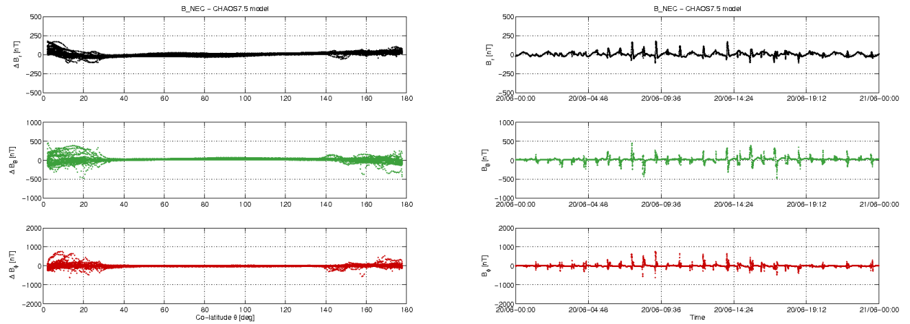
Figure 3-11: S/C B day 20/06: time series of B_{NEC} - B_{Chaos} residuals (right) and B_{NEC} - B_{Chaos} vs colatitude (left).
