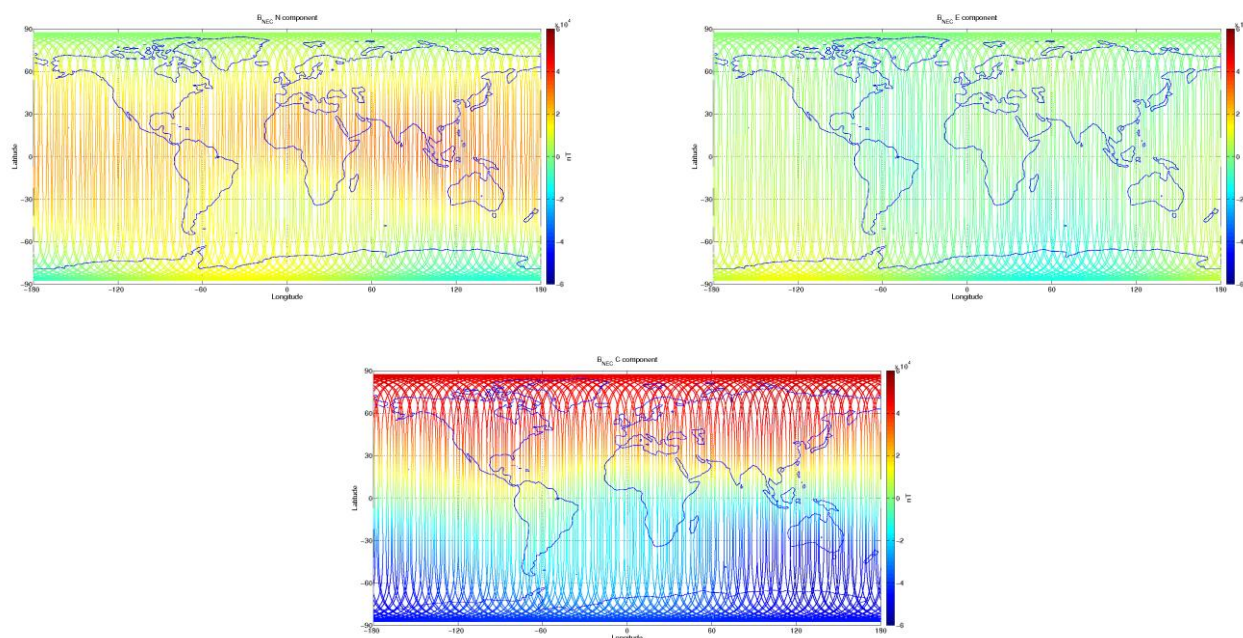
Figure 3-9: S/C C, world map plots of the geomagnetic field and components measured during monitoring period 20/06-26/06. From top to bottom: B_{NEC} components (North, East, and Centre) of magnetic field from VFM measurement.
