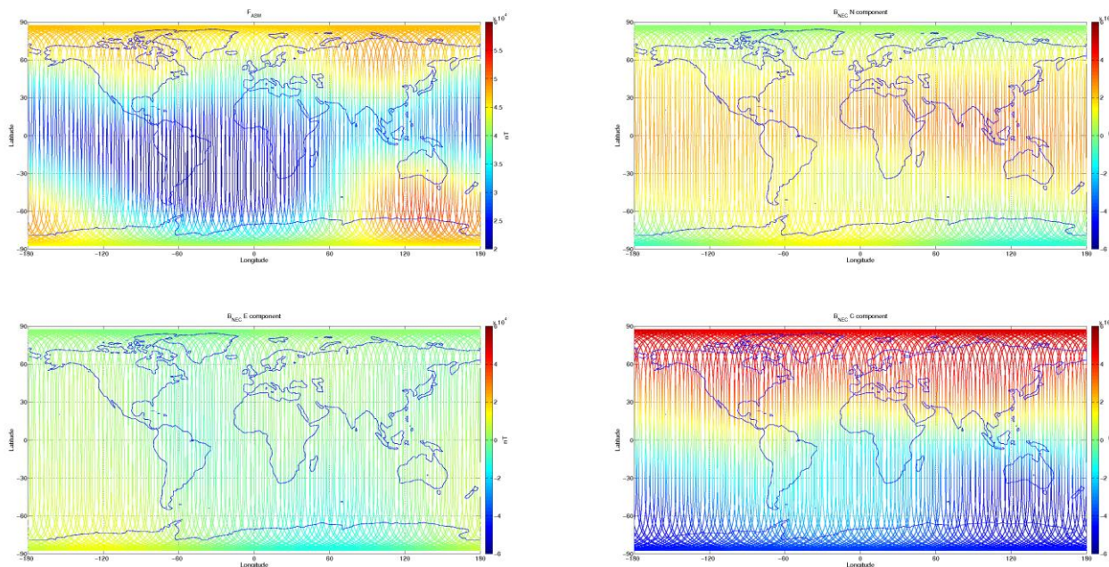
Figure 3-7: S/C A, world map plots of the geomagnetic field and components measured during monitoring period 20/06-26/06. From top to bottom: F-magnetic field from ASM measurement, B_{NEC} components (North, East, and Centre) of magnetic field from VFM measurement.
