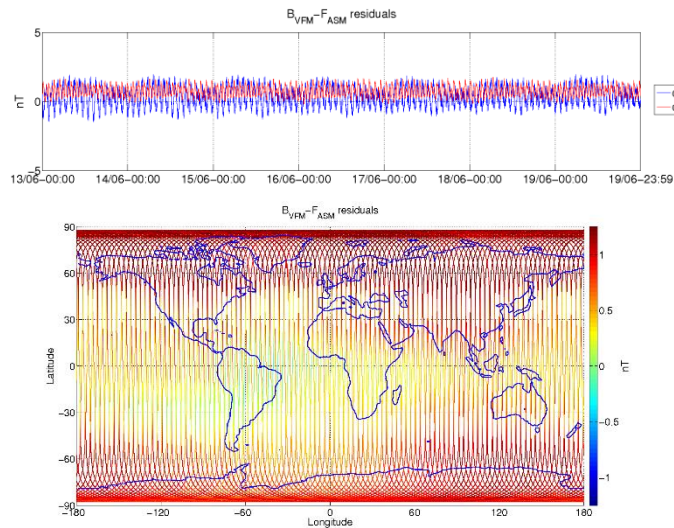
Figure 3-6: ASM-VFM residuals for S/C B, during monitoring period 13/06-19/06. In top figure are plotted: difference between |B_{VFM}| and F_{ASM} (without dB_{Sun} correction) (blue colour), and the residuals with dB_{Sun} corrections (red colour). In bottom figure residuals are presented on the world map.
