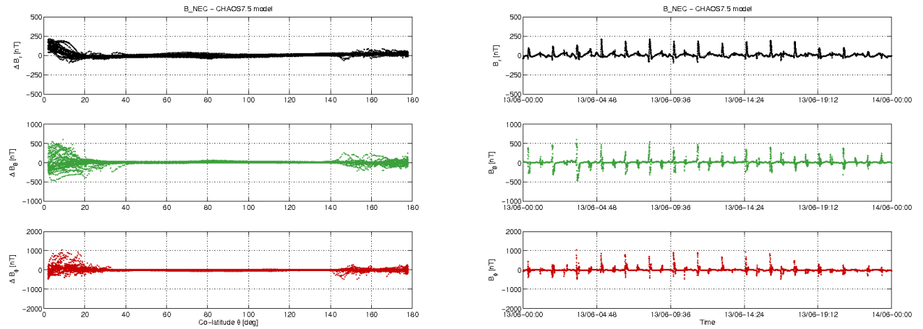
Figure 3-11: S/C B day 13/06: time series of B_{NEC} - B_{Chaos} residuals (right) and B_{NEC} - B_{Chaos} vs colatitude (left).
