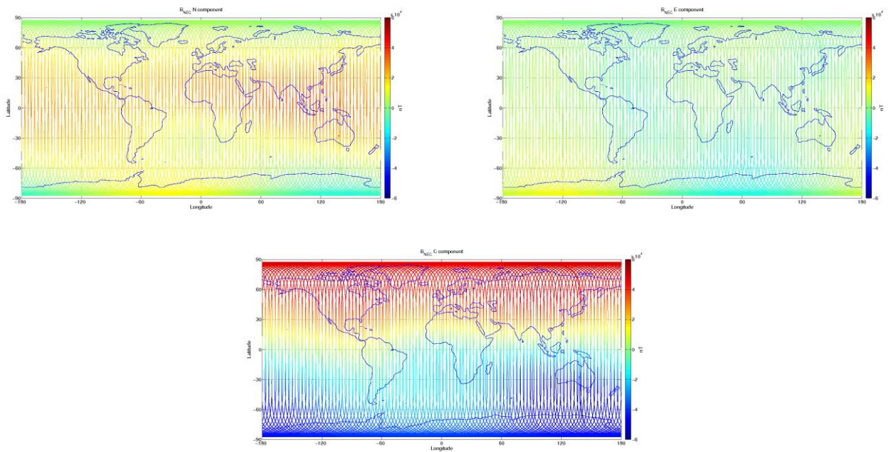
Figure 3-9: S/C C, world map plots of the geomagnetic field and components measured during monitoring period 13/06-19/06. From top to bottom: B_{NEC} components (North, East, and Centre) of magnetic field from VFM measurement.
