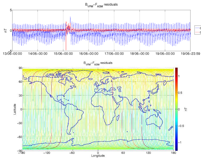
Figure 3-5: ASM-VFM residuals for S/C A, during monitoring period 13/06-19/06. In top figure are plotted: difference between |B_{VFM}| and F_{ASM} (without dB_{Sun} correction) (blue colour), and the residuals with dB_{Sun} corrections (red colour). In bottom figure residuals are presented on the world map.
