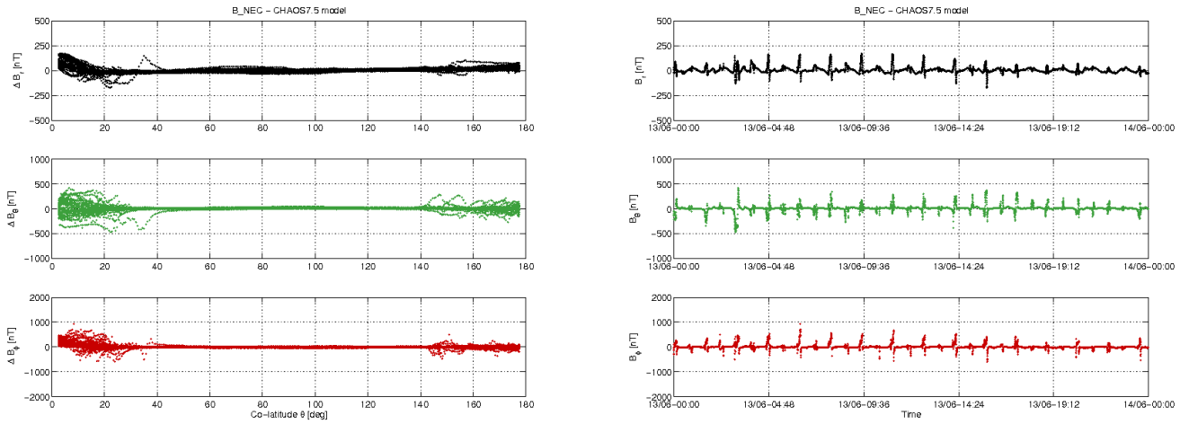
Figure 3-10: S/C A day 13/06: time series of B_{NEC} - B_{Chaos} residuals (right) and B_{NEC} - B_{Chaos} vs colatitude (left).
