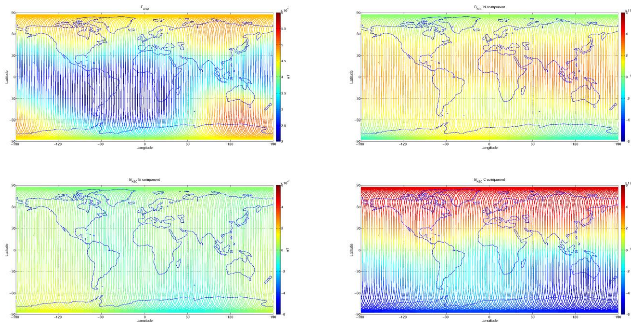
Figure 3-7: S/C A, world map plots of the geomagnetic field and components measured during monitoring period 13/06-19/06. From top to bottom: F-magnetic field from ASM measurement, B_{NEC} components (North, East, and Centre) of magnetic field from VFM measurement.
