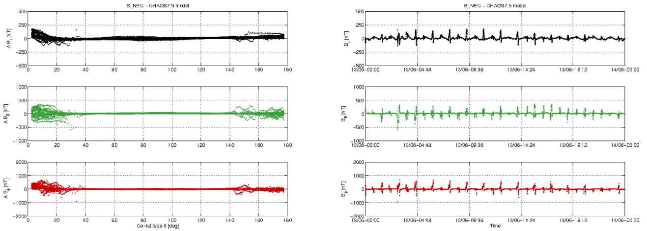
Figure 3-12: S/C C day 13/06: time series of B_{NEC} - B_{Chaos} residuals (right) and B_{NEC} - B_{Chaos} vs colatitude (left)
