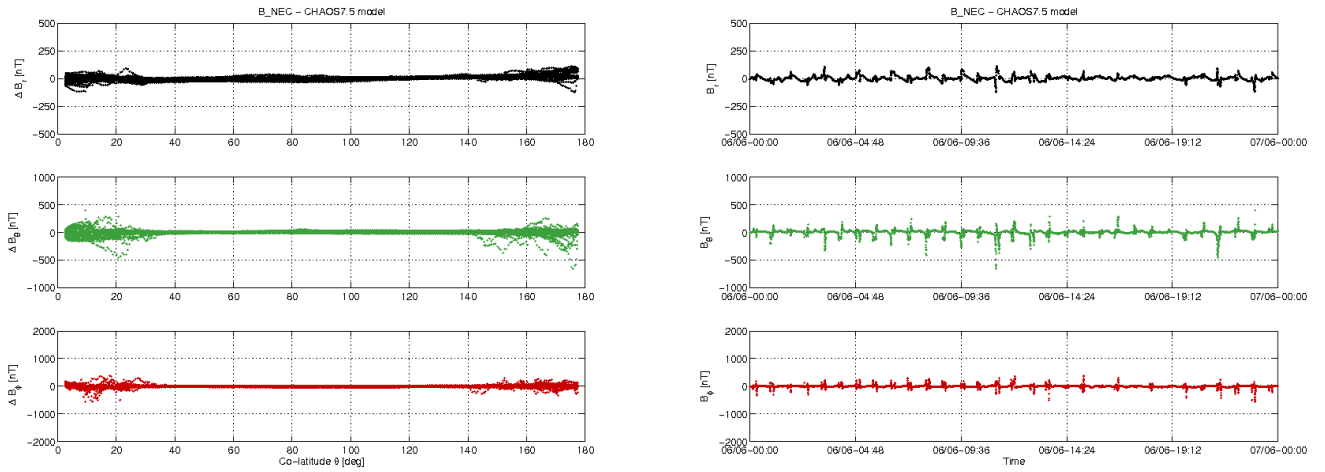
Figure 3-10: S/C A day 06/06: time series of B_{NEC} - B_{Chaos} residuals (right) and B_{NEC} - B_{Chaos} vs colatitude (left).
