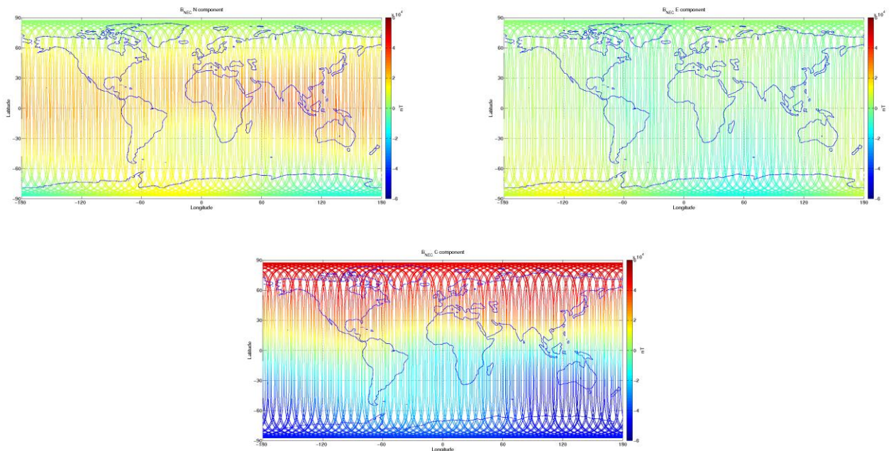
Figure 3-9: S/C C, world map plots of the geomagnetic field and components measured during monitoring period 06/06-12/06. From top to bottom: B_{NEC} components (North, East, and Centre) of magnetic field from VFM measurement.
