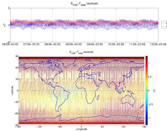
Figure 3-6: ASM-VFM residuals for S/C B, during monitoring period 06/06-12/06. In top figure are plotted: difference between |B_{VFM}| and F_{ASM} (without dB_{Sun} correction) (blue colour), and the residuals with dB_{Sun} corrections (red colour). In bottom figure residuals are presented on the world map.
