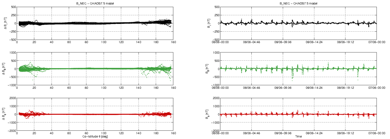
Figure 3-12: S/C C day 06/06: time series of B_{NEC} - B_{Chaos} residuals (right) and B_{NEC} - B_{Chaos} vs colatitude (left)
