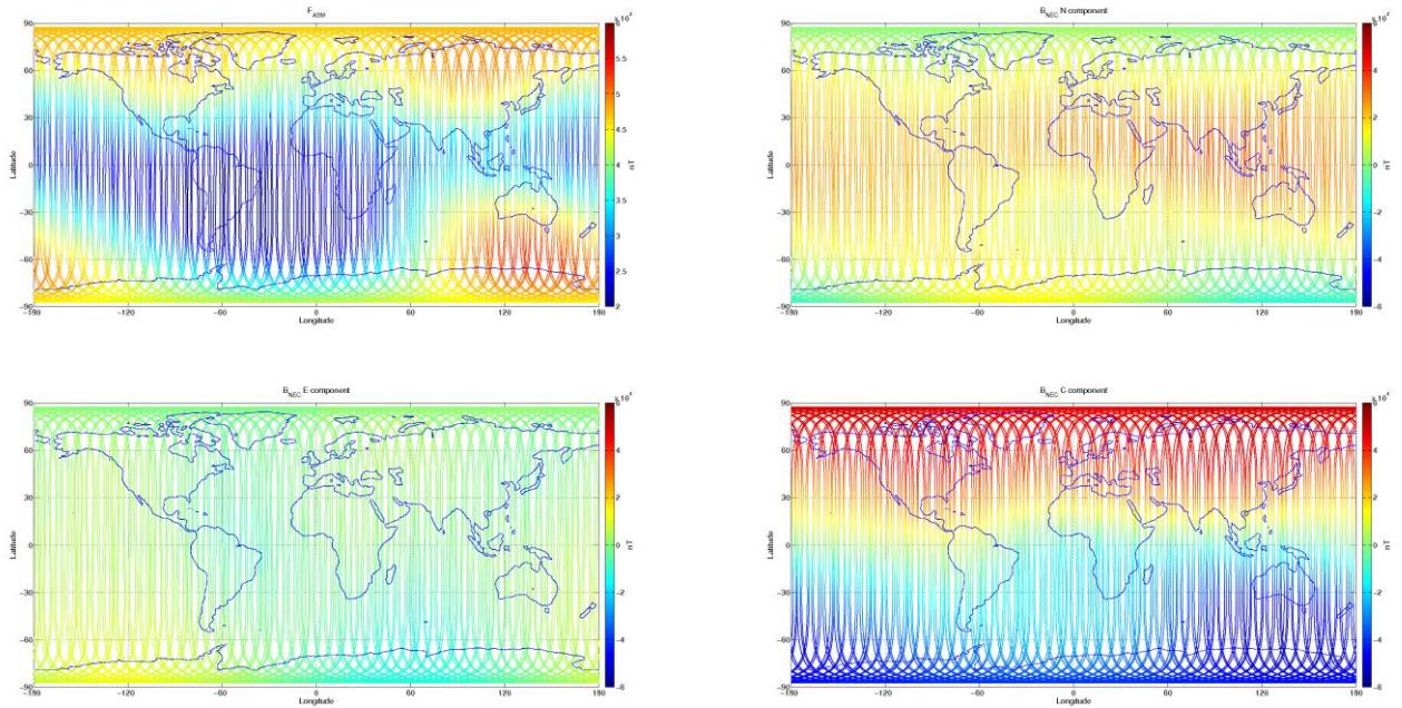
Figure 3-7: S/C A, world map plots of the geomagnetic field and components measured during monitoring period 06/06-12/06. From top to bottom: F_{ASM} magnetic field from ASM measurement, B_{NEC} components (North, East, and Centre) of magnetic field from VFM measurement.
