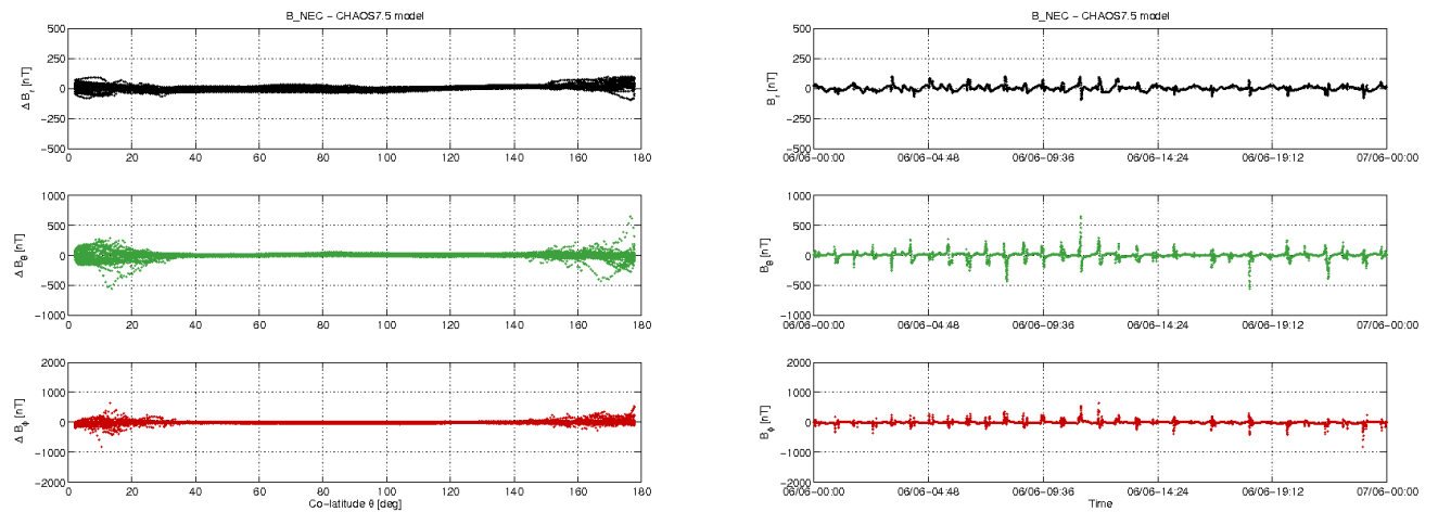
Figure 3-11: S/C B day 06/06: time series of B_{NEC} - B_{Chaos} residuals (right) and B_{NEC} - B_{Chaos} vs colatitude (left).
