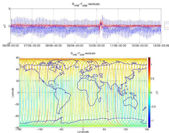
Figure 3-5: ASM-VFM residuals for S/C A, during monitoring period 06/06-12/06. In top figure are plotted: difference between |B_{VFM}| and F_{ASM} (without dB_Sun correction) (blue colour), and the residuals with dB_Sun corrections (red colour). In bottom figure residuals are presented on the world map.
